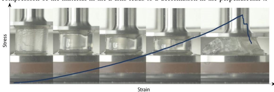
Figure 2.2 Compression test on hydrogel cylinders
