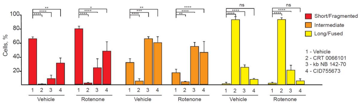
Figure 21. PKD activity is required for mitochondrial fission in mouse NIH 3T3 cells. (A) Confocal fluorescence microscopy images of NIH 3T3 cells treated with vehicle (DMSO) or one of three different PKD inhibitors (10 \mu M CRT 0066101, 10 \mu M kb-NB 142-70 or 30 \mu M CID 755673) in combination with vehicle or 1 \mu M Rotenone. Mitochondria were stained with MitoTracker Red (pseudocolored in white) and nuclei were counterstained with DAPI. Scale bar: 20 \mu m. (B) Quantification of the mitochondrial morphology of cells shown in (A). Mitochondrial shape was classified as fragmented (no clear shape, less than 2 \mu m long), intermediate (2 \mu m - 5 \mu m long) or long (tubular or fused, more than 5 \mu m long) and displayed as percentage of cells having majority of their mitochondria falling in the respective category. For each group at least 300 cells were counted. Data are shown as mean with SD of three independent experiments. ****: p < 0.0001 , by two-way ANOVA using Dunnett's multiple comparisons test.
