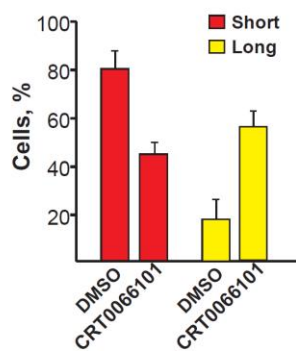
Figure 24. PKD inhibition reduces mitochondrial fission rate in pancreatic cancer PANC1 cells. (A) Fluorescence microscopy images of PANC1 cells treated with vehicle (DMSO) or PKD inhibitor (10µM CRT 0066101) for 14 hours. Mitochondria were stained with MitoTracker Red and nuclei were counterstained with DAPI. Scale bar: 20 µm. (B) Quantification of the mitochondrial morphology of cells shown in (A). Mitochondrial shape was classified as short (round or rod-like, 2-5µm long), or long (tubular or fused, more than 5µm long) and displayed as percentage of cells having majority of their mitochondria falling in the respective category. For each group at least 100 cells were counted. Data are shown as mean with SD of two independent experiments.
