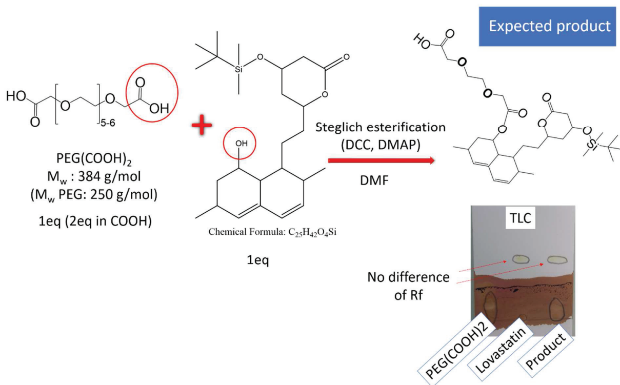
Scheme 13 Steglich esterification procedure between lovastatin and PEG(COOH) 2 . The product was analyzed by thin layer chromatography (TLC) (mobile phase Et 2 O; revelator: I 2 and a solution of KMnO 4 ). The product is a mixture of the two initial compounds.
