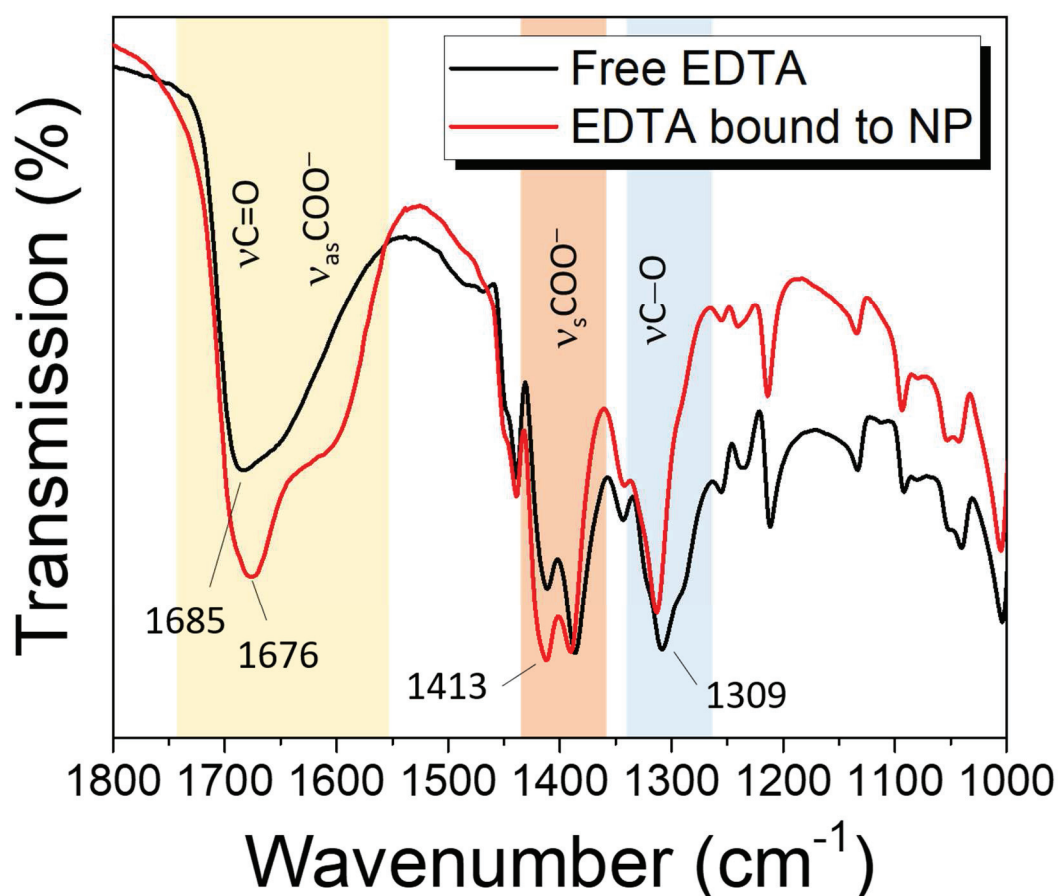
Figure 31 FTIR-ATR spectrum of GdF 3 NPs prepared in the presence of EDTA (red line) compared to the spectrum of free EDTA (black line).
