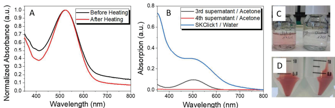
Figure 57 SKClick1 particles. A) Absorption spectra before and after heating the particle suspension with LEM-A. B) Purification steps of SKClick1 followed by absorption spectroscopy. C) Picture of the 3 rd (pink) and 4 th (colorless) supernatants. D) Picture of the pellets of SKClick1 after purification.
