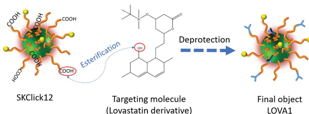
Scheme 11 First strategy for lovastatin coupling to SKClick 12 nanoparticle.
