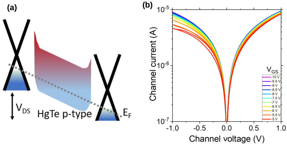
Figure 4.7 – Zone III: V_{GS} < V_D , regime p-p'-p (a) Band alignment of the graphene/HgTe/graphene junction in the p-p'-p configuration. (b) The associated quasi-ohmic I-V curves at different gate voltages at 240 K
