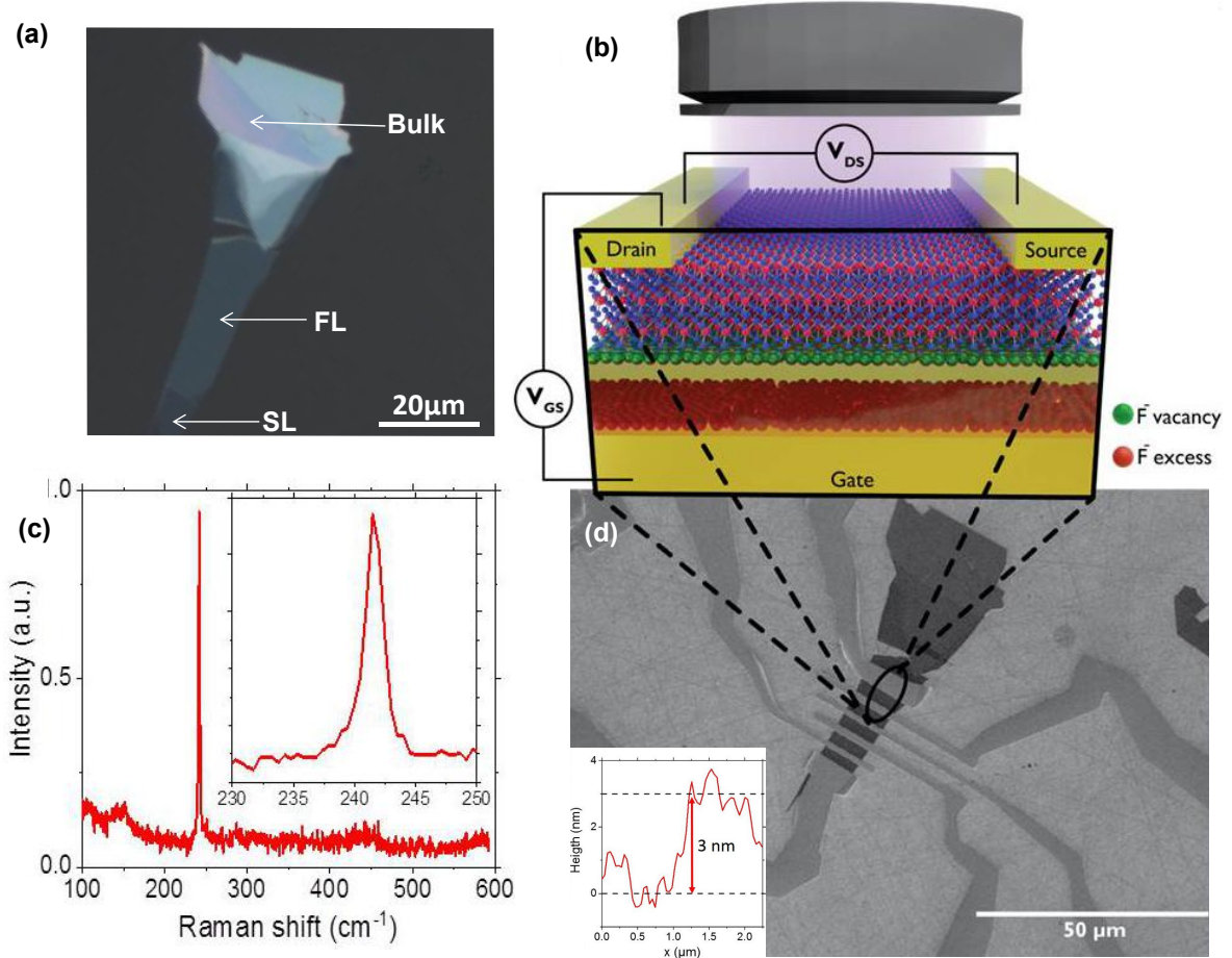
Figure 3.4 – (a) Optical image of exfoliated MoSe 2 on LaF 3 substrate: By optical contrast, single layer and few layers can be distinguished from bulk material. (b) Scheme of the photodetector device and electrical connections. Tri-layer MoSe 2 on a LaF 3 substrate is contacted by two gold electrodes (drain and source), and gating is performed by applying a bias between drain and a bottom gold contact below LaF 3 . Top access allows addressing optically the MoSe 2 channel while reaching higher carrier density thanks to the ionic glass gate. (c) Raman spectra of the MoSe 2 flake with A 1g mode at 242 cm -1 . The inset is a zoom on the peak relative to the A 1g mode of MoSe 2 . Done at HORIBA Scientific by Abdelkarim Ouerghi and Thibault Brule. (d) SEM image of the flake and gold contacts. Length and width of the channel are 2.6 and 9.3 μm respectively. The inset height profile from AFM measurements with a thickness of 3 ± 0.5 nm corresponding to 3-4 layers MoSe 2 .
