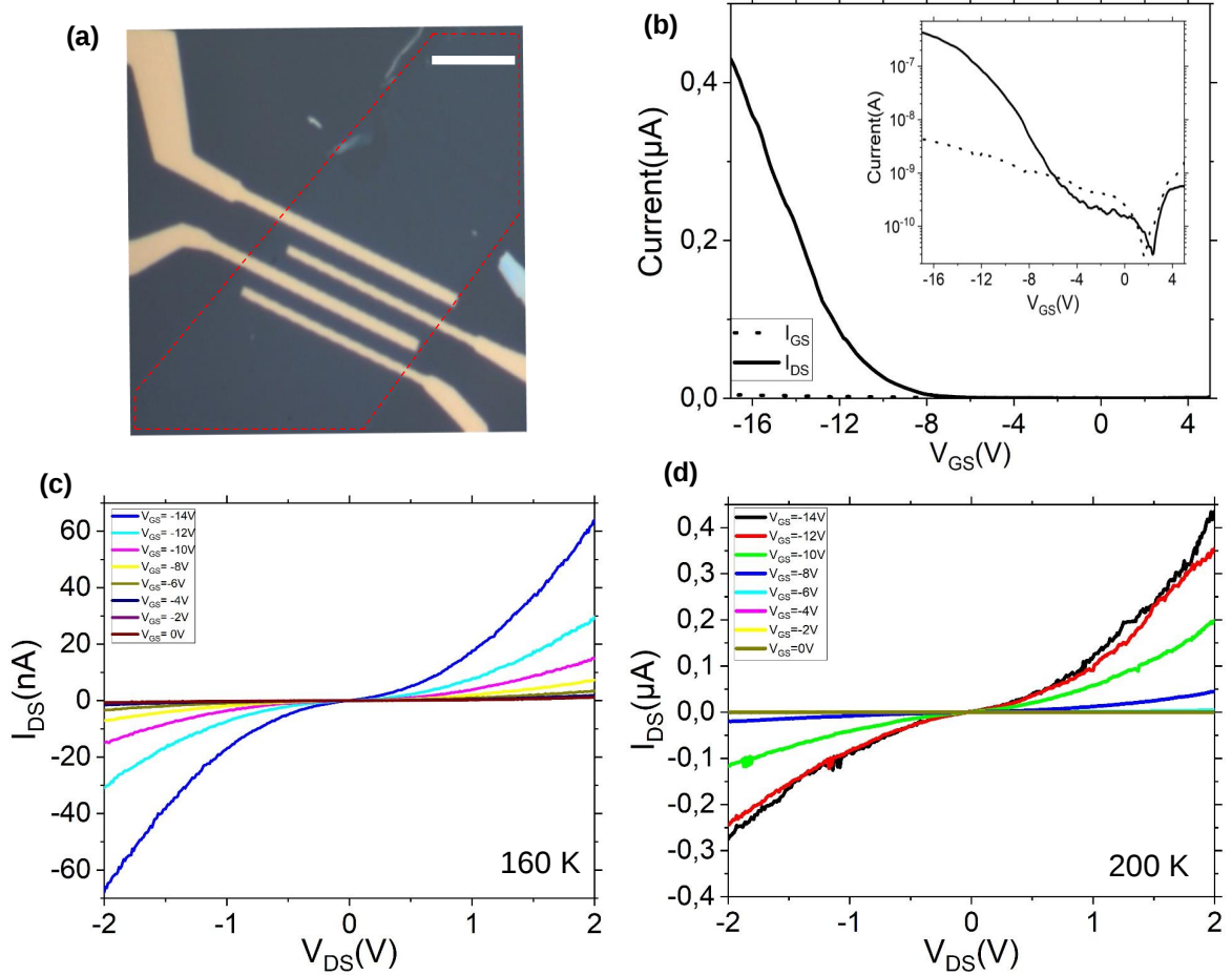
Figure 3.7 – (a) Optical image of the multi-electrodes device fabricated using e-beam lithography, the region in dash line is the flake. Scale bar: 10 μm. (b) Transfer curve at 200 K under 2 V drain-source bias with LaF 3 gating showing hole conduction in WSe 2 flake. Inset: Transfer curve in logarithmic scale. (c) I DS -V DS curves for different gate voltages with increasing current with the gate voltages at 160 K. (d) I DS -V DS curves for different gate voltages with increasing current with the gate voltages at 200 K.
