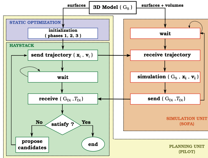
FIGURE 4.6 – Communication pipeline between the planning and simulation units.
