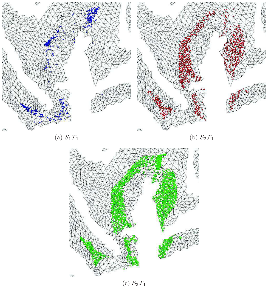
FIGURE 6.17 – Zoom on the Pareto fronts of \mathcal{M}_1 in blue, \mathcal{M}_2 in red, and \mathcal{M}_3 in green
