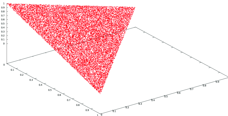
FIGURE 6.5 – Uniform sampling of 20,000 combinations of parameters w_i using a Dirichlet distribution for n = 3 weights and associated objective functions.
