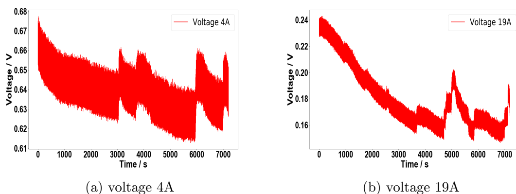
Figure 4.21: Raw voltage signal(Serpentine) (a) 4A (b) 19A
