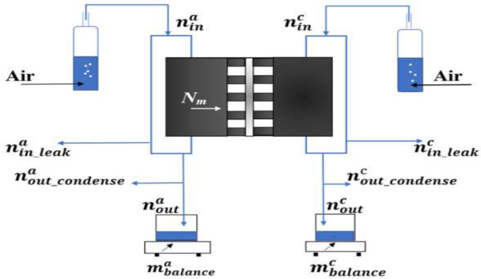
Figure 2.13: Experimental setup with losses
