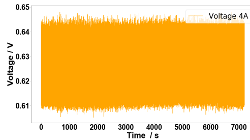
Figure 4.30: Voltage 4A
