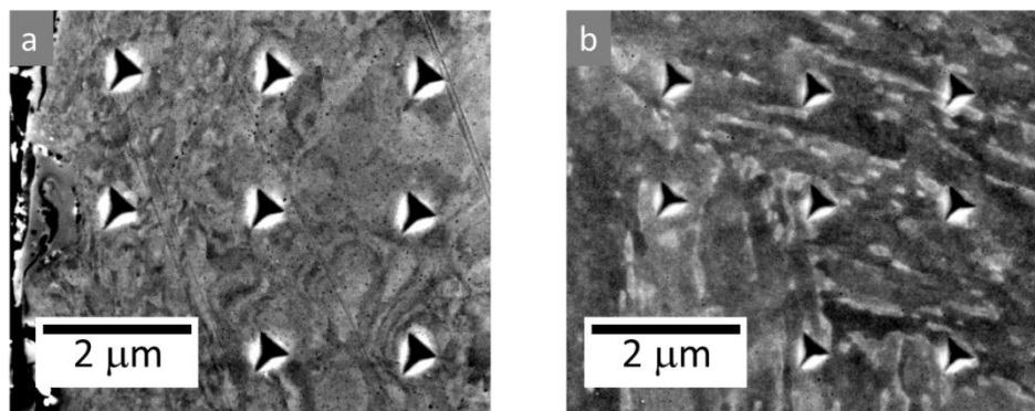
Figure 4-14. SEM images revealing the microstructure of the substrate taken a) away of the interface b) at the interface. The microstructure at the interface is made of very small grains associated with deformation patterns while the microstructure in the bulk shows a regular lath microstructure.
