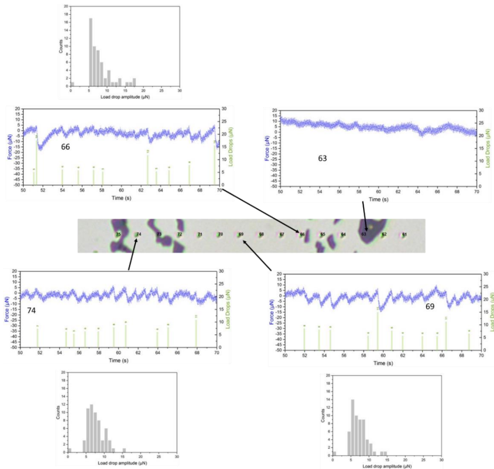
Figure 5-35. Results of the statistical analysis of the load drops relative to the location in the dendritic arm.
