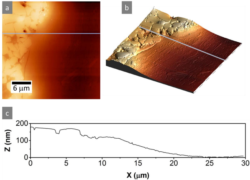
Figure 4-8. (a) AFM topography image of the surface at the interface after CMP with colloidal silica. The blue line represents the position of the profile shown in the figure (c). (b) 3D representation of the topography image shown in (a). (c) Height profile at the interface.
