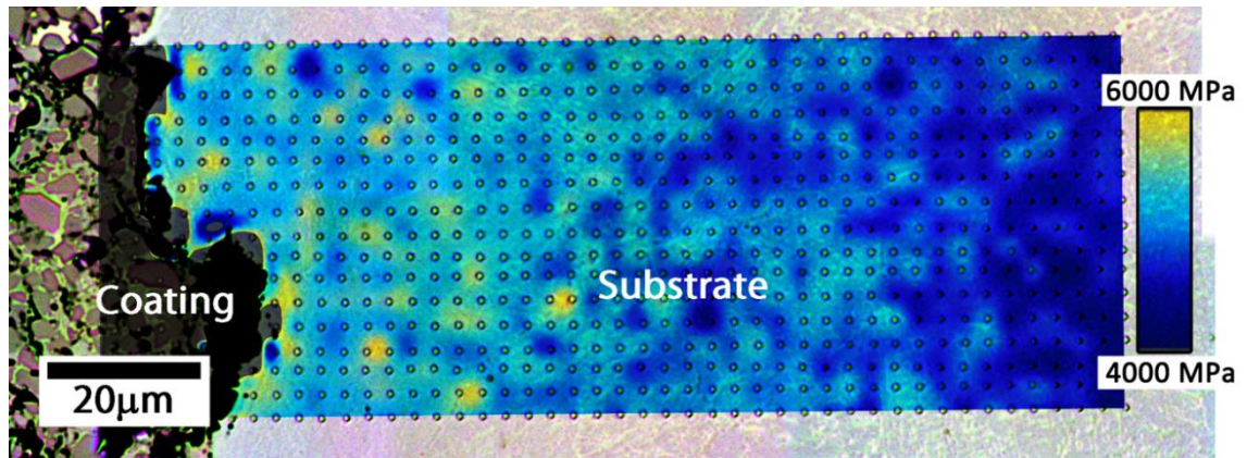
Figure 4-11. Nanohardness cartography built from a 17 \times 45 nanoindentation array at the interface between the coating and the substrate. The hardness map is superimposed to the optical microscopy image of the indented area.
