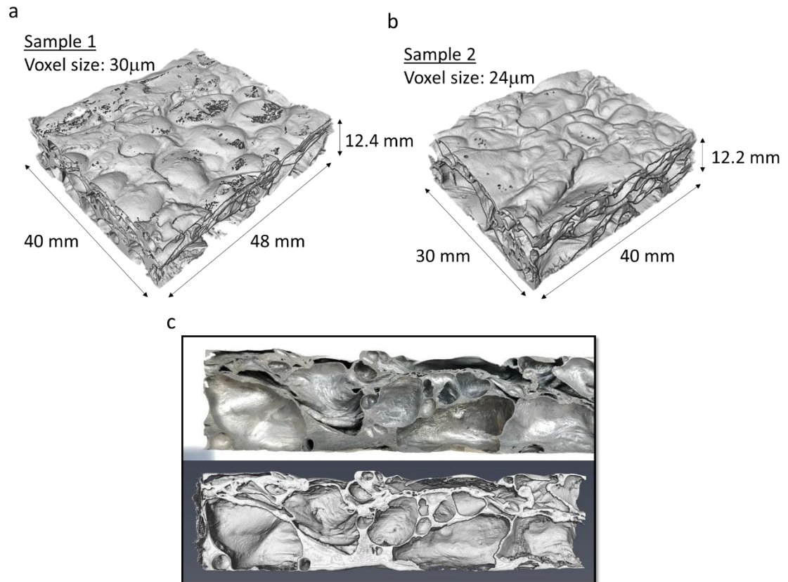
Figure 5-1. (a) Reconstruction of sample 1 (voxel size 30µm) (b) Reconstruction of sample 2 (voxel size 24µm) (c) and (d) Comparison of the same cross section obtained from a photograph (top) and x-ray tomography (bottom)
