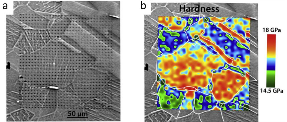
Figure 3-10. Hardness cartography applied to a plasma-nitrided 316 stainless steel (a) SEM image of the array of indentations used to reconstruct the hardness map (b) Hardness map revealing the heterogeneities of the hardness of the microstructure [113]
