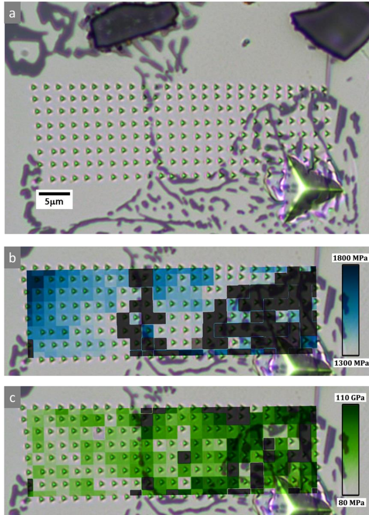
Figure 5-25. (a) Optical micrograph of the surface after indentation. The array is made of 10x25 indentations. (b) Nanohardness cartography reconstructed from the array shown in (a). Each square represents a single nanohardness value. (c) Cartography of Young's modulus from the array shown in (a).
