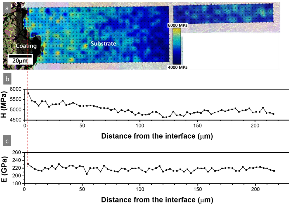
Figure 4-12. (a) Complementary nanohardness cartography built from a 6*30 nanoindentation array (b) Hardness as a function of the distance from the interface. The hardness remains constant
