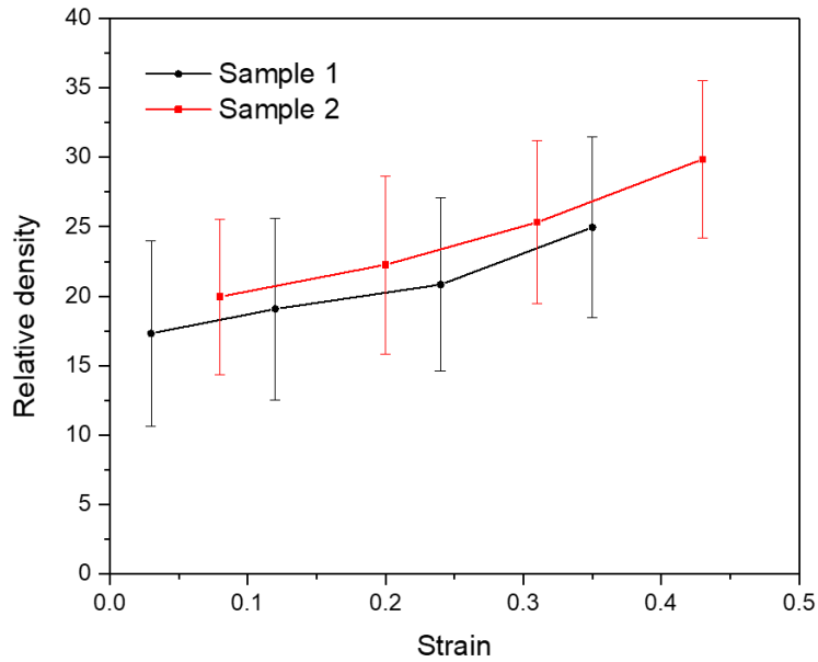
Figure 5-17. Evolution of the relative density as a function of strain for the two samples tested.
