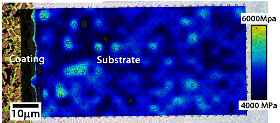
Figure 4-13. Nanohardness cartography built from a 15*30 nanoindentation array at the interface between the coating and the substrate. The substrate was polished with a diamond solution up to 1µm prior to the deposition of the coating. No hardening is observed in the substrate.
