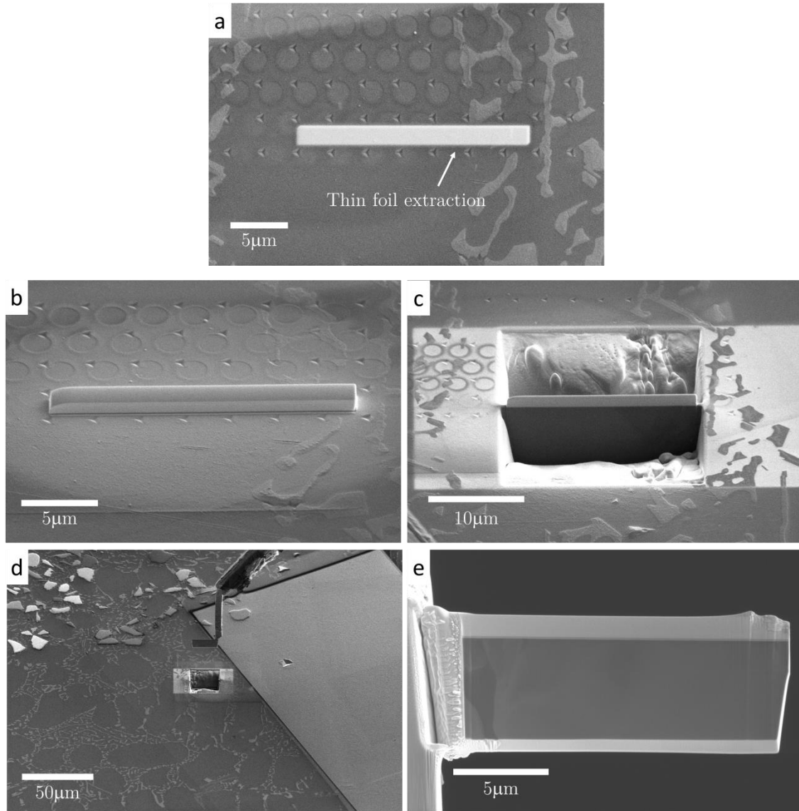
Figure 5-9. Procedure of the FIB lift-out technique used to prepare thin foils for TEM imaging. (a) The thin foil is extracted between two lines of indents inside a 5x15 array. (b) A layer of platinum is deposited to protect the surface from sputtering. (c) The thin foil is prepared by milling trenches. (d) The thin foil is extracted using a micromanipulator. (e) The foil is attached to a high purity beryllium grid and thinned down to be transparent to electrons.
