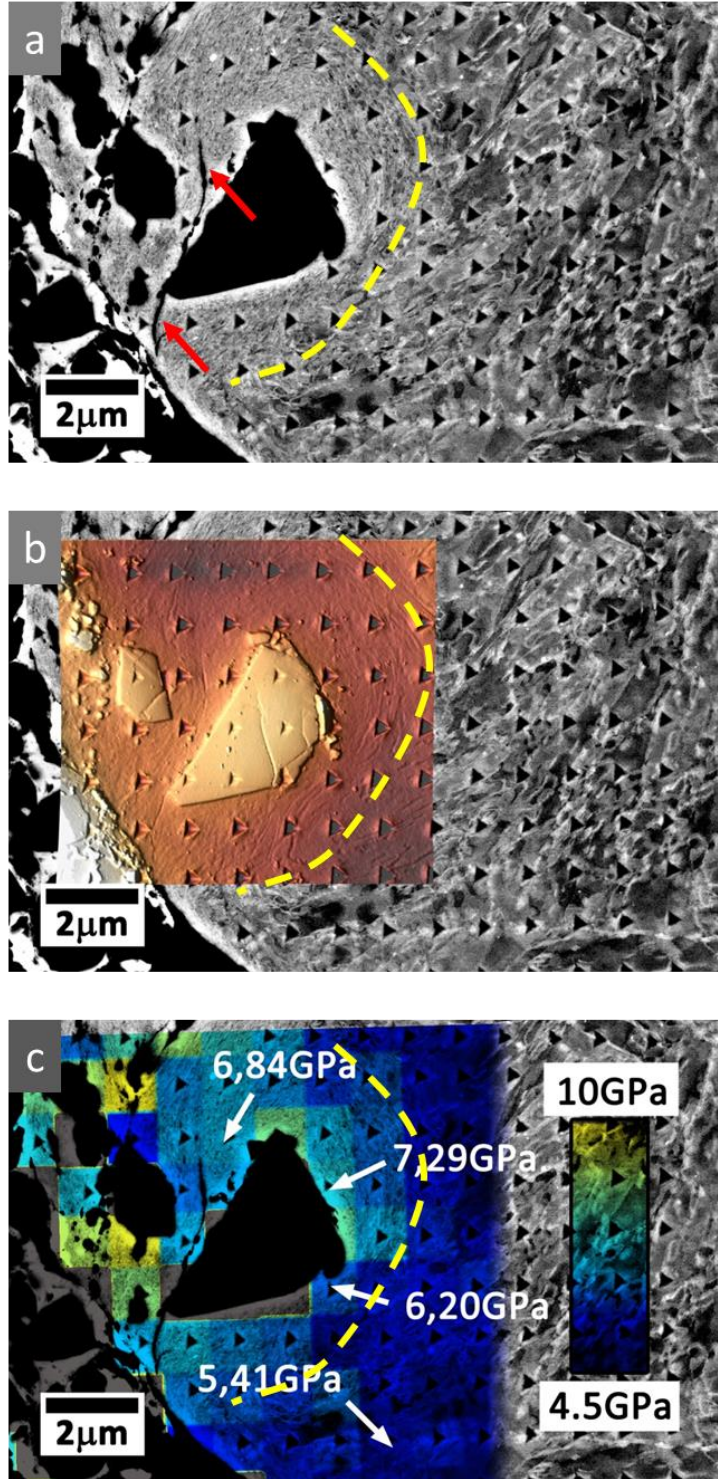
Figure 4-17. Nanoindentation array on an alumina particle. (a) SEM image showing the microstructure around the particle. The yellow line delimits an ultra-fine-grained structure in the vicinity of the particle. (b) The same area imaged by AFM (3D top view) (c) Nanohardness map around the alumina particle.
