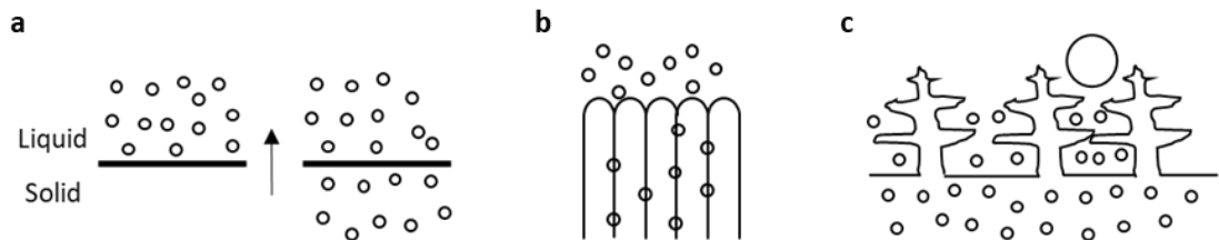
Figure 2-10. Influence of interface shape on particles. (a) The planar interface can result in pushing (left) or engulfment (right). (b) Cellular interface showing pushing at interface and entrapment between cells. (c) Dendritic interface; small particles are entrapped in interdendritic spaces while large particles are pushed [76]
