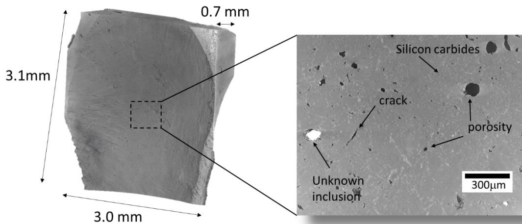
Figure 5-4. High-resolution scan of the piece aluminum foam (left) with a zoomed in view (right) revealing some microstructural features of the materials like porosity inside the walls, cracks, and silicon carbides.
