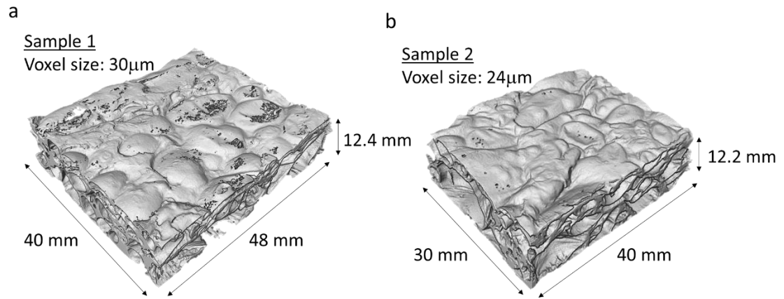
Figure 3-6. A tomographic image of the two samples used to characterize the morphology of the foam. The two samples have different dimensions resulting in different voxel size. (a) Reconstruction of sample 1 (voxel size 30 μm) (b) Reconstruction of sample 2 (voxel size 24 μm)
