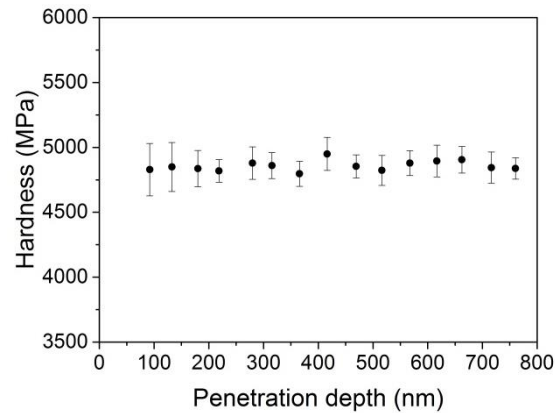
Figure 4-15. Nanohardness as a function of the penetration depth. Each data point is the average of 15 hardness values obtained from indentations made at the same depth for a total of 225 indentations. The errors bars correspond to the standard deviation calculated from those 15 values.
