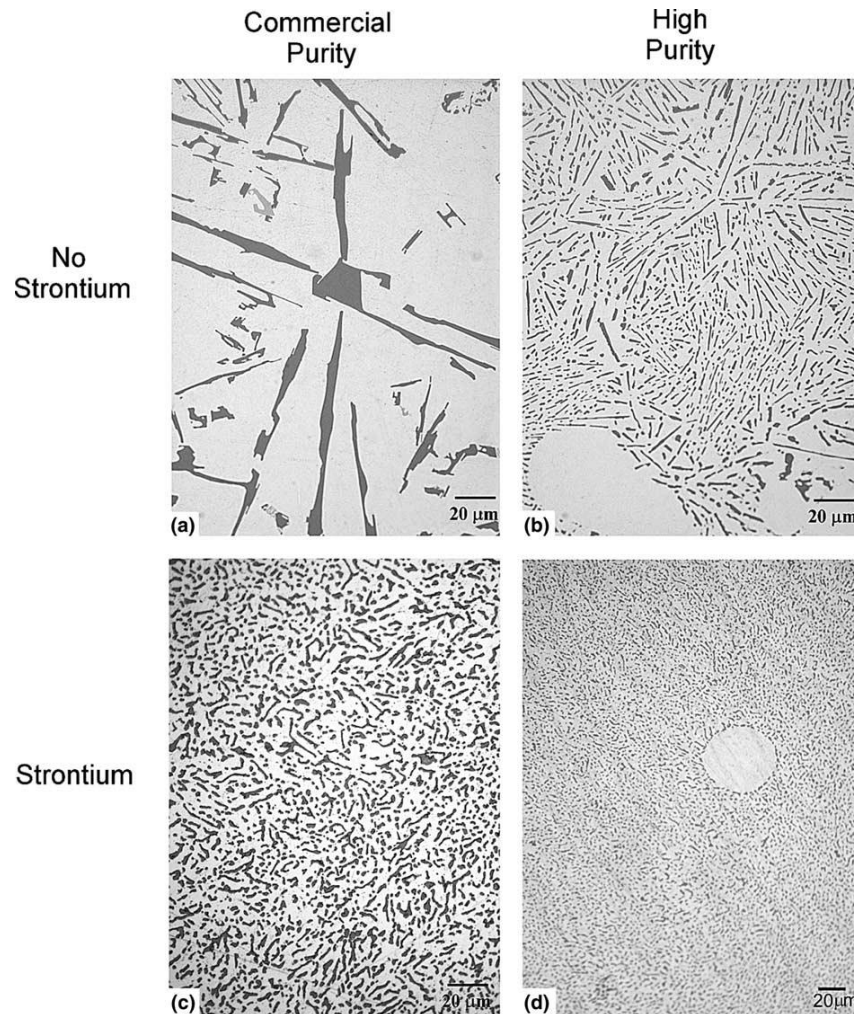
Figure 2-8. Different microstructures of commercial and high purity aluminum with and without addition chemical modifiers (Sr here) [69]
