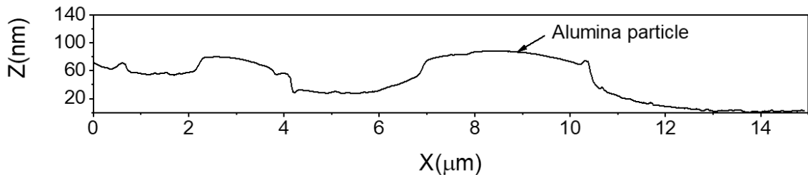
Figure 4-16. Height profile around the particle along the blue line shown in Figure 4-17b.
