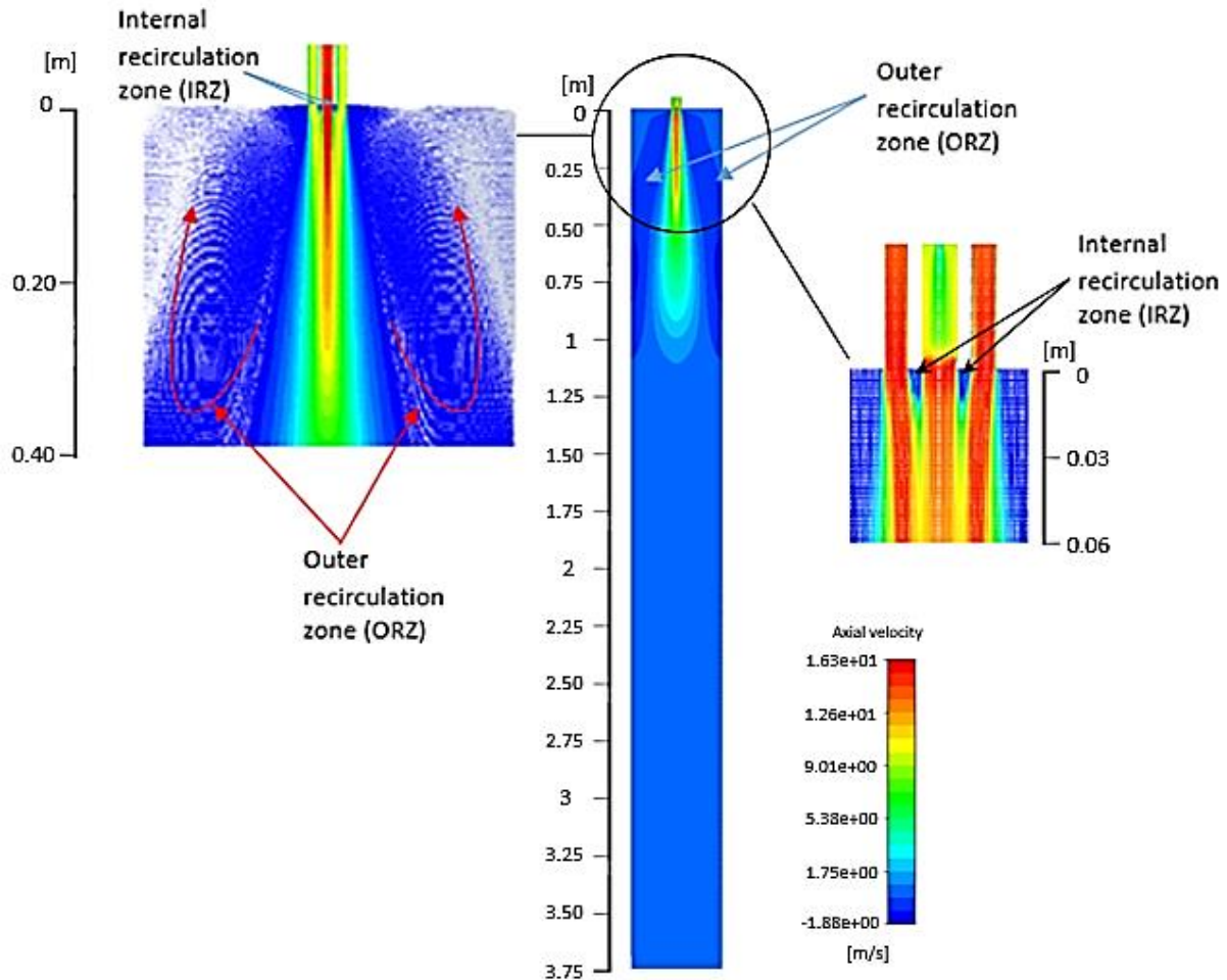
Figure VII.8: Axial velocity contours of the homogeneous phase for Pine flame
