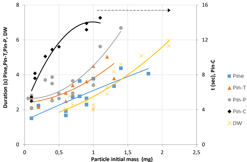
Figure V.19: Total burnout duration in PCS at 800°C
