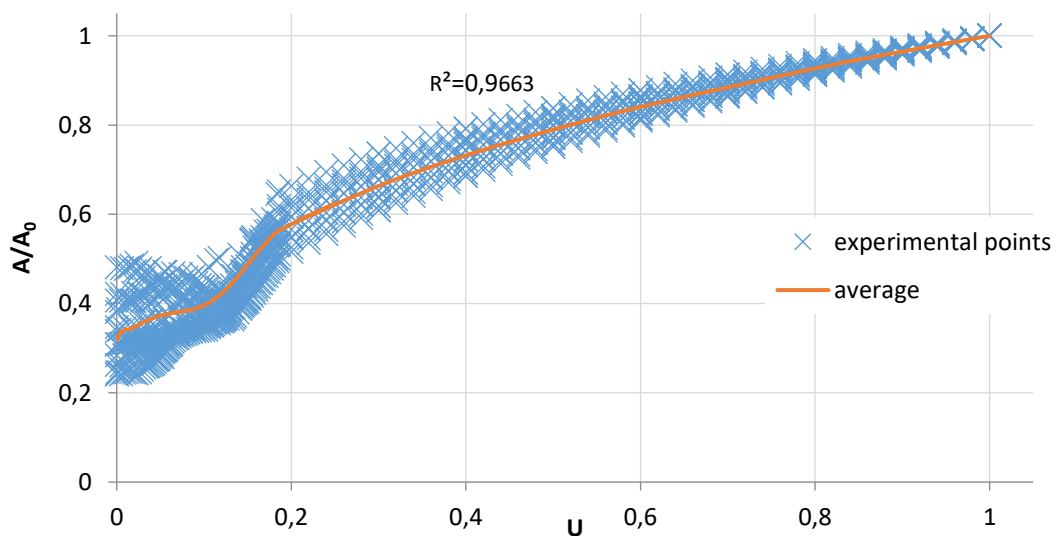
Figure V.21: Average area evolution of Pine versus the unburnt fraction at 800°C
