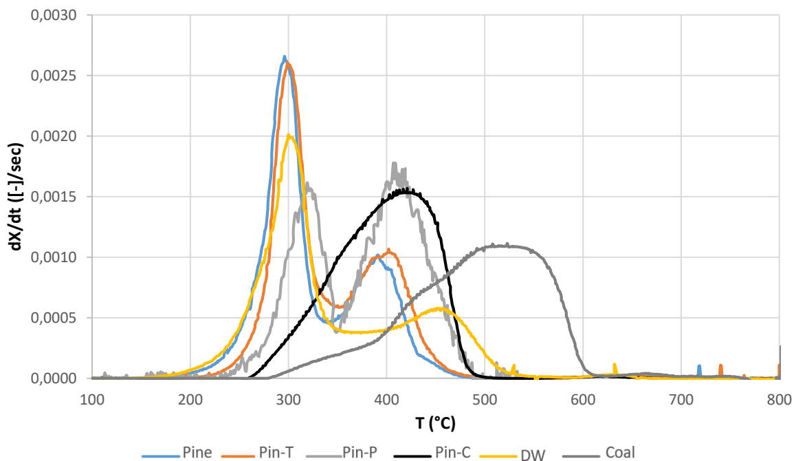
Figure V.4: Comparison of the time derivative of the mass fraction of the combustion of different fuels (10°C/min to 800°C with air)
