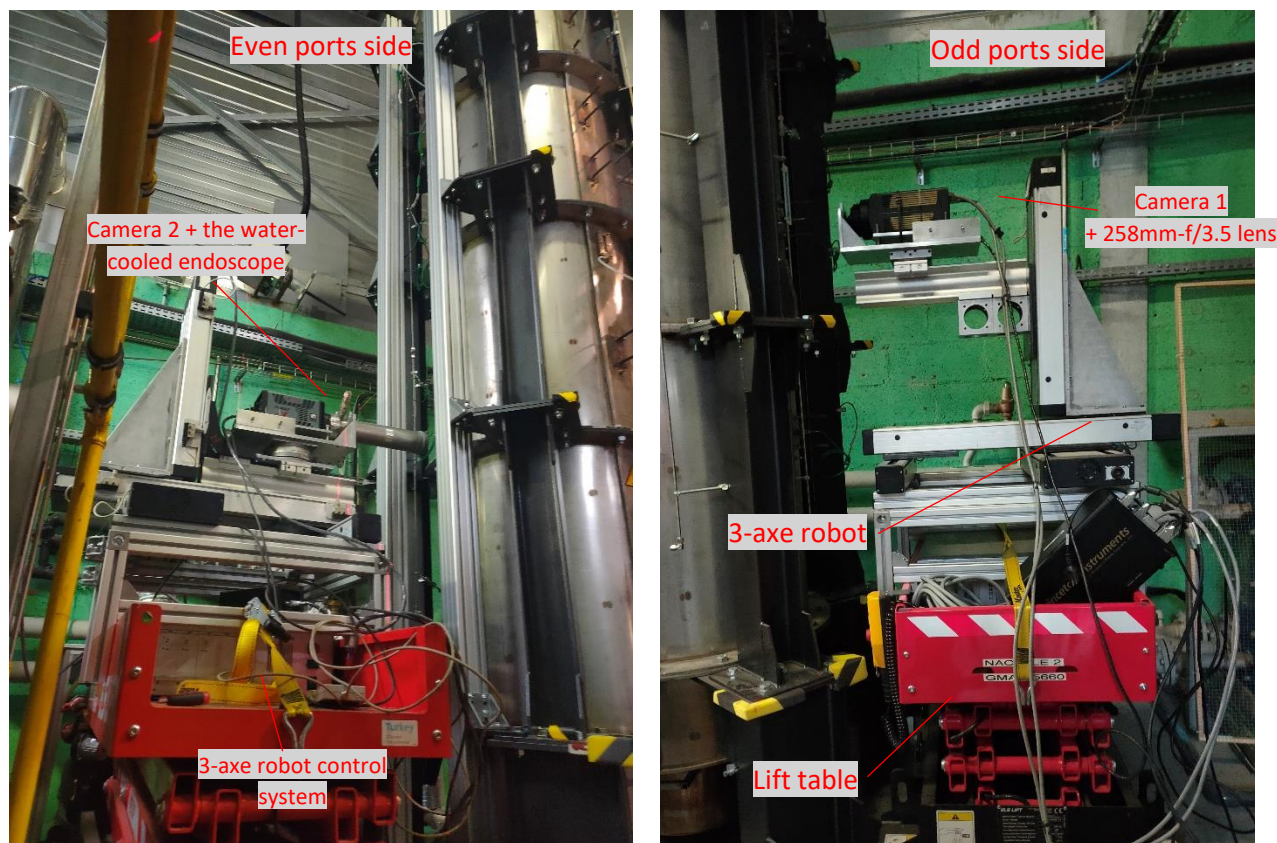
Figure III.21: The optical systems held by the 3-axe robot on the lift table from both sides of the chamber
