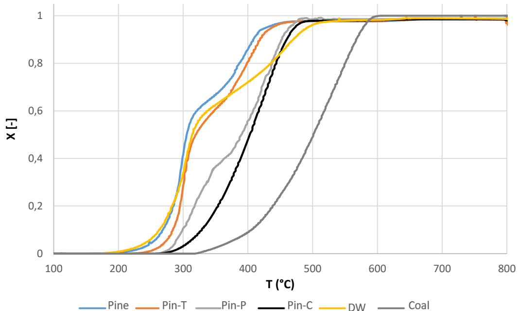
Figure V.3: Comparison of the conversion curves of the combustion of different fuels (10°C/min to 800°C with air)
