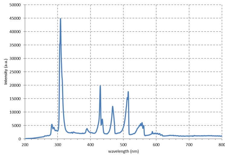
Figure III.18: Typical chemiluminescence spectrum observed in partially premixed flames [171]
