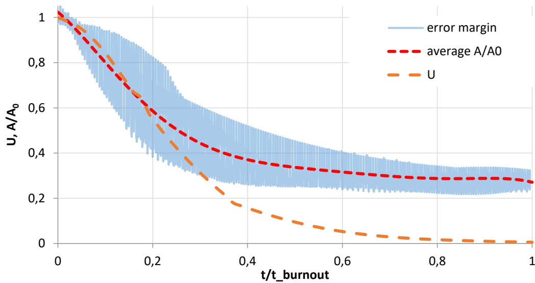
Figure V.20: Normalized area ( A/A_0 ) (in PCS) and unburnt fraction ( U ) (in HTR) vs the normalized combustion time of Pine at 800°C
