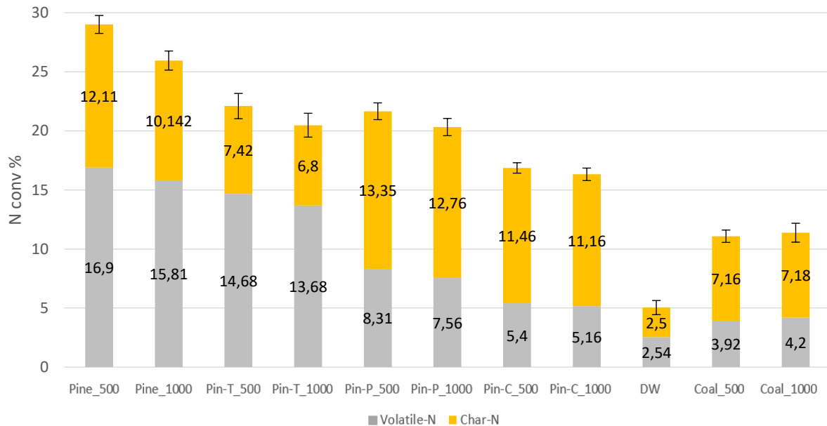
Figure V.11: Char (Char-N) and volatile (Volatile-N) nitrogen conversion to NO during two combustion stages for different biomass sizes (500 \mu\text{m} and 1000 \mu\text{m} ) in HTR at 800°C
