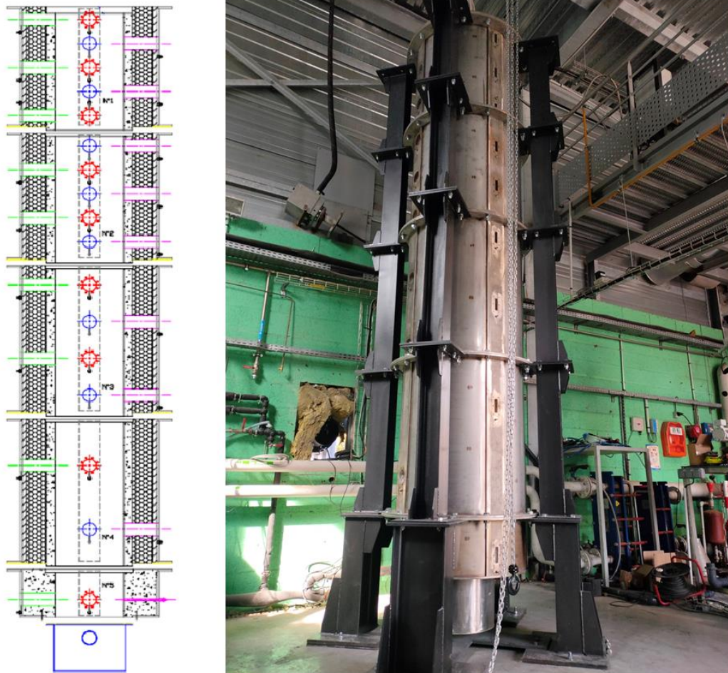
Figure A.1: The final furnace structure with several ports distribution
