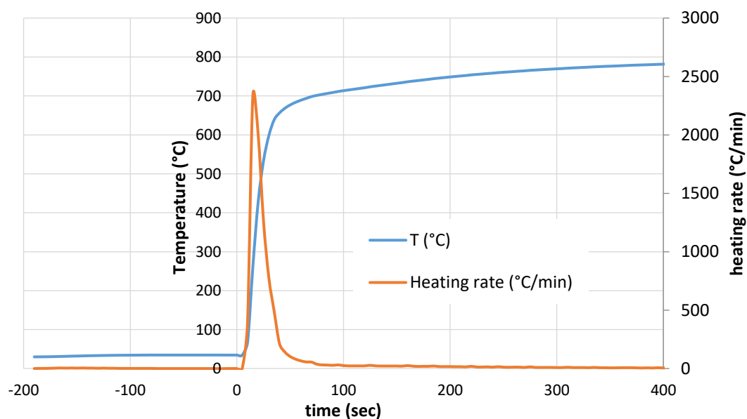
Figure II.7: Typical sample temperature evolution (insertion at t=0 )
