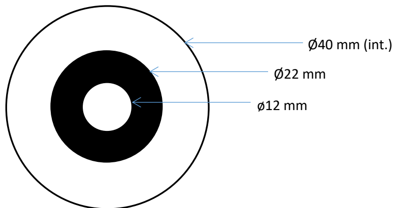
Figure III.6: bluff-body dimensions
