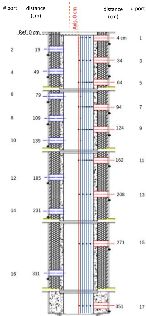
Figure VII.3: Optical accesses for flame imaging and gas sampling points along the reactor length (black dots). They lie on eight vertical axis (blue lines) parallel to the axis of the chamber (red line). The axial distance from the burner (in cm) is indicated next to the port numbers (1 to 17).
