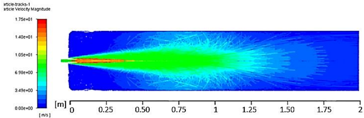
Figure VII.9: Trajectories of 1400 particles of Pine in reactive flow color-scaled by their velocities
