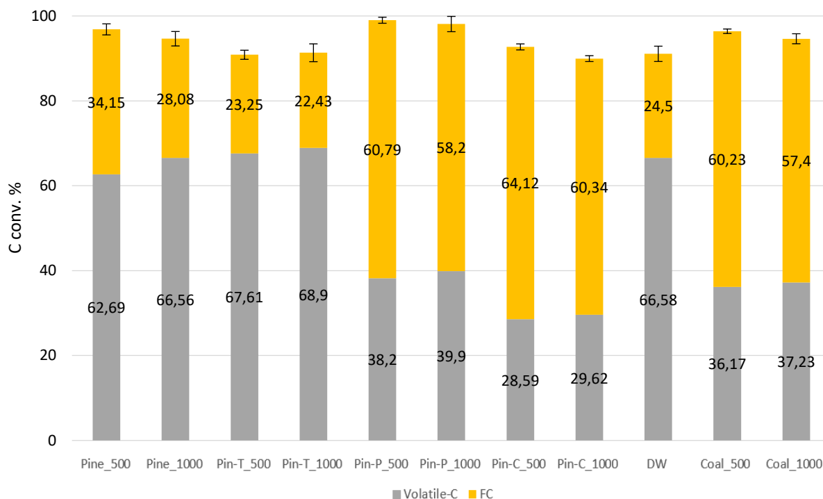
Figure V.9: Char (FC) and volatile (Volatile-C) carbon conversion to CO and CO 2 during two combustion stages for different biomass sizes (500 \mu\text{m} and 1000 \mu\text{m} ) in HTR at 800°C
