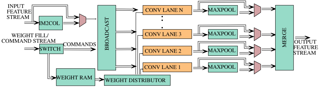
Figure 6.4: The detailed architecture of the streaming accelerator.
