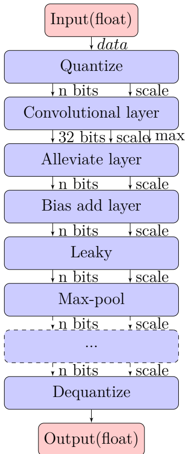
Figure 5.1: The network design for quantization
