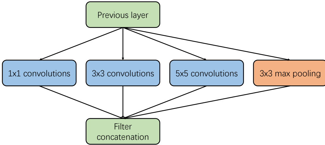
Figure 2.7: The structure of Inception Naive version
