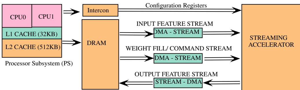
Figure 6.2: The overall of hardware architecture .
