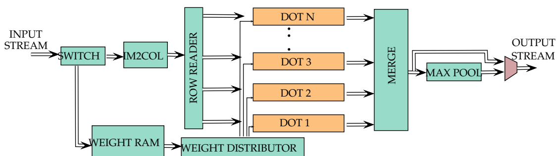
Figure 7.7: The detailed architecture of the Accelerator
