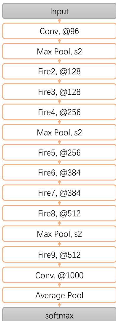
Figure 2.13: The structure of SqueezeNet
