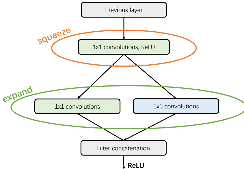
Figure 2.12: The Fire Module in SqueezeNet
