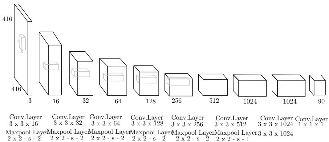
Figure 2.17: The structure of tiny-YOLO
