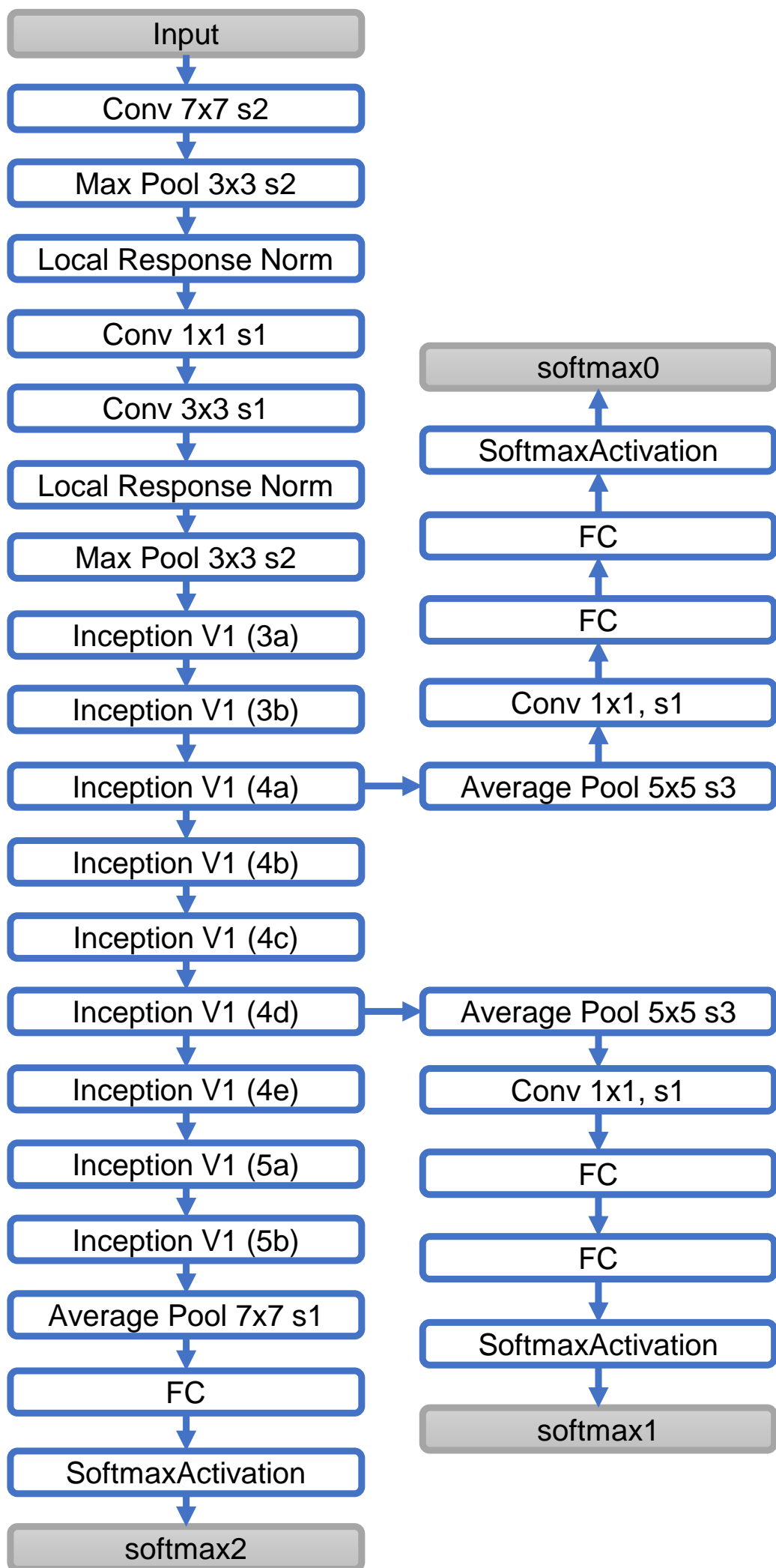
Figure 2.9: The structure of GoogLeNet [1].
