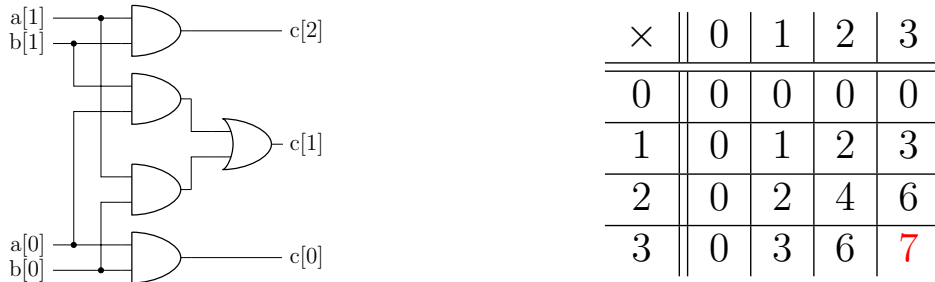
Figure 7.2: An approximate 2 bits unsigned multiplier.
