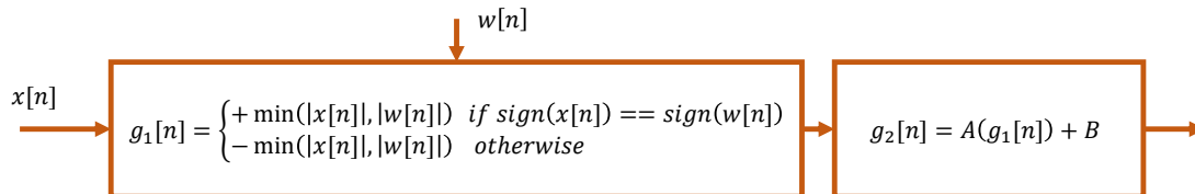
Figure 8.2: The approximate multiplication system constructed by the min-selector.
