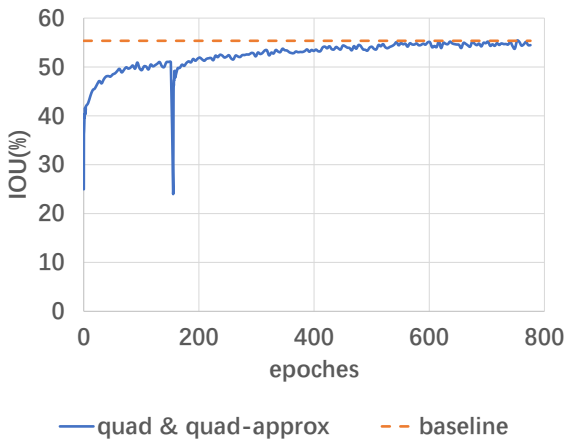
Figure 7.4: IOU of quad network and then quad-approx network, baseline correspondence to original tiny-YOLO.
