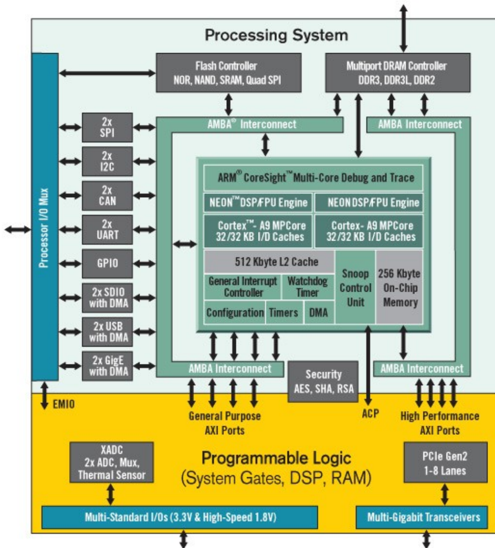
Figure 3.10: Zynq APSoC architecture
