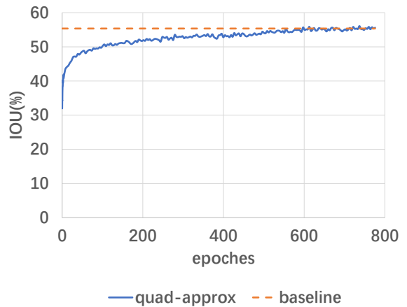
Figure 7.5: IOU of quad-approx network applied at the beginning of training, baseline correspondence to original tiny-YOLO.
