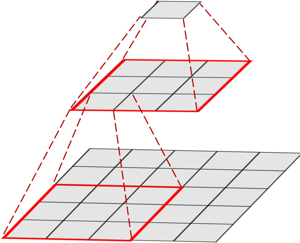
Figure 4.1: The fields of view of the 5 \times 5 kernel replaced by 3 \times 3 kernels
