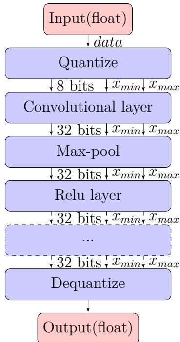
Figure 4.3: In continuous quantization, the quantized output, minimum and maximum float could be used as input for the next layer directly, and the dequantize layer is as the end of all quantized layer.
