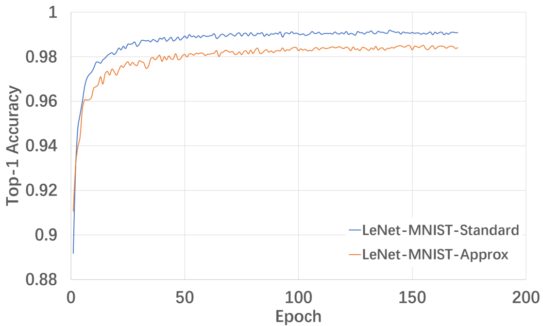
Figure 8.5: Top-1 accuracy of LeNet applied to MNIST.
