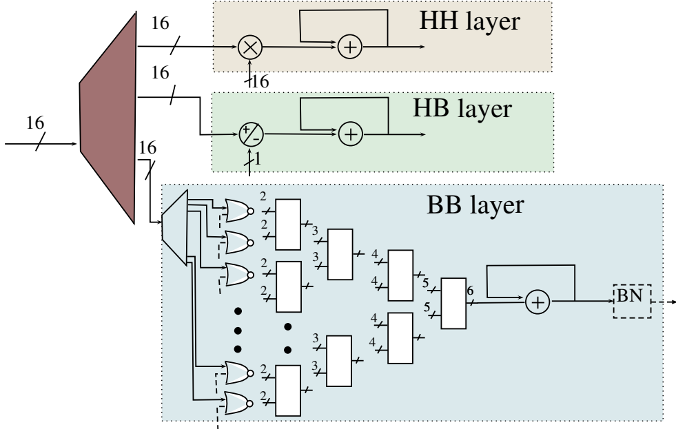
Figure 6.5: The detailed architecture of the convolutional lanes.
