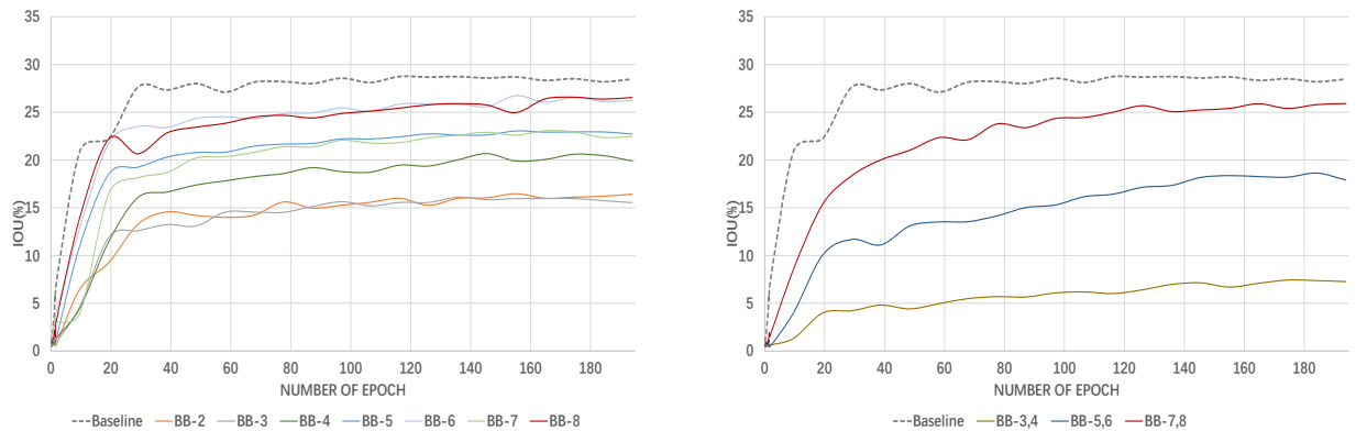
Figure 6.1: IOU along the training of the 12 architecture on the DAC dataset.
