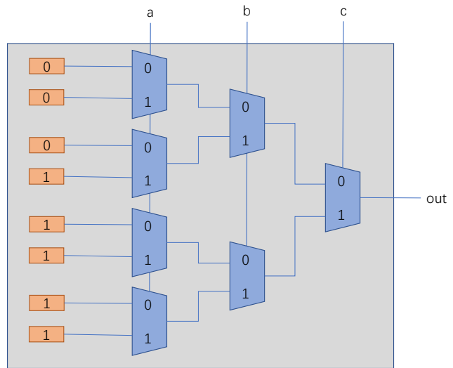
Figure 3.8: A 3-input LUT for the logic operation
