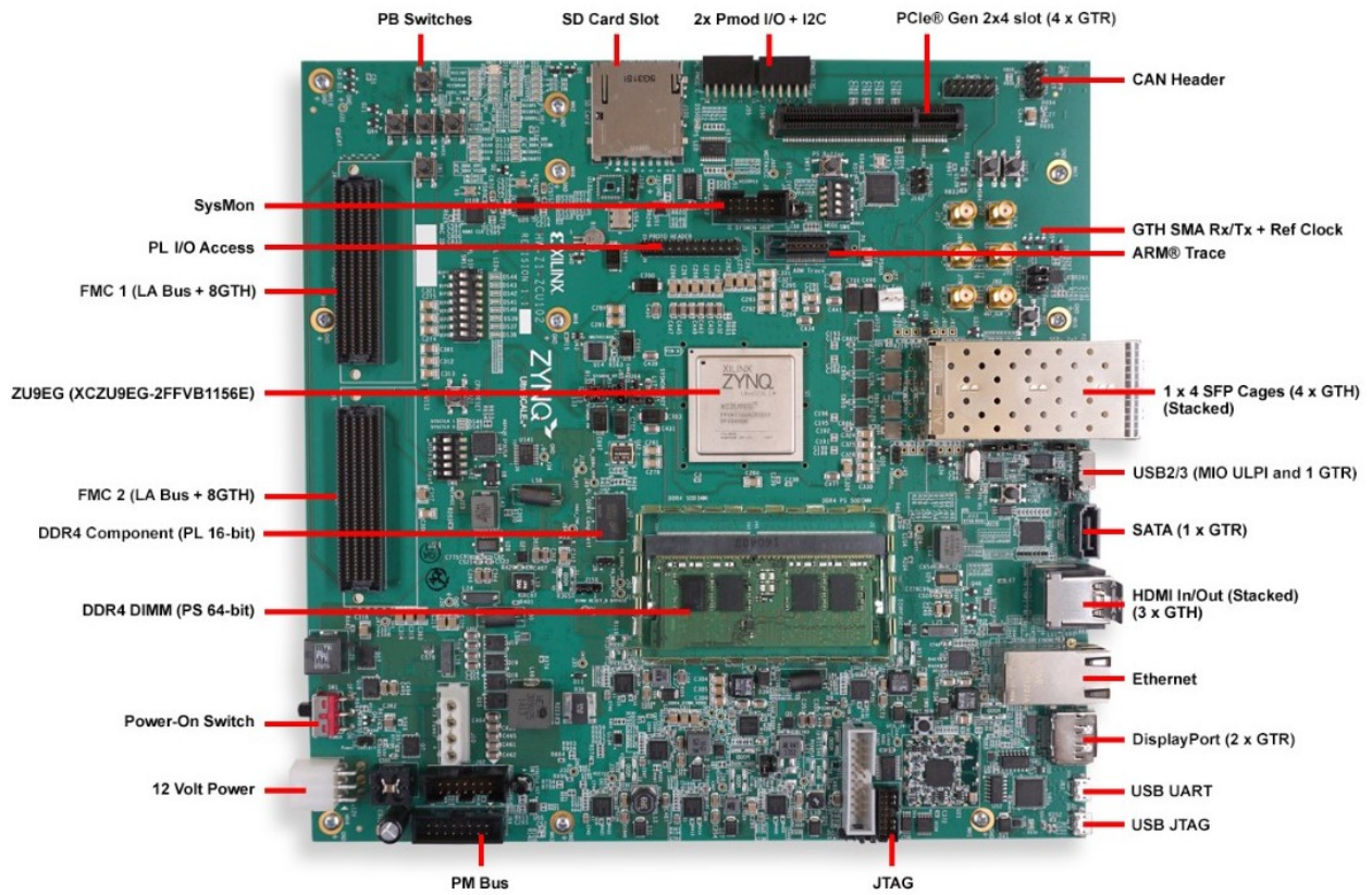
Figure 3.12: The devices and interfaces in ZCU102 board
