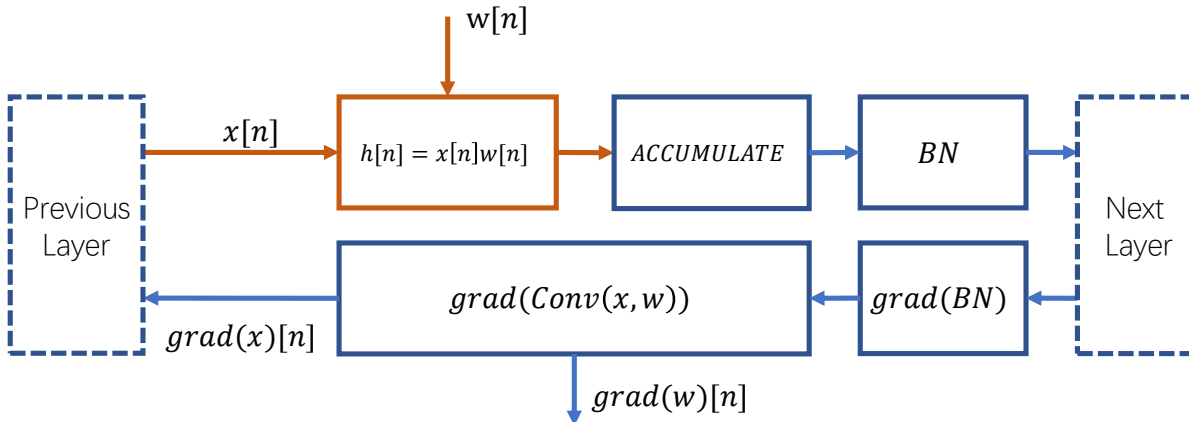
Figure 8.1: The convolutional layer is considered as a system.
