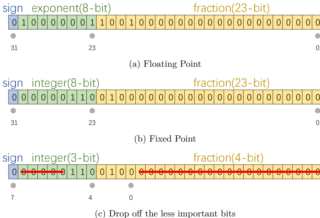
Figure 4.2: The formats of decimals in computers.
