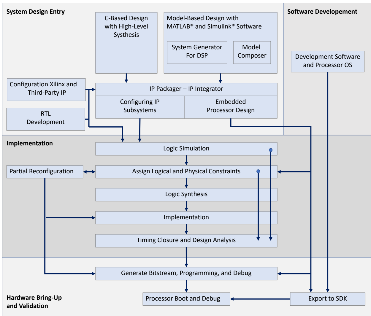
Figure 3.9: Vivado Design Suite High-Level Design Flow
