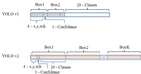
Figure 2.16: Content of the bounding boxes
