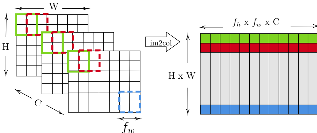
Figure 6.3: Image to Matrix (im2col) Transformation.
