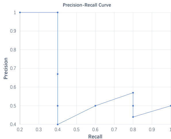
(b) The Precision-Recall Curve.
