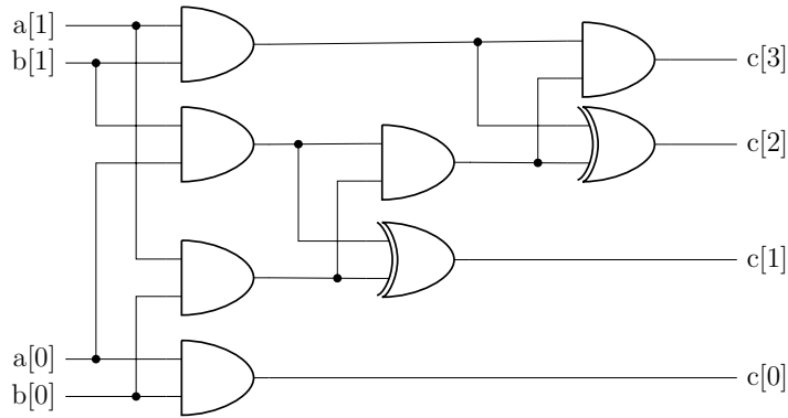
Figure 7.3: One of the standard multiplier for 2 bit operands
