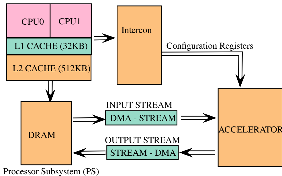
Figure 7.6: The overall of hardware architecture
