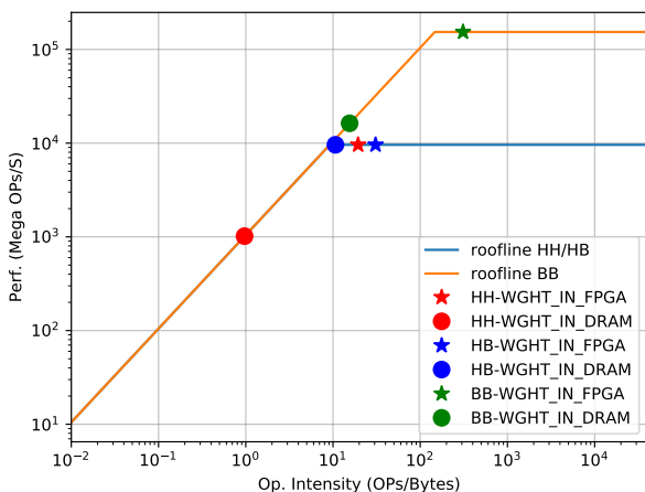
Figure 6.6: The architectural choices and their explanation with roofline.
