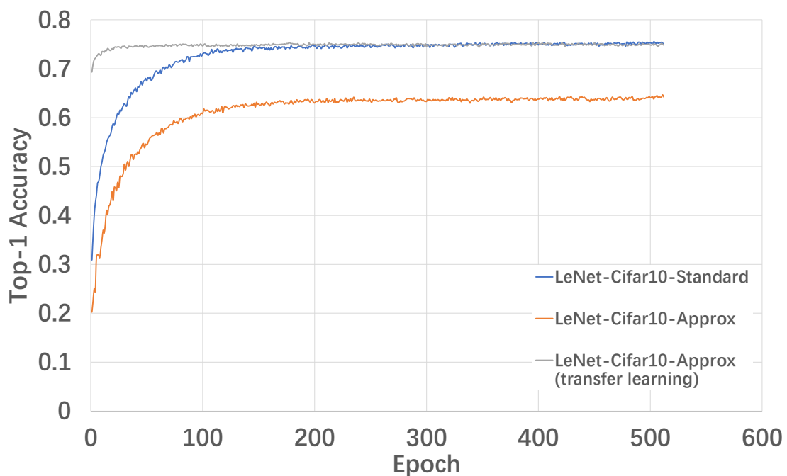
Figure 8.6: Top-1 accuracy of LeNet applied to Cifar10.
