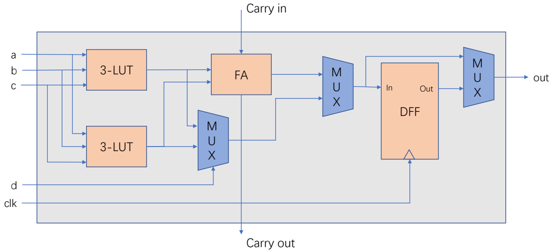
Figure 3.6: The architecture of Configurable Logic Blocks
