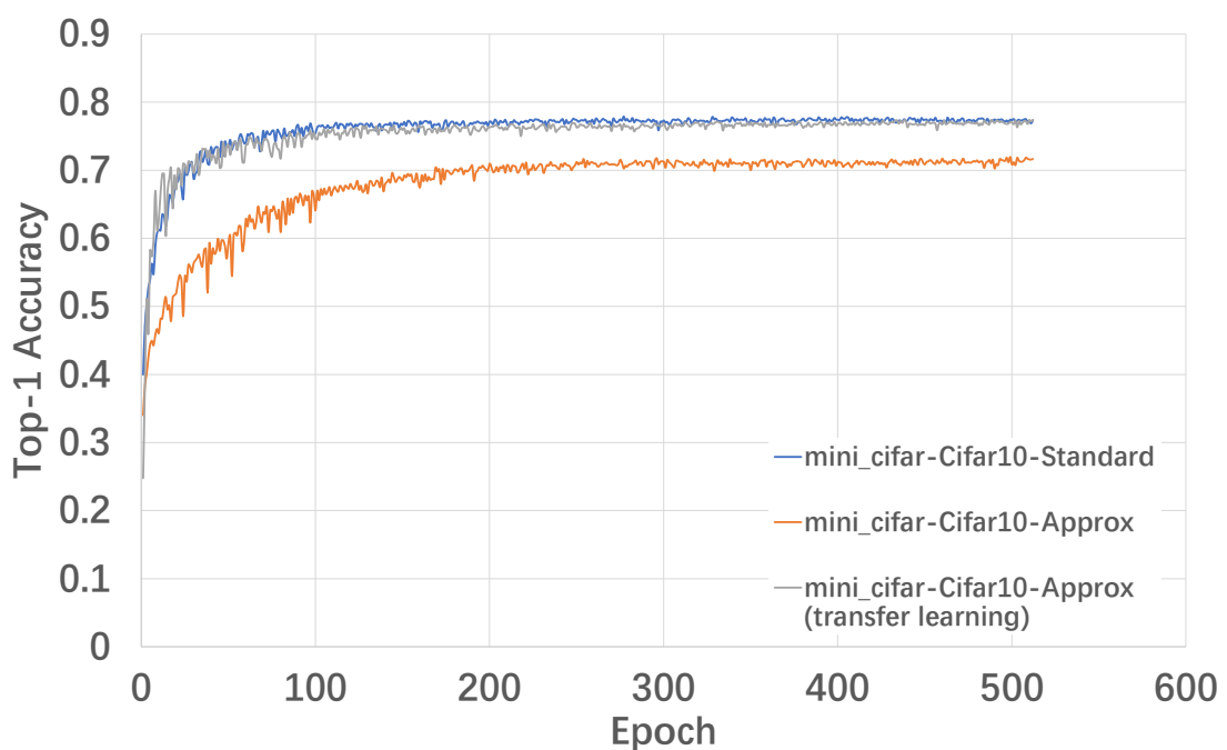
Figure 8.7: Top-1 accuracy of mini-cifar applied to Cifar10.
