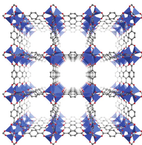
Figure 2-6 A portion of the crystal structure of \text{Zn}_4\text{O}(\text{BDC})_3 (MOF-5). Blue tetrahedra represent \text{ZnO}_4 units, while gray and red spheres represent C and O atoms, respectively; H atoms are omitted for clarity.
