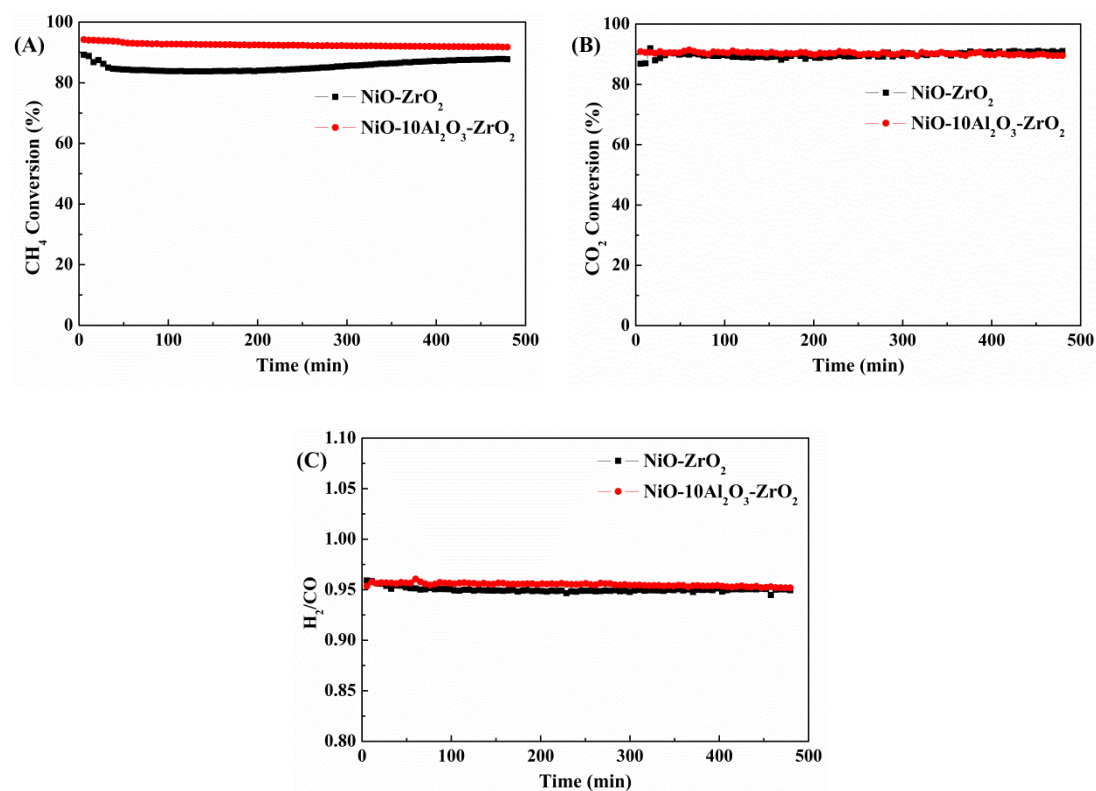
Figure 5-11 (A) CH 4 conversion , (B) CO 2 conversion and (C) H 2 /CO ratio in isothermal conditions (700 °C) on NiO-10Al 2 O 3 -ZrO 2 in the presence of CH 4 :CO 2 :Ar=10:10:80, GSHV=48,000 h -1
