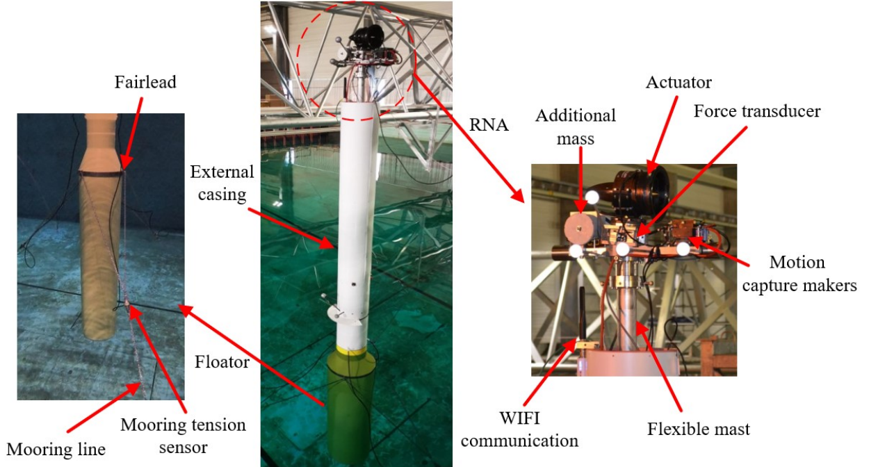
Figure 5.3 – Description of the FWT experimental set-up (Arnal 2020).
