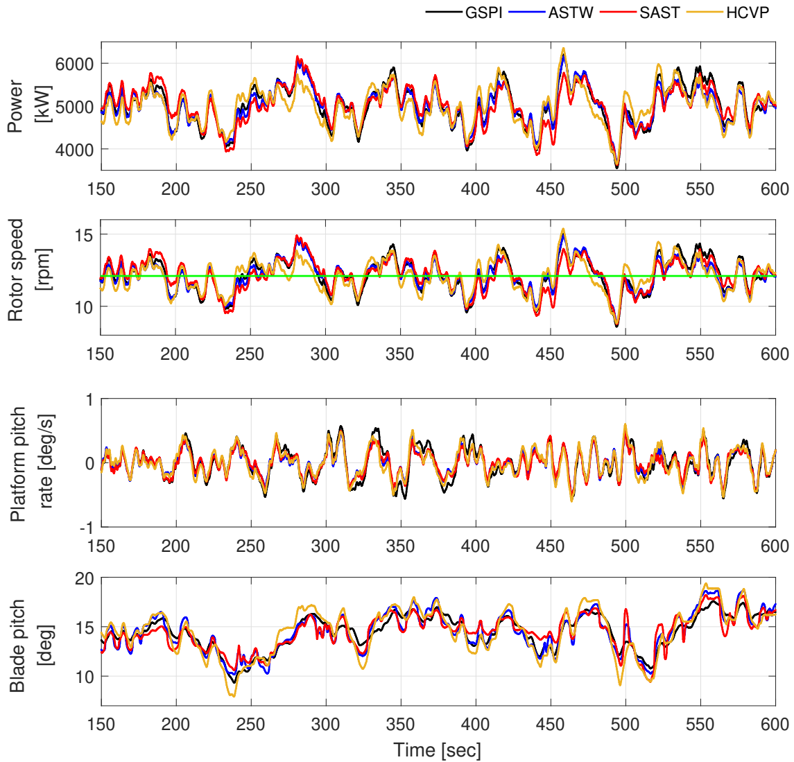
Figure 2.10 – Scenario 3 . Main variables of the FWT versus time ( sec ) respectively, obtained by GSPI (black), ASTW (blue), SAST (red) and HCVP (yellow). The green line in the second sub-figure indicates the rated rotor speed \Omega_{r0} (12.1 rpm ).
