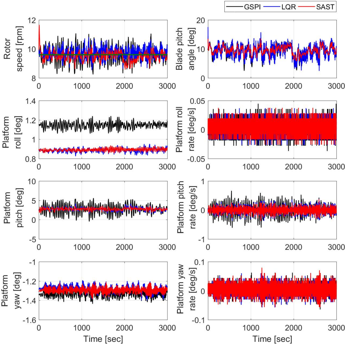
Figure 5.7 – Scenario 2. Measured variables of the experimental set-up versus time ( sec ), obtained by GSPI (black), LQR (blue) and SAST (red). The green line in the first sub-figure indicates the rated rotor speed ( 9.6 rpm ).
