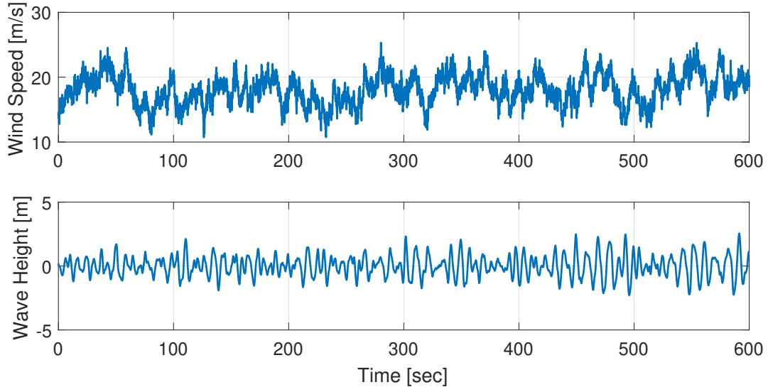
Figure 3.2 – Wind speed ( top ) and wave height ( bottom ) versus time ( sec. ).
