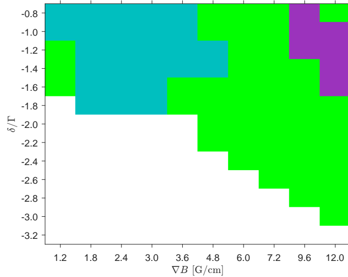
Figure 2.19: \delta - \nabla B phase-space colormap diagram that is drawn according to the instability criteria seen in the text. The following color code is used for the unstable clouds: blue, green and purple for respectively the case-A, -B and -C clouds. White color is used for stable clouds, determined by the experimental result in Fig. 2.10. Note that this diagram is used in drawing the instability regime boundaries in the \delta - \nabla B phase-space diagram seen in Fig. 2.20.
