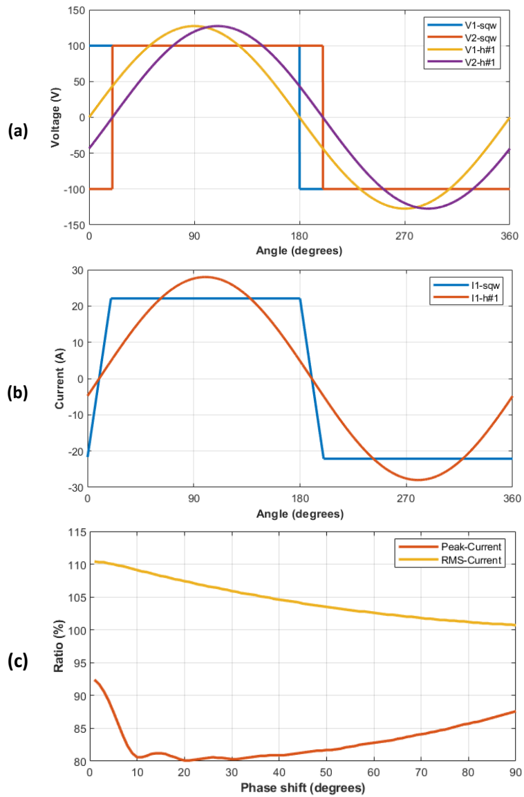
Figure 2.13: Comparison between results of first harmonic approximation and square-wave analysis: (a) Voltages and (b) Currents for phase shift of 20 degrees; (c) Variation of the ratio of square-wave to 1 st harmonic parameters including power, peak current and effective current for phase shift of zero to 90 degrees.
