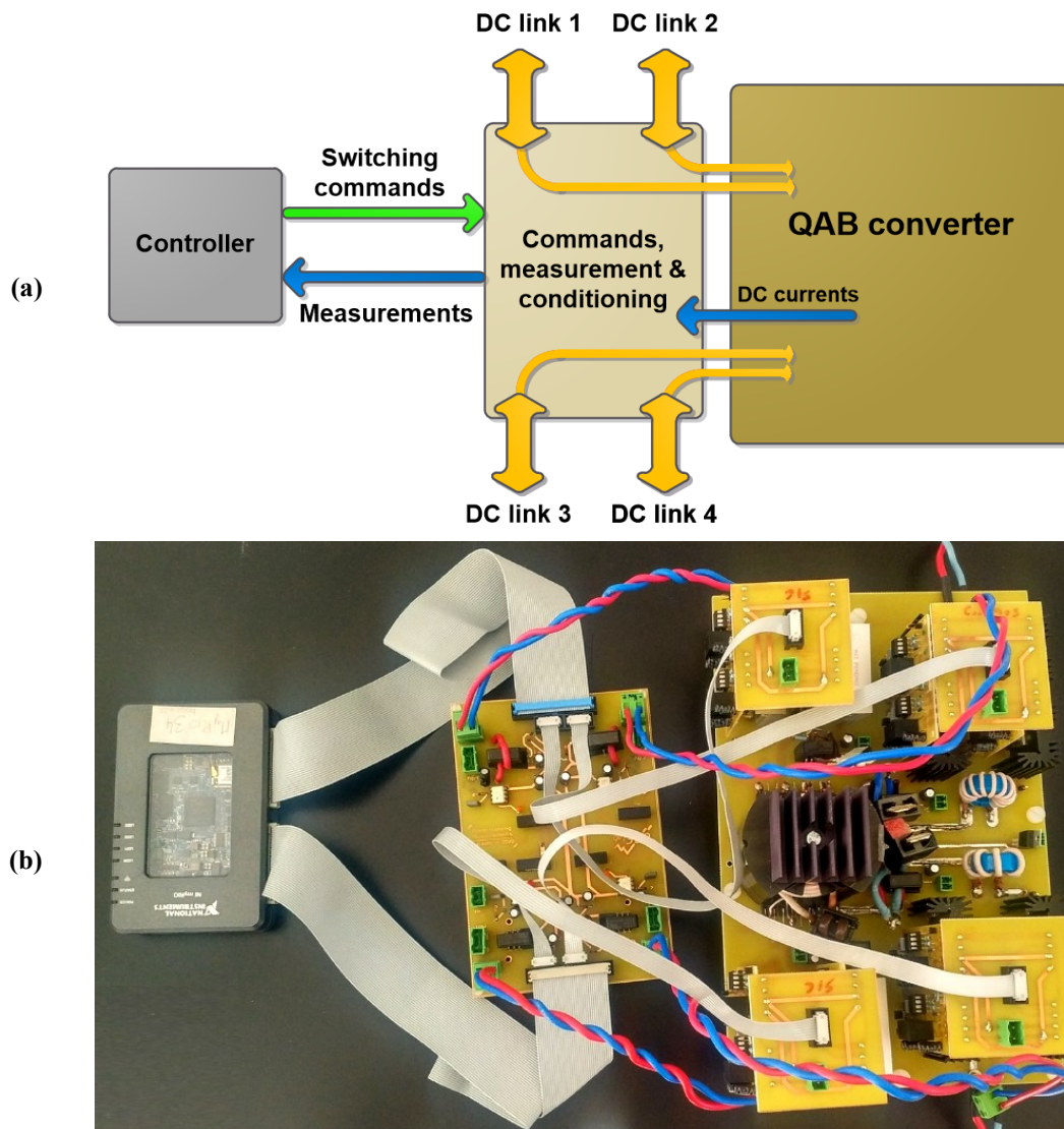
Figure 4.6: The test setup: (a) the schematics; and (b) the real test setup, including the QAB converter, the measurement and conditioning board and the controller. The yellow arrows in (a) indicate power connections, and the rest are command and measurement signals.
