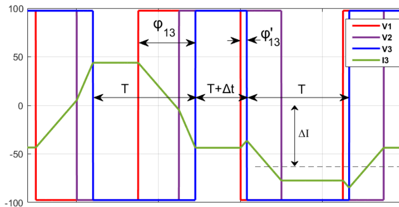
Figure 3.14: A large change in phase shift of port 3 leads to loosing ZVS on this port, as the current is always negative because of the large DC current offset. Since phase shift reduces in this example, \Delta t has a negative value.
