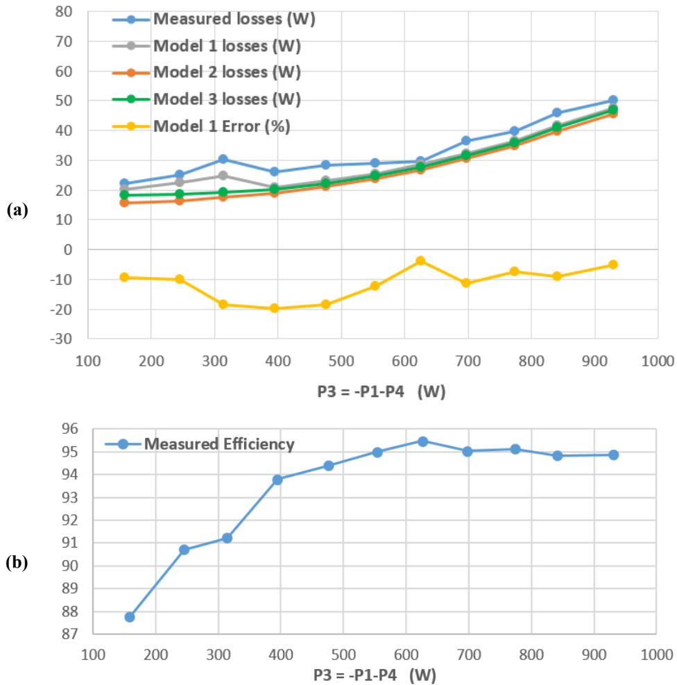
Figure 4.19: (a) Comparing measured losses with predictions of the loss models. (b) Evolution of efficiency as the powers increase. Port 1 and port 4 are the sources of energy and equally feed port 3. Power transfer of port 2 is kept close to zero.
