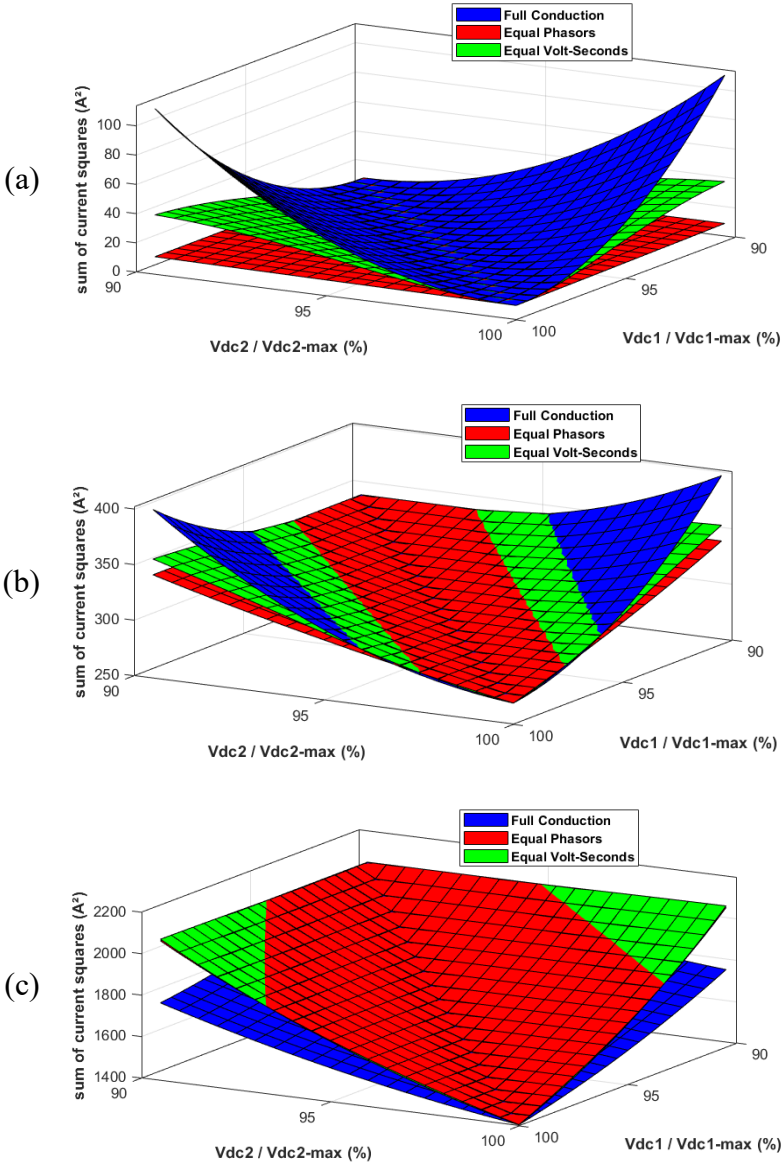
Figure 2.22: Comparing sum of current squares in different voltage modulations as DC link voltages of a DAB vary from their nominal value, when transferring (a) 20%, (b) 50% and (c) 100% nominal power. Sum of current squares is chosen as a parameter that is directly related to conduction losses in the converter.
