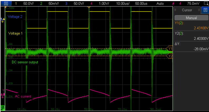
Figure 3.27: Comparing cancellation of AC component of the current in steady state with different CTs: (a) “EFD CT”; and (b) “Tore CT”. Channels 1 and 3 (yellow and blue) indicate the active bridge voltages of the DAB. Channel 2 (green) is the output of the Hall effect sensor. Channel 4 (pink) is the output of a clamp AC current sensor.
