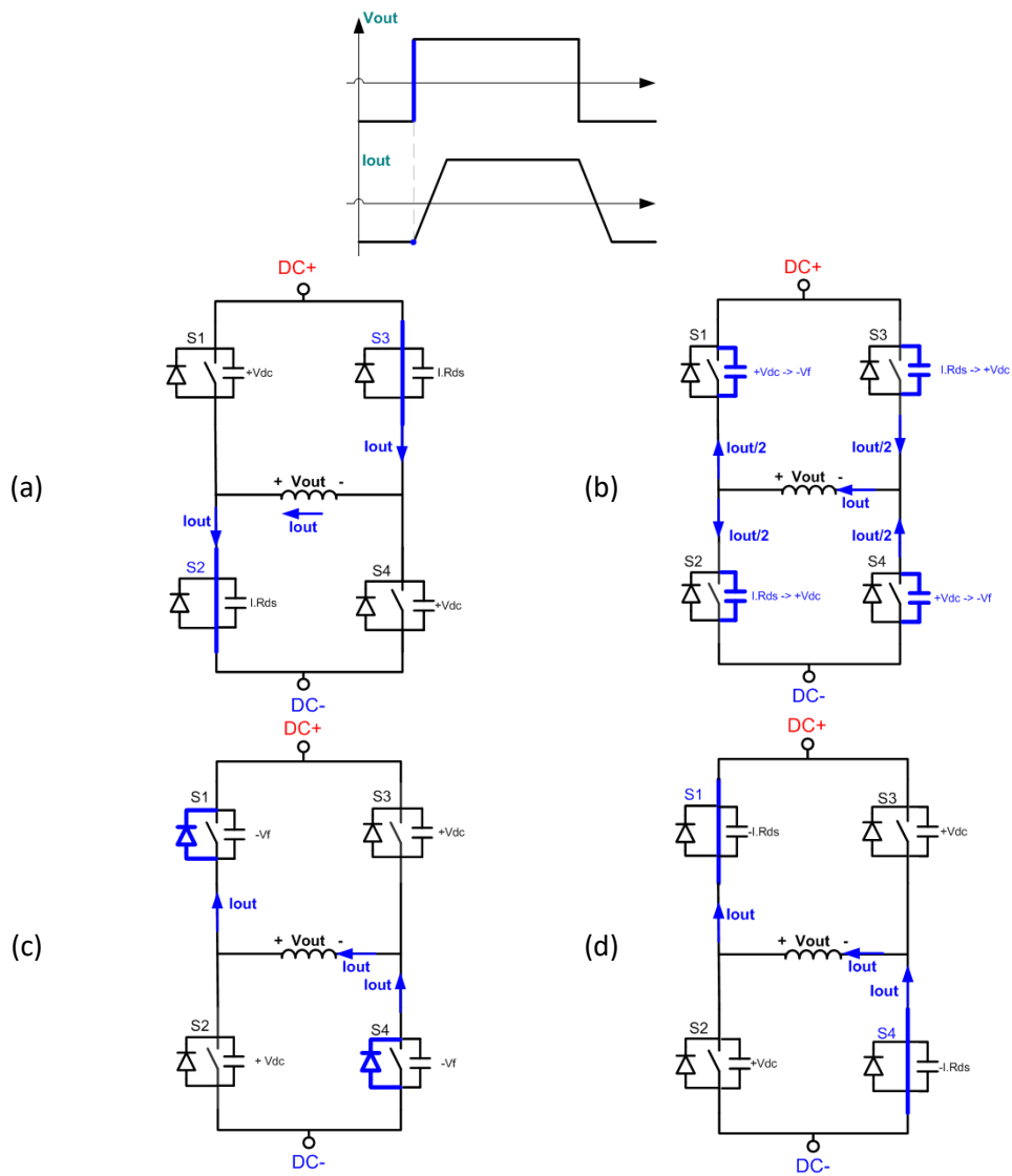
Figure 3.2: Soft switching in an active bridge; the switching process is divided into four steps of a, b, c and d.
