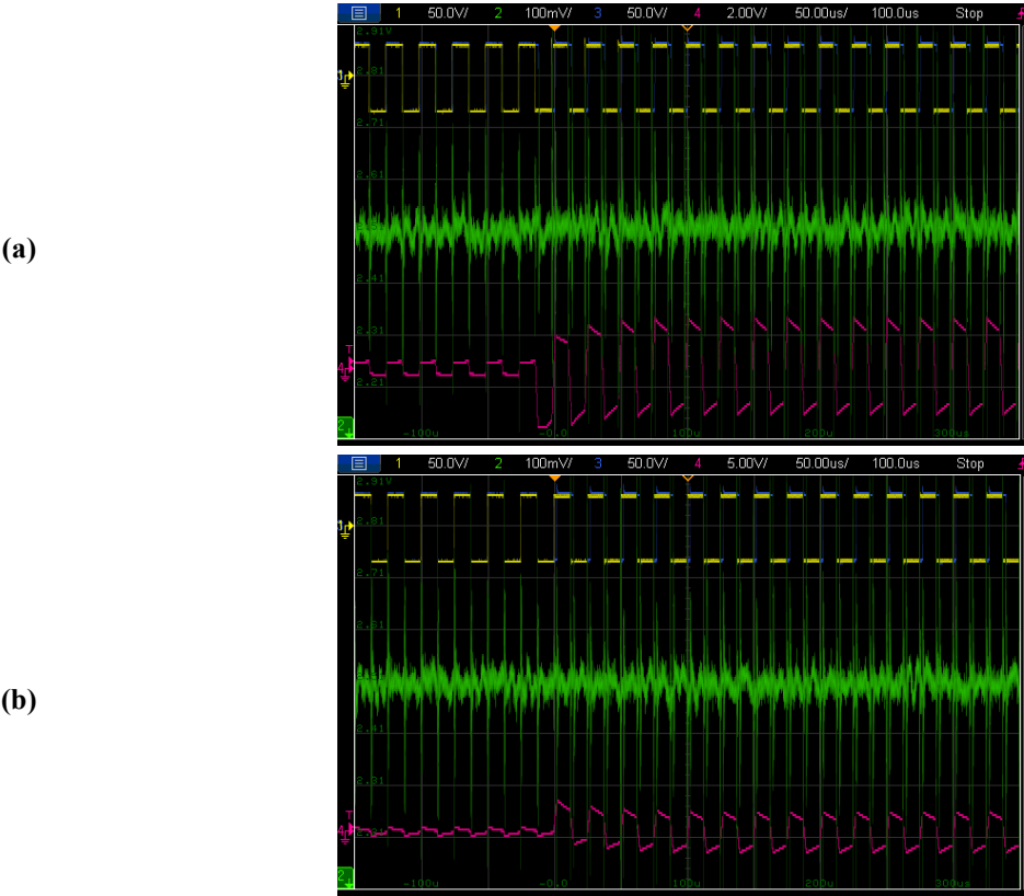
Figure 3.28: Comparing cancellation of AC component of the current during a power transient with different CTs: (a) “EFD CT”; and (b) “Tore CT”. Channels 1 and 3 (yellow and blue) indicate the active bridge voltages of the DAB. Channel 2 (green) is the output of the Hall effect sensor. Channel 4 (pink) is the output of a clamp AC current sensor.
