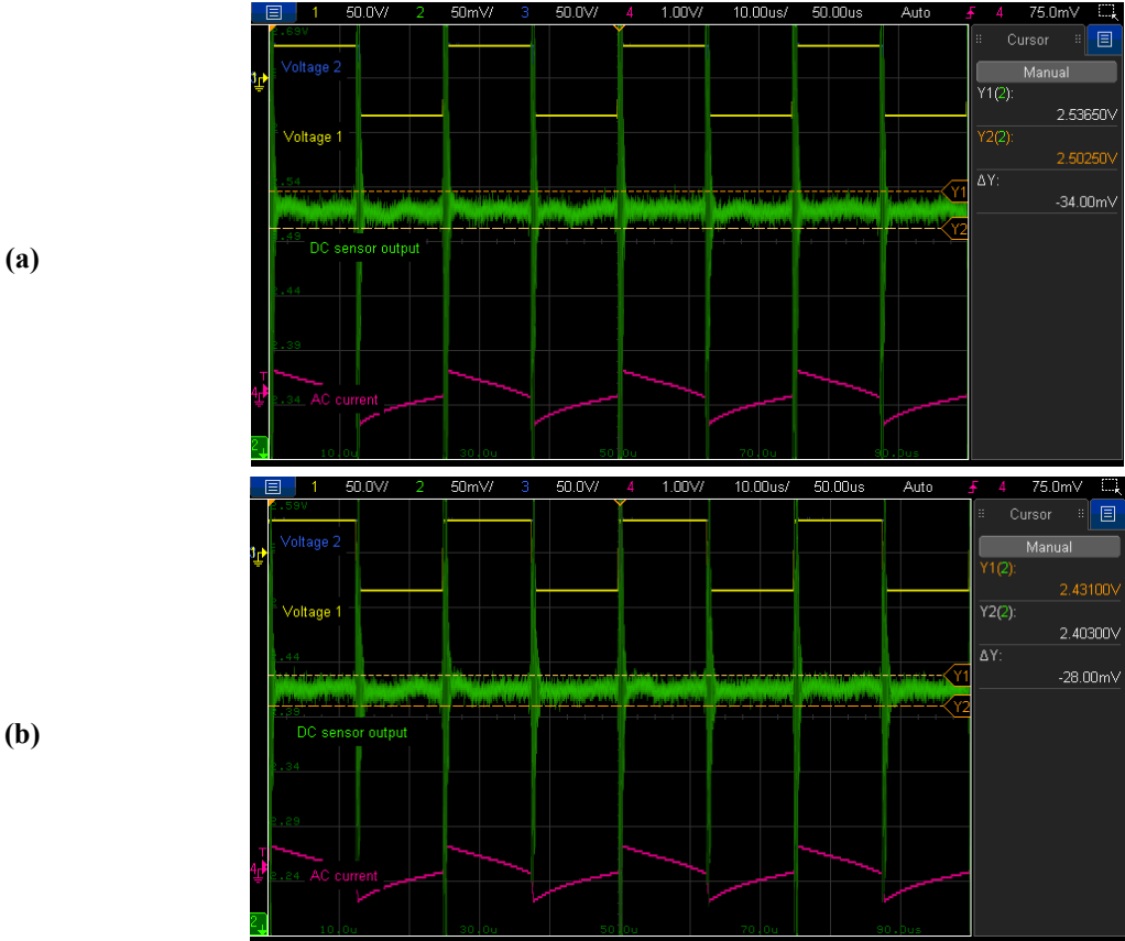
Figure 3.27: Comparing cancellation of AC component of the current in steady state with different CTs: (a) “EFD CT”; and (b) “Tore CT”. Channels 1 and 3 (yellow and blue) indicate the active bridge voltages of the DAB. Channel 2 (green) is the output of the Hall effect sensor. Channel 4 (pink) is the output of a clamp AC current sensor.
