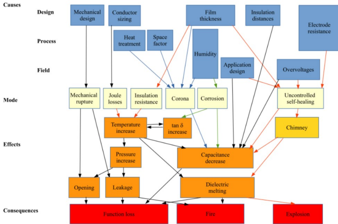
Figure 2.5: Failure modes of metalized film capacitors with their causes and consequences [64].
