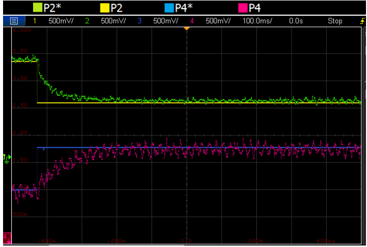
Figure 4.12: Closed loop results of the same test as Figure 4.11. The control system is composed of a PI feedback loop alone.
