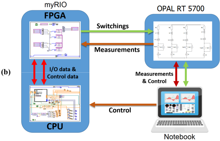
Figure 4.9: Real-time simulation setup with OPAL RT 5700 simulator.
