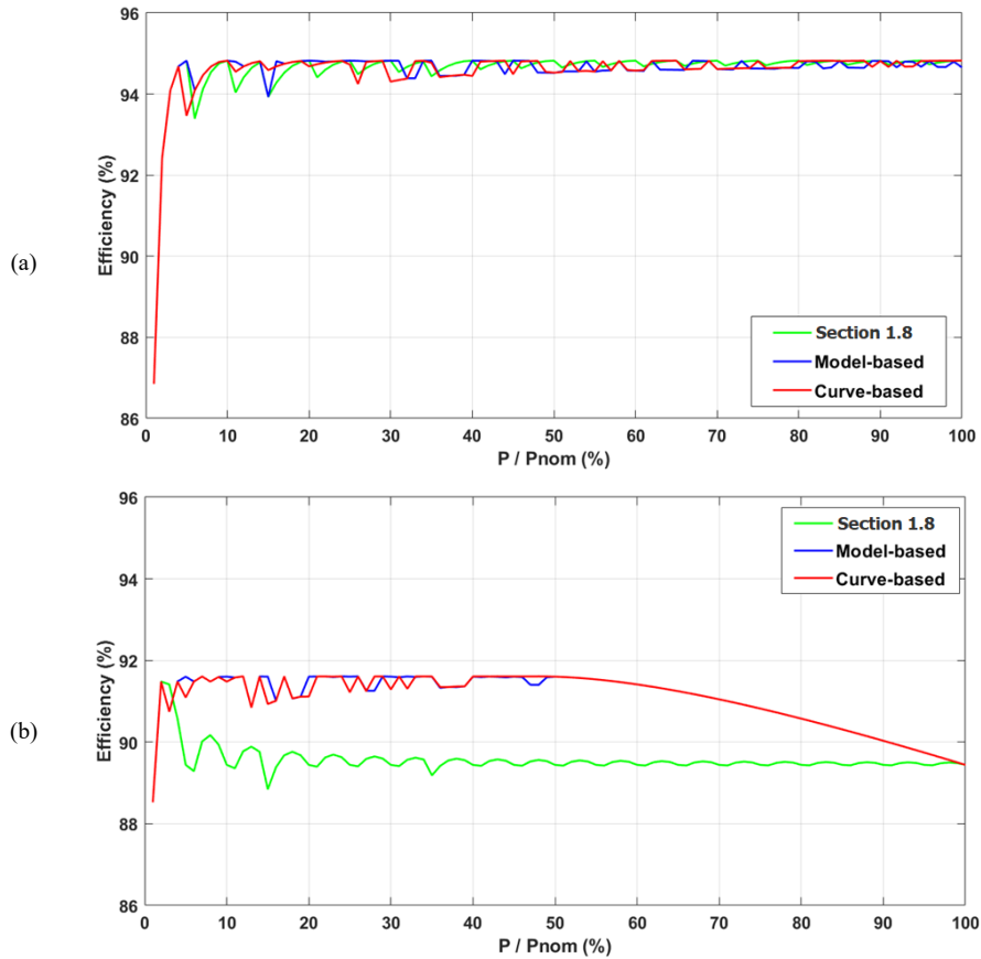
Figure 1.16: Comparing efficiency of different methods over full power range for: (a) design A, and (b) design B.
