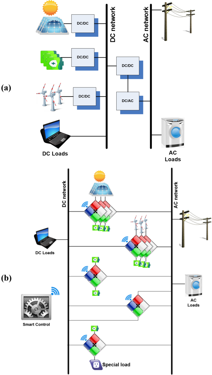
Figure 3: (a) An example of a classic microgrid structure; (b) The proposed cluster of converters.
