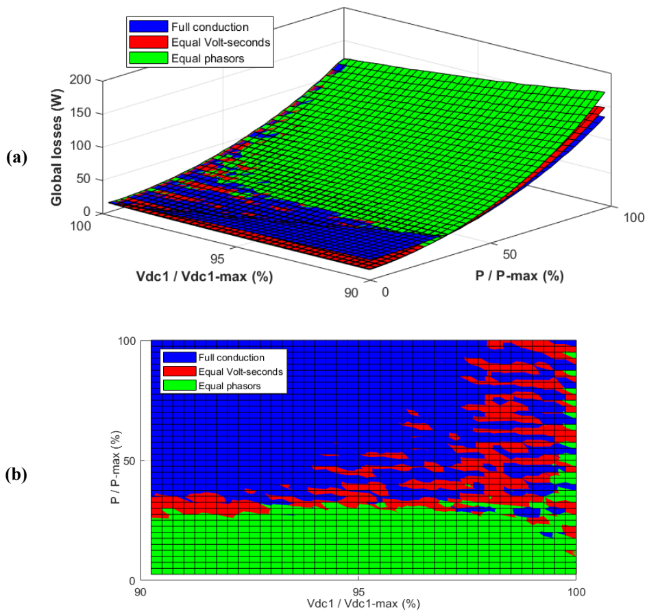
Figure 3.34: Comparison of total losses due to different voltage modulations in a QAB as the DC link voltage of the first port and the power transfer change. (a) shows the 3D view; (b) is the bottom view, indicating the modulation with smallest losses.
