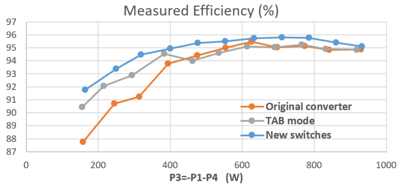
Figure 4.20: Comparing efficiency of different test in scenario 4.
