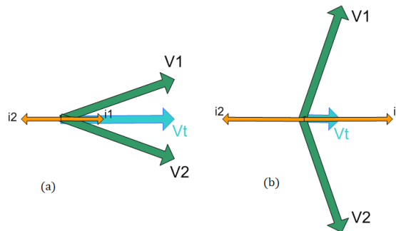
Figure 2.25: The two possible solutions for a certain real power transfer in a DAB with the same voltage magnitudes, but different transformer voltages and phase shifts: (a) with the plus sign in Equation (2.45); and (b) with the negative sign in Equation (2.45).
