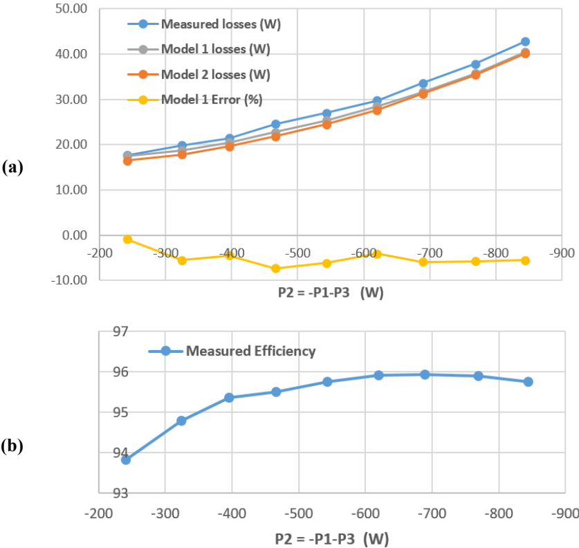
Figure 4.16: (a) Comparing measured losses with predictions of the loss models. (b) Evolution of efficiency as the powers increase. Port 2 is the source of energy and feeds port 1 and port 3 equally. Power transfer of port 4 is kept close to zero.
