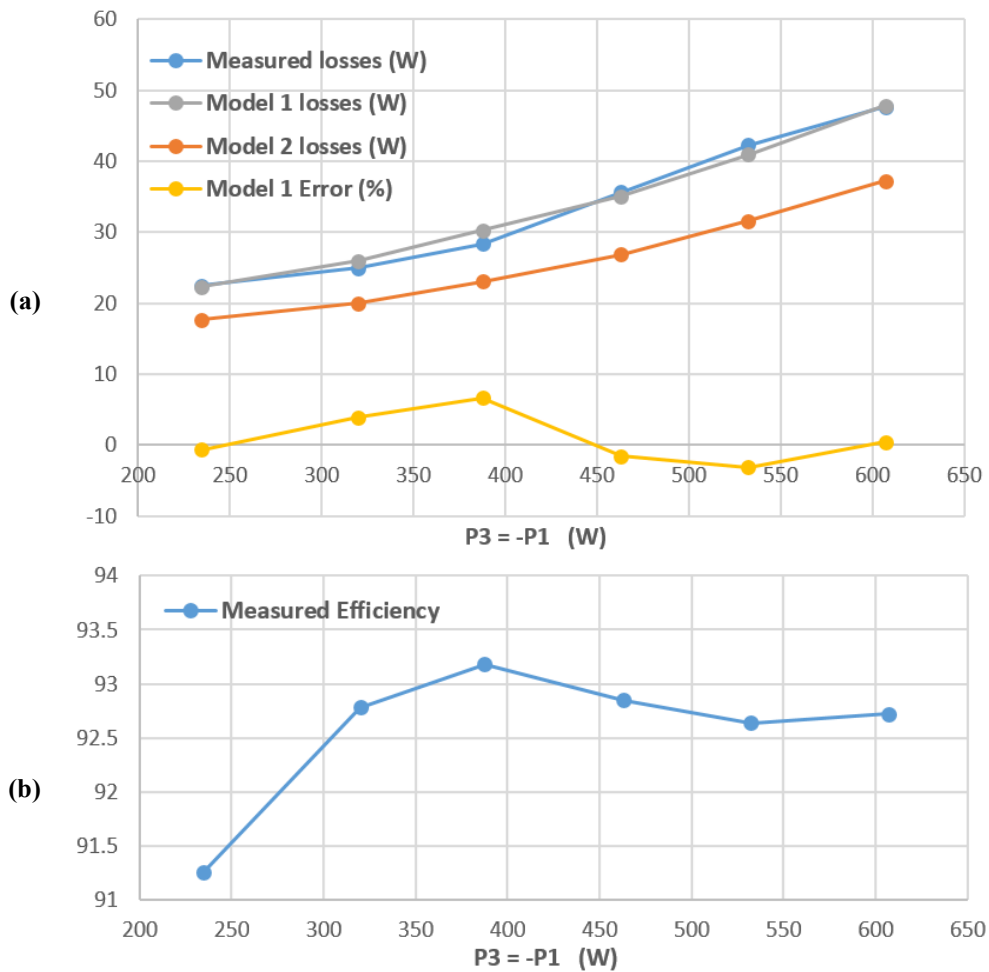
Figure 4.18: (a) Comparing measured losses with predictions of the loss models. (b) Evolution of efficiency as the powers increase. Port 1 is the source of energy and feed port 3. Power transfers of port 2 and port 4 are kept close to zero.
