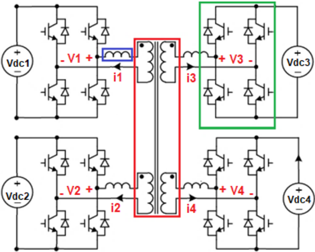
Figure 2.1: A QAB converter: the green box shows an active bridge; the red box is a multi-winding transformer; the blue box is an inductor, which can be either an external one or the leakage inductance of the transformer.
