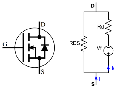
Figure 3.1: Current sharing between channel and body diode of a mosfet during reverse conduction
