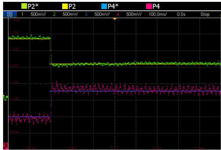
Figure 4.13: Closed loop results of the same test as Figure 4.11. The control system has both PI feedback and matrix feedforward loops activated.
