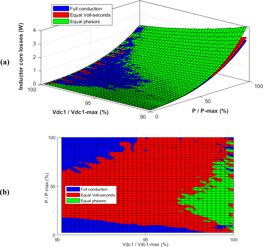
Figure 3.31: Comparing losses in magnetic cores of the inductors of a QAB with different voltage modulations. (a) shows the 3D view; (b) is the bottom view, indicating the modulation with smallest losses.
