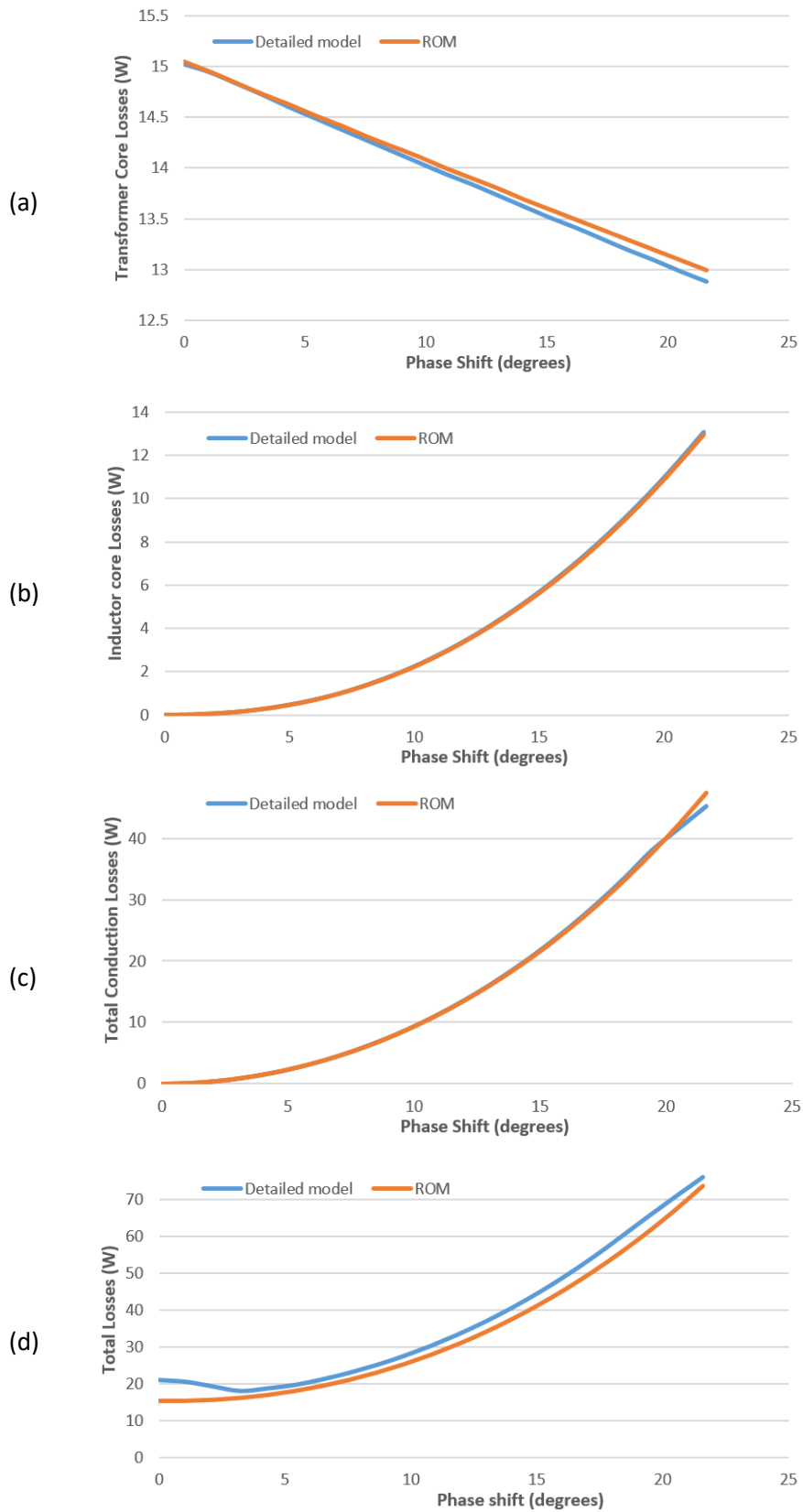
Figure 3.11: Comparing predictions of the ROM and the detailed model of losses in a QAB: (a) transformer core losses; (b) total inductor core losses; (c) total conduction losses; and (d) total losses when there is 5% voltage variation on one port.
