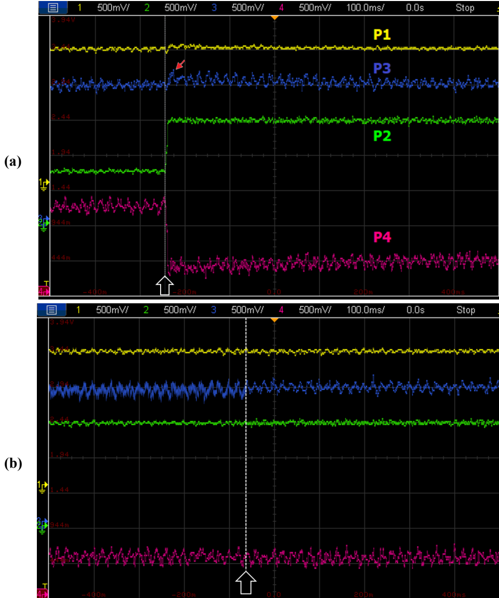
Figure 4.21: Performance of the converter if the ports with zero power transfer are disconnected: (a) automatically, by the control system; and (b) manually, after their power is set to zero. In this test P2 drops to zero and is disconnected at the moment indicated by the white dotted line.
