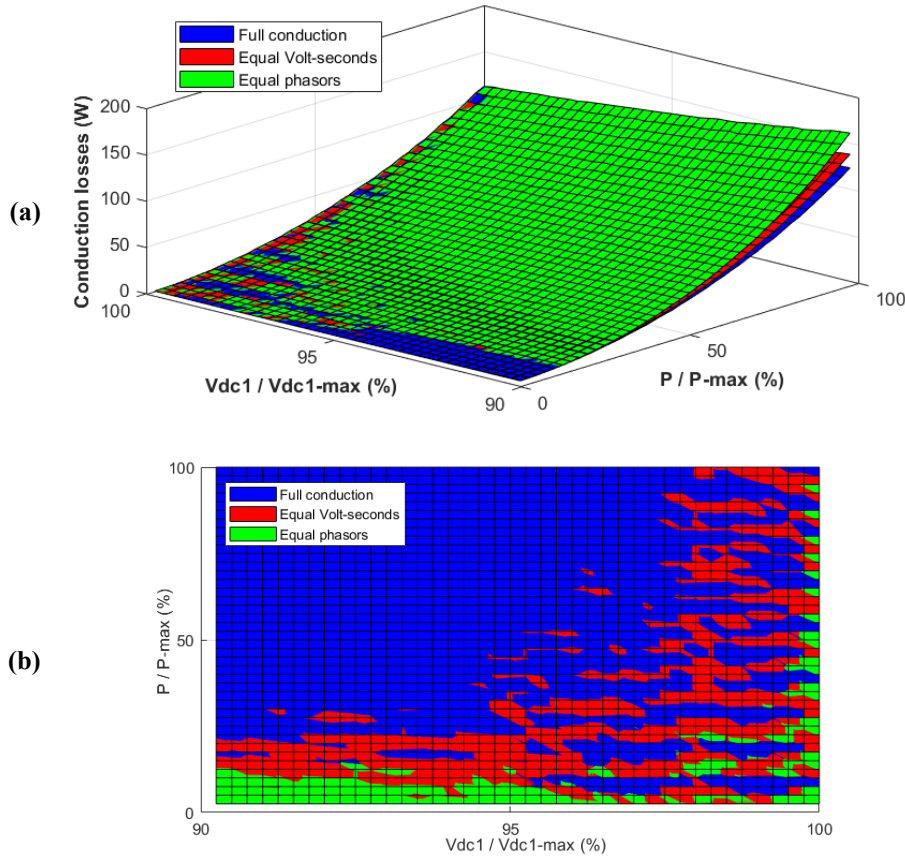
Figure 3.30: Comparing conduction losses when DC link voltage of the first port changes between 90% and 100% nominal voltage, and the power transfer of all ports increase from 0 to 100% nominal power. The rest of DC link voltage are constant at their nominal value. (a) shows the 3D view; (b) is the bottom view, indicating the modulation with smallest losses.
