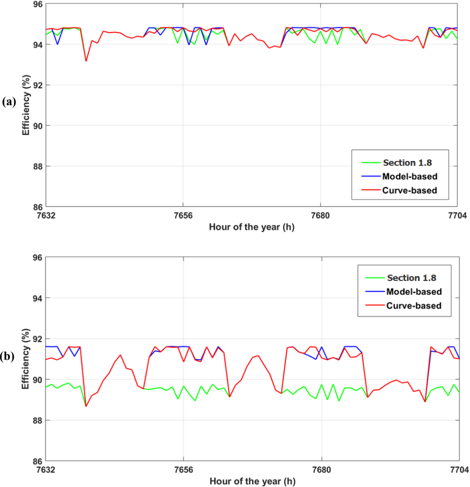
Figure 1.17: Efficiency over three consecutive days for (a) converter design A; and (b) converter design B.
