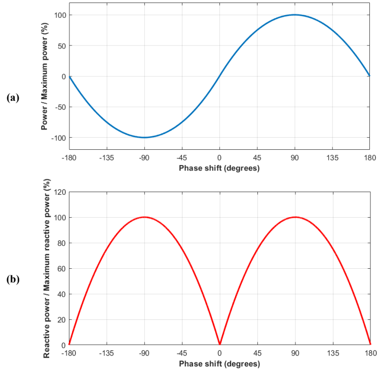
Figure 2.11: (a) Active and (b) reactive power transfer in a DAB as a function of phase shift.
