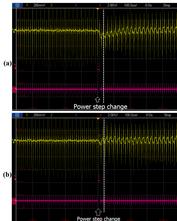
Figure 4.22: Performance of DC current cancellation during power transients. (a) Formation of DC current during power transient when cancellation is off; and (b) Preventing formation of DC current when the cancellation control is on. The yellow curve shows output of the DC current sensor setup. The white dotted line indicates the change in power flow and hence the phase shift, activating the two-step phase shift control to avoid formation of a DC current.
