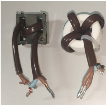
Figure 3.25: Different types of CT that were tested in the proposed DC current measurement setup: EFD core on the left and toroid core on the right.
