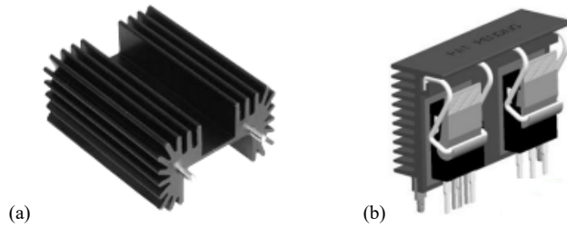
Figure 4.3: Heat sinks: (a) RA-T2X-38E heat sink for each switch of port 1 and port 2; and (b) OMNI-UNI-18-50 heat sink for each arm of port 3 and port 4.
