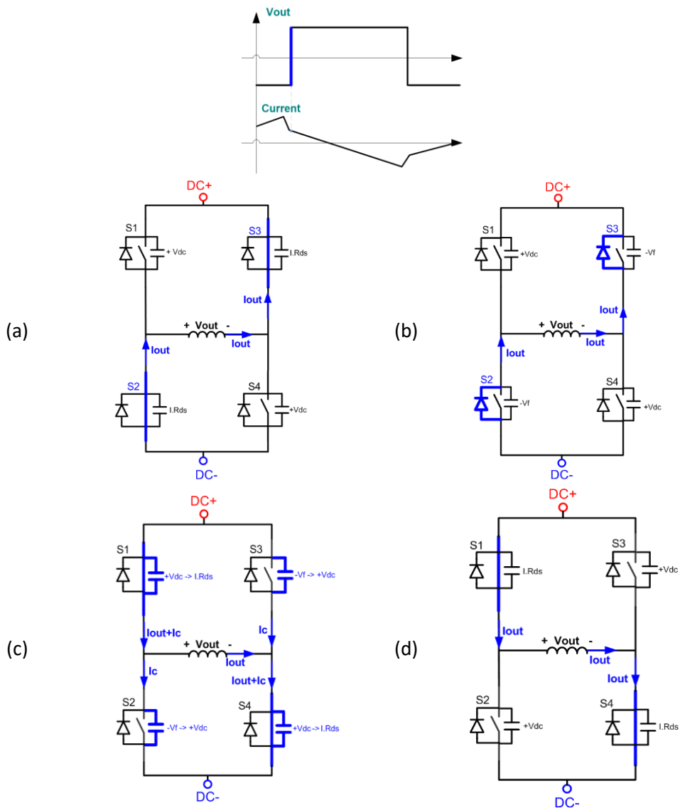
Figure 3.4: Hard switching in an active bridge; the switching process is divided into four steps of a, b, c and d.
