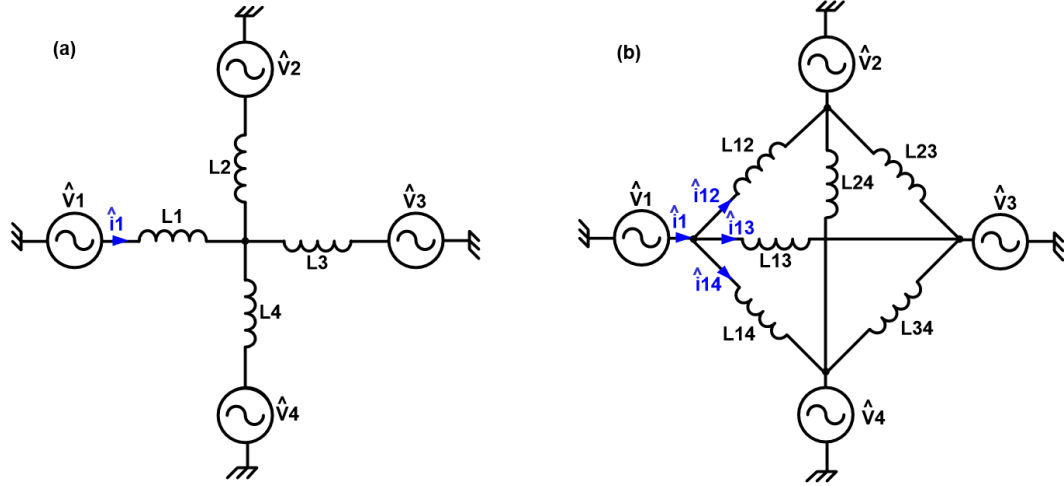
Figure 2.14: (a) First harmonic model of a QAB converter; (b) The first harmonic model of a QAB after applying star-to-delta transform on the network of inductances.
