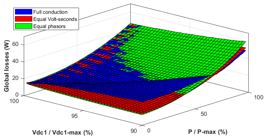
Figure 3.35: Comparison of total losses due to different voltage modulations in a QAB as the DC link voltage of the first port and the power transfer change. The axis representing P/Pmax shows the power transfer of the third and the fourth port, while the first and the second ports do not exchange any real power.
