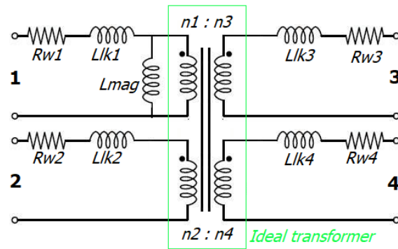
Figure 4.5: The T model of the transformer. R_w and L_{lk} indicate winding resistances and leakage inductances of each port, respectively. The magnetizing inductance of the core is marked as L_{mag} .
