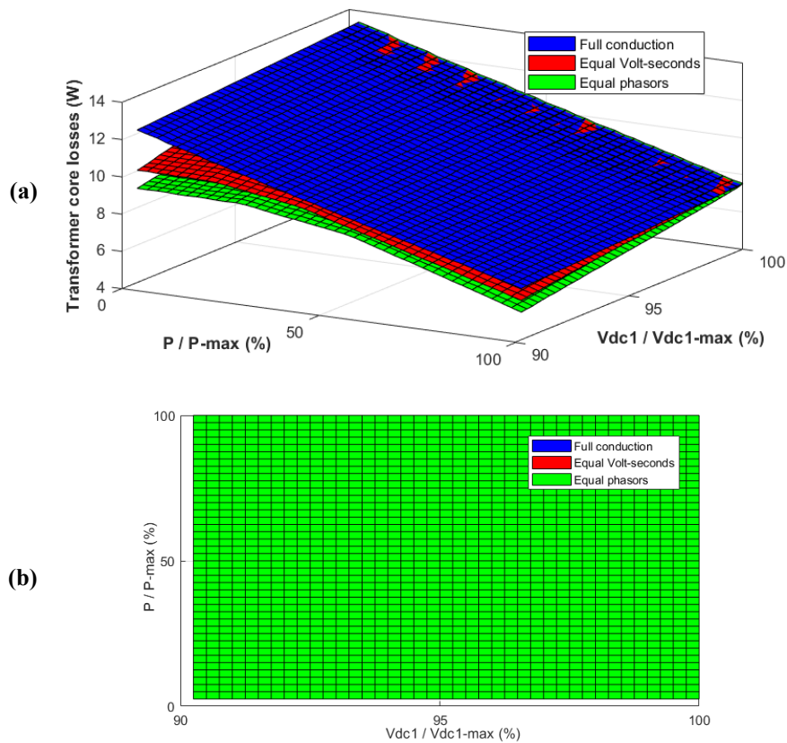
Figure 3.32: Comparing losses in magnetic core of the transformer of a QAB with different voltage modulations. (a) shows the 3D view; (b) is the bottom view, indicating the modulation with smallest losses.
