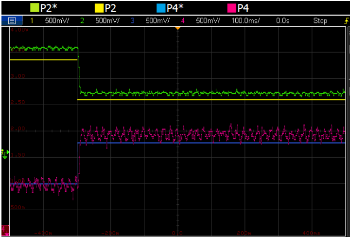
Figure 4.11: Open loop results of a step change in reference powers. The reference values (P2* and p4*) are shown along with their corresponding measured values (P2 and P4).
