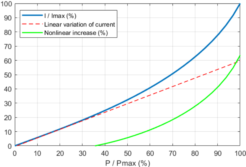
Figure 2.15: Nonlinear increase in current of an active-bridge in a QAB, as the power transfer of the corresponding port gets close to its maximum value. The dotted line displays an imaginary linear increase, to indicate the extent of the nonlinear increase in current.
