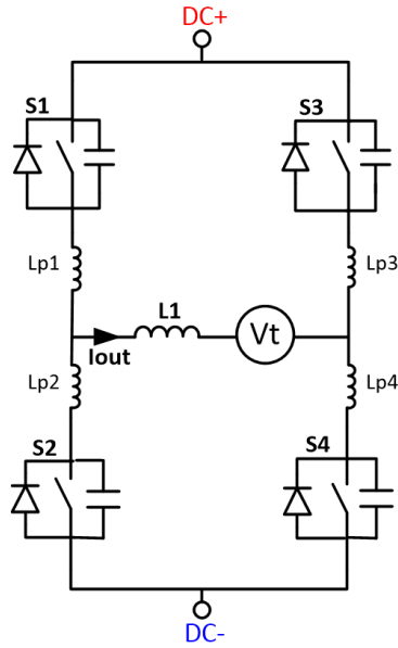
Figure 3.15: An active bridge with its parasitic inductances in series with each switch. V_t is the voltage across transformer windings.
