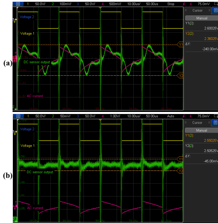
Figure 3.22: Evaluation cancellation of AC component of the current in steady state: (a) no AC cancellation; (b) with AC cancellation. Channels 1 and 3 (yellow and blue) indicate the active bridge voltages of the DAB. Channel 2 (green) is the output of the Hall effect sensor. Channel 4 (pink) is the output of a clamp AC current sensor.
