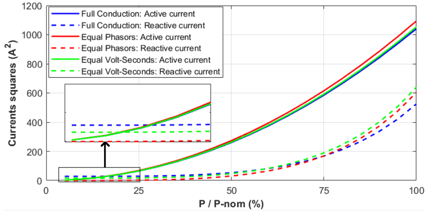
Figure 2.23: Comparing active and reactive currents of a DAB in different voltage modulations. DC link voltages of the primary and secondary are equal to 95% and 100% nominal voltage, respectively.
