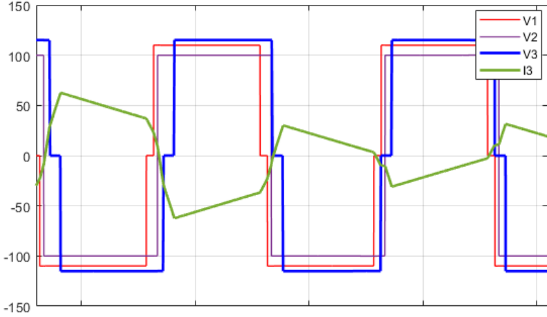
Figure 3.17: Performance of the two-step phase-shift change in a case with arbitrary DC link voltages and duty cycles.
