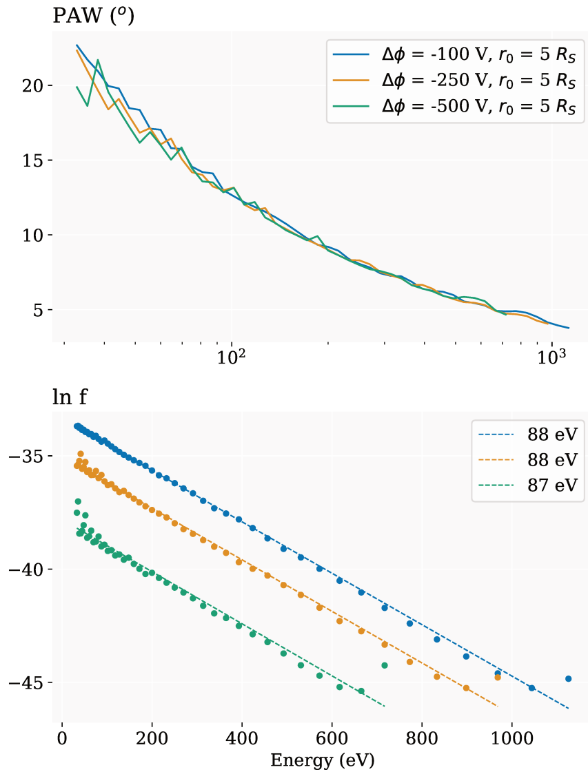
Figure 4: PAW (upper plot), and parallel slice through the VDF ( f_{\parallel} , lower plot) with respect to electron energy, resulting from the simple collisionless focusing model at the distance of 35 R_S . Different colours correspond to the examples with different \Delta\phi . The dashed line in the lower plot represents a 1D Maxwellian fit to f_{\parallel} , giving the T_{s,\parallel} marked in the legend.
