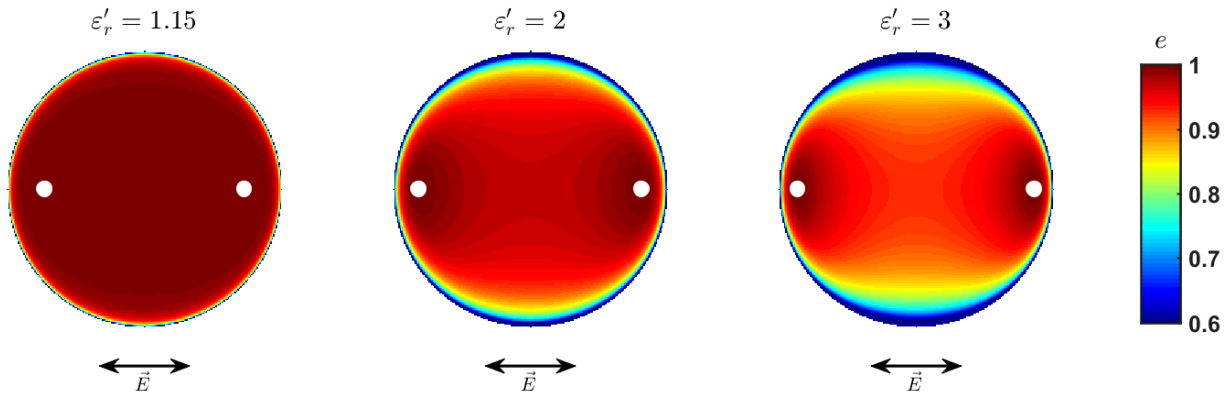
Figure 2.12 – Emissivity maps given by Fresnel’s equations for an ideal smooth, uniform, dielectric, spherical surface, for dielectric constants of \epsilon'_r = 1.15 , 2, and 3. The direction of the electric field sensed by the antenna \vec{E} is indicated. Polarization parallel to \vec{E} is therefore left–right, whereas perpendicular polarization is top–bottom. The Brewster highlights peak at the Brewster angles \theta_B , which are marked with a black dot.
