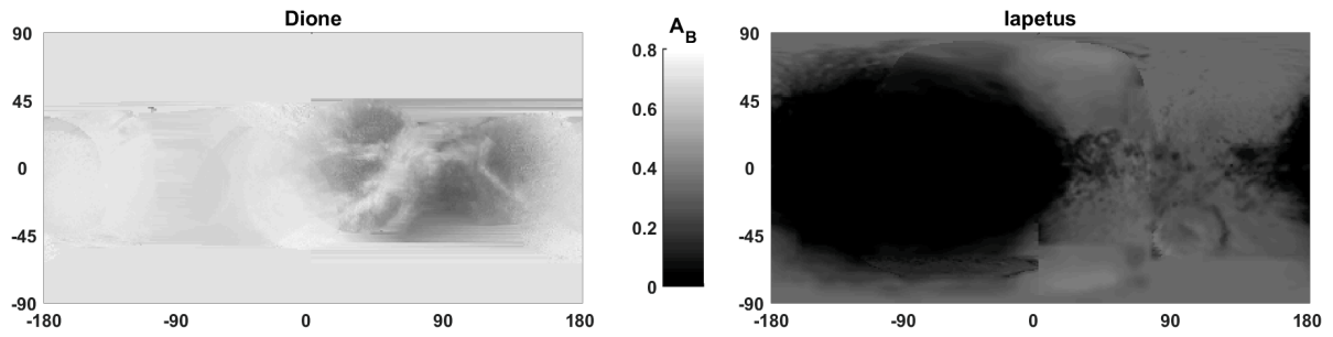
Figure 5.3 – Bolometric Bond albedo maps of Dione (adapted from Blackburn et al., 2012) and Iapetus (Blackburn et al., 2011).
