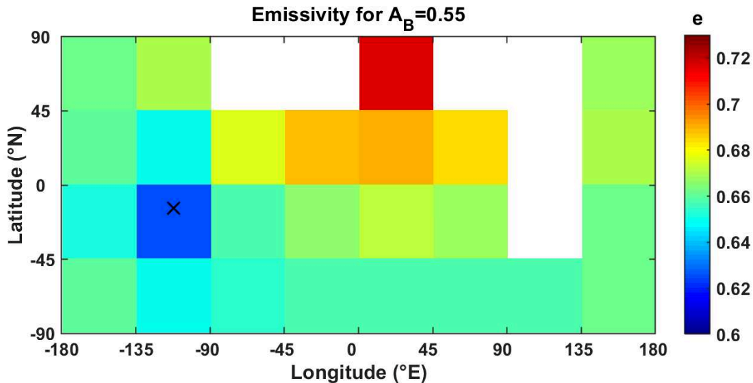
Figure 6.19 – Same as Fig. 6.14, except Saturn’s contribution to the incoming flux is now accounted for in the model. Note that, while the sub-Saturn anomaly remains, its amplitude is decreased.
