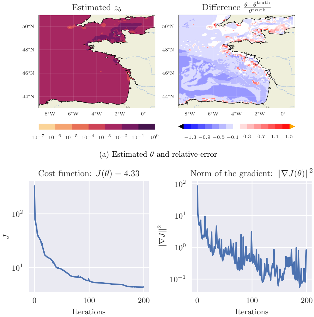
(b) Objective function evolution along the iterations
