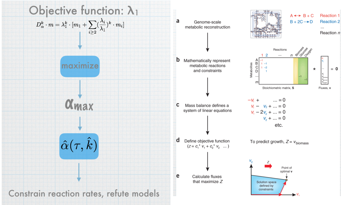
Figure 8.2: Flux Balance Analysis versus “Synchronous Balanced Analysis” (Right: Flux Balance Analysis ) A workflow for FBA, as taken from [142]. When applied to growth maximization, the biomass objective function is defined by adding an artificial “biomass” reaction into the reaction network, the flux of which is set to be equal to the exponential growth rate \lambda . Thus, growth optimization using FBA is achieved by maximizing the flux of this “biomass reaction”. (Left: “ Synchronous Balance Analysis ”) For BRNs comprised exclusively of unimolecular reactions, our Petri net execution semantics enables the mathematical characterization of the system’s growth rate, which in turn avoids any artificial addition to the model: maximizing the growth rate becomes akin to finding the matrix D_\alpha with the maximal biggest eigenvalue. Our method can also be used to constrain reaction rates and/or refute models, based on their parameter values.
