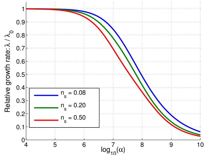
Figure 7.5: The model is simulated for increasing storage capacities \alpha , for three different environments ( n_s = 0.08, 0.20 and 0.5 ). We denote by \lambda_0 the growth rate obtained when the storage capacity is \alpha = 1 , for any given n_s . The relative growth rate \lambda/\lambda_0 is defined as the growth rate obtained for a given storage capacity \alpha , relative to the growth rate when \alpha = 1 . One observes that the relative growth rate decreases, as the storage capacity \alpha increases. The faster a cell grows, the more storage is detrimental to growth.
