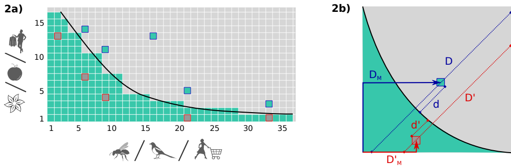
Figure 2.3: Distances and continuous approximations for measuring nestedness. Panel a) shows the scheme of a non-perfectly nested network. Green squares depict the interactions and the black curve represents the Isocline of perfect nestedness (IPN) which separates, in an ideally perfect nested matrix, the region where all the nodes are connected from the region with no interactions. The unexpectedly present interactions above the IPN are highlighted in blue, while absent interactions below the IPN are highlighted in red. Panel b) represents the mapping of a matrix into the unit square. The black curve corresponds to the IPN, and unexpectedly present (absent) interactions are highlighted in blue (red). The figure shows two different kind of distances that may be used for measuring nestedness: D , D' , d and d' (traced in dashed lines) are used in the calculation of the temperature, while D_M and D'_M (represented by solid arrows) are used by the nestedness index based on the Manhattan distance (NMD).
