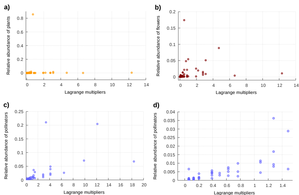
Figure 3.13: Relation among the relative abundance and the Lagrange multipliers for: a) plants, b) flowers and c) pollinators. The d) panel shows the detail of plot c). The Lagrange multipliers are rescaled to the mean. The data correspond to a plant-pollinator network, collected in the un-restored site –also named control site– by Kaiser-Bunbury et al. (2009). As can be seen, in comparison to the restored site, here the plant population is dominated by a superabundant species.
