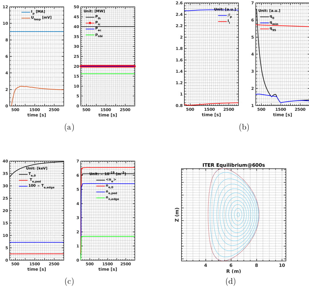
Figure 2.3: Simulation of an H-mode steady-state plasma scenario on ITER. (a) Left: time traces of plasma current and the loop voltage; Right: time traces of the auxiliary heating powers. (b) Left: time traces of plasma poloidal parameter and internal inductance; Right: time traces of the safety factors at typical points. (c) Left: time traces of electron temperatures at typical points; Right: time traces of electron densities at typical points. (d) The ITER magnetic equilibrium and flux surfaces in a poloidal cross-section at 600 s.
