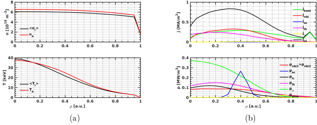
Figure 2.4: The magnetic and kinetic profiles of the reference scenario for H-mode steady-state plasma on ITER at 925.9 s. Left panels: plasma density profiles (top), and plasma temperature profiles (bottom); Right panels: plasma current drive profiles (top), and plasma deposited power profiles (bottom).
