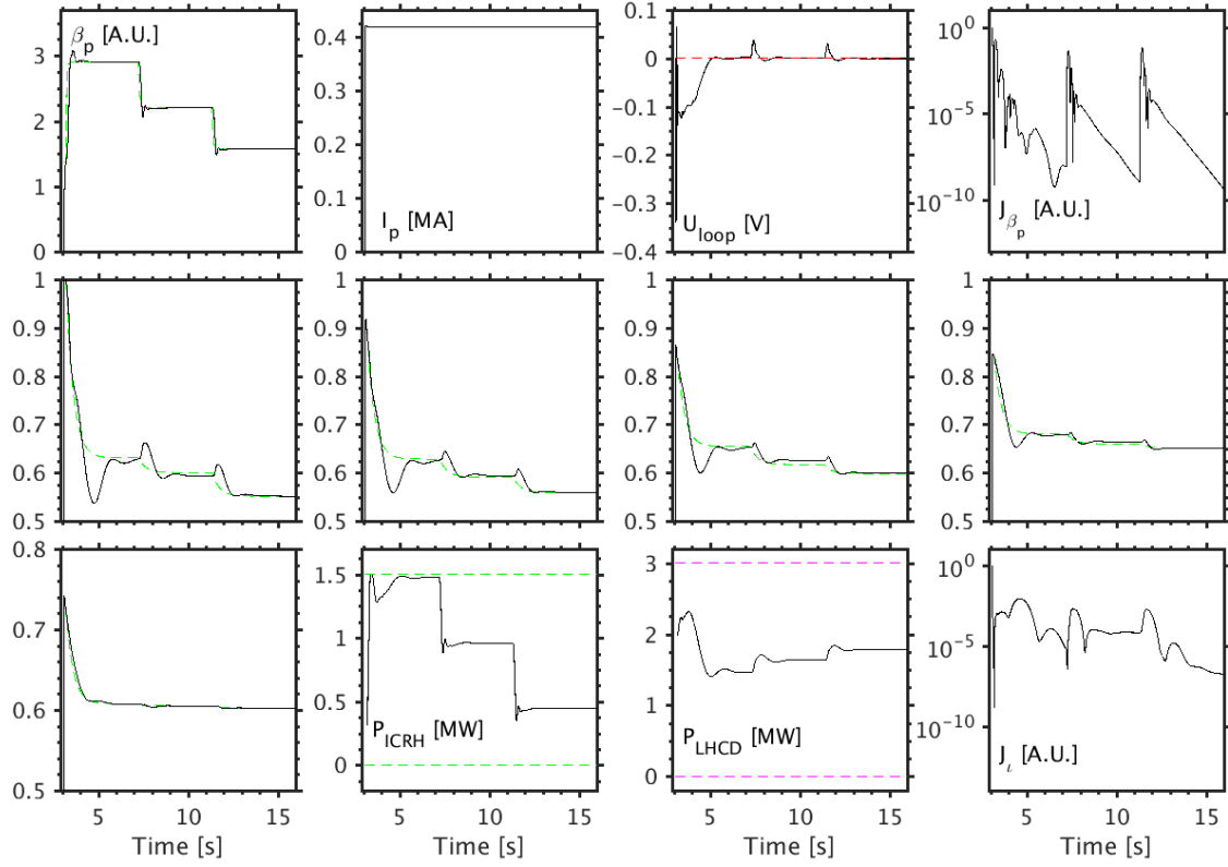
Figure 3.9: Tracking of \iota points at 0, 0.1, 0.2, ..., 0.4 and \beta_p simultaneously. Top panels from left to right: time traces of plasma poloidal pressure \beta_p , plasma current I_p , the loop voltage U_{\text{loop}} (black solid) with the zero loop voltage line (red dashed), the averaged relative error for \beta_p , \langle J_{\beta_p} \rangle . Middle panels from left to right: time traces of the \iota setpoints (green dashed) and evolutions (black solid) at x = 0, 0.1, 0.2, 0.3 . Bottom panels from left to right: time traces of the \iota setpoints (green dashed) and evolutions (black solid) at x = 0.4 , the actuated ICRH power P_{\text{ICRH}} (black solid) associated with its power limits (green dashed), the LHCD power P_{\text{LHCD}} (black solid) associated with its power limits (magenta dashed), and the averaged relative error for \iota , \langle J_{\iota} \rangle .
