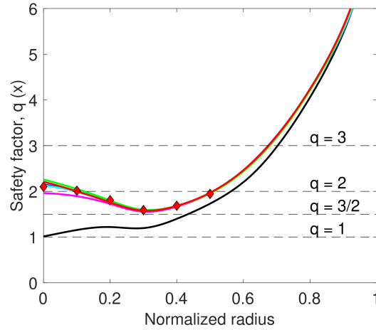
Figure 5.4: Combined distributed q(x) control and slow \beta_p control with LHCD and ICRH. Achieved q(x) at t = 3.2 s (black), 5.1 s (magenta), 7.1 s (blue), 9.1 s (cyan), 9.6 s (green) and 12.5 s (red). These times are shown on Fig. 5.3 by vertical lines. The target q -profile is constant (diamond symbols) and \mu(x) = 1 for 0 \leq x \leq 0.5 . \beta_p control starts at 4.2 s while q(x) control starts at 3.2 s.
