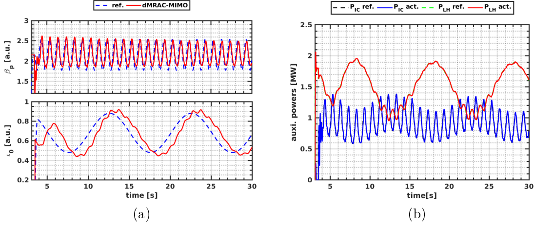
Figure 4.16: Simultaneous tracking of \beta_p and u_0 using the ICRH and LHCD powers. (a) Time traces of the reference trajectories and the achieved values of \beta_p (top) and u_0 (bottom). (b) Time traces of the requested and achieved auxiliary heating and current drive powers.
