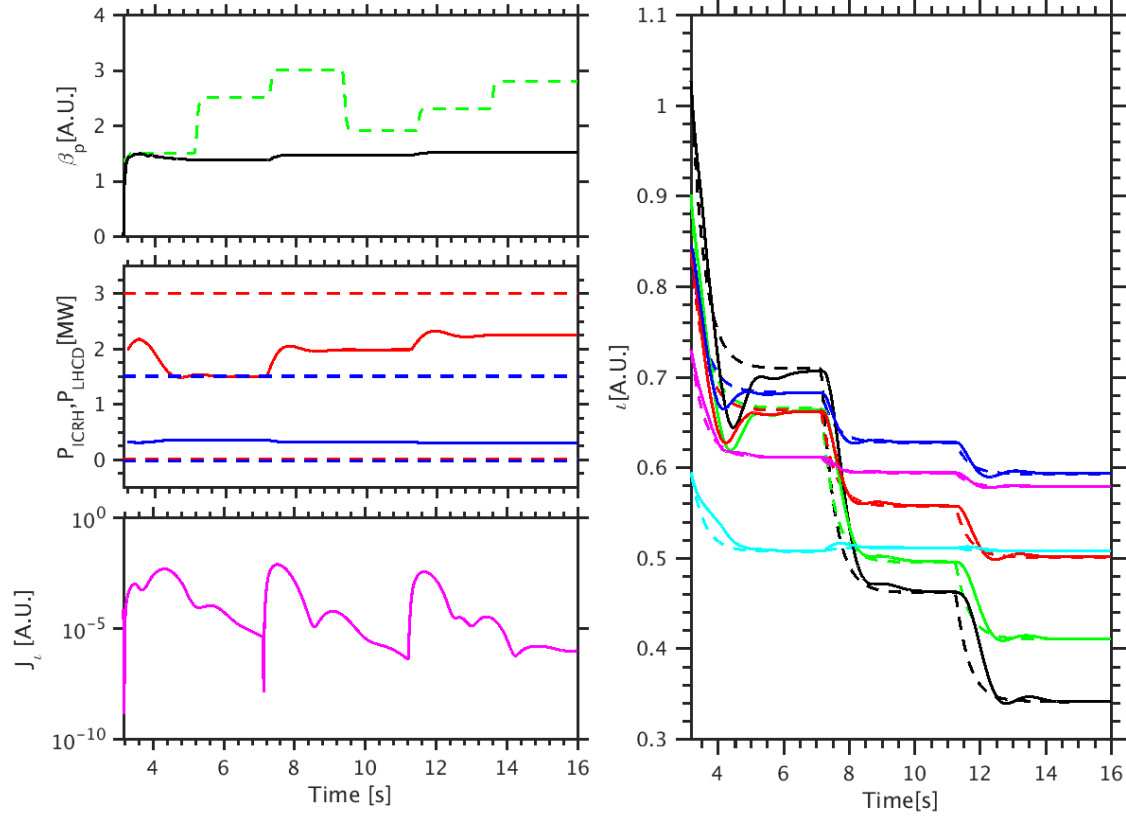
Figure 3.6: Tracking \iota points at 0, 0.1, 0.2, ..., 0.4. Left-top panel: time traces of \beta_p setpoints (green dashed) and evolutions (black) with \beta_p control relaxed. Left-middle panel: time traces of actuated powers P_{ICRH} (blue) and P_{LHCD} (red), as well as the ICRH (blue dashed) and LHCD (red dashed) power limits. Left-bottom panel: time traces of the averaged relative error index for \iota . Right panel: time traces of \iota setpoints (dashed) and evolutions (solid) at x = 0 (black), 0.1 (green), 0.2 (red), 0.3 (blue), 0.4 (magenta), 0.5 (cyan) with \iota feedback control.
