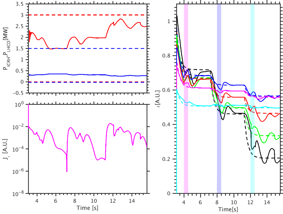
Figure 3.14: Disturbance rejection of \iota control. Left-top panel: time traces of actuated powers P_{\text{ICRH}} (blue) and P_{\text{LHCD}} (red), power ranges of ICRH (blue dash) and LHCD (red dash). Left-bottom panel: time traces of the averaged relative error index for \iota . Right panel: time traces of \iota values (solid) and setpoints (dashed) at x = 0 (black), 0.1 (green), 0.2 (red), 0.3 (blue), 0.4 (magenta), 0.5 (cyan) with \iota feedback control. Magenta, light purple and cyan areas are respectively indicating 30 % increase of \bar{n}_e , H_{98}(y, 2) and Z_{\text{eff}} .
