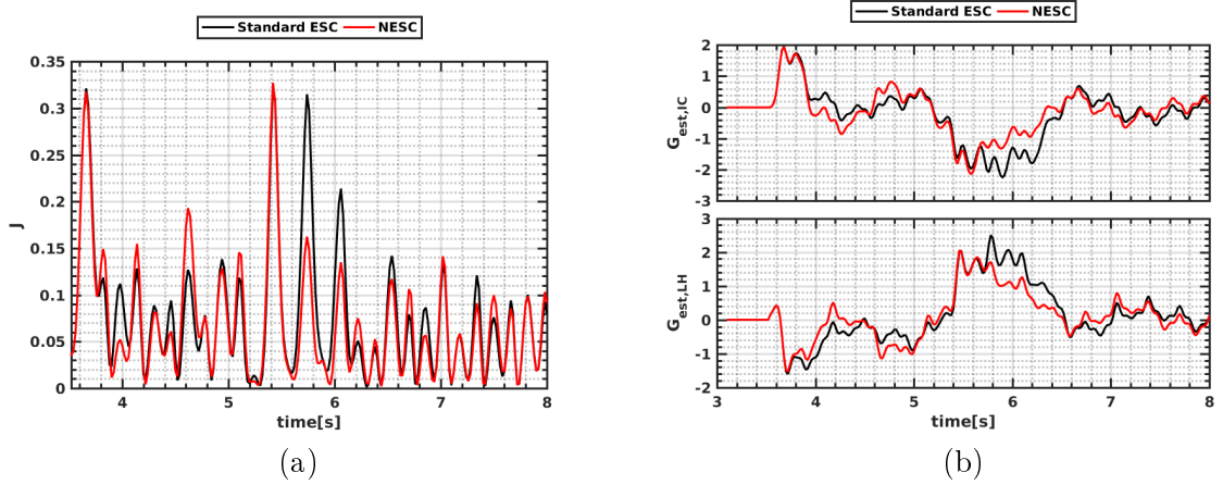
Figure 4.4: Time traces of (a) the performance index and (b) the gradient estimates on EAST.
