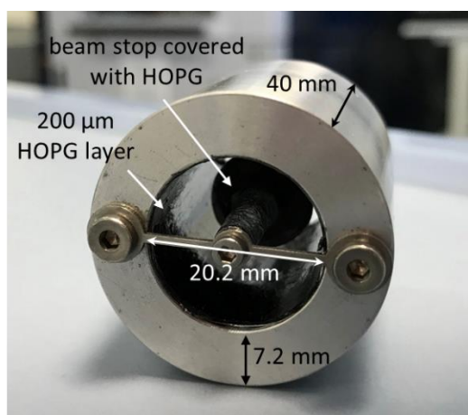
Figure 3.22. HOPG monochromator.
