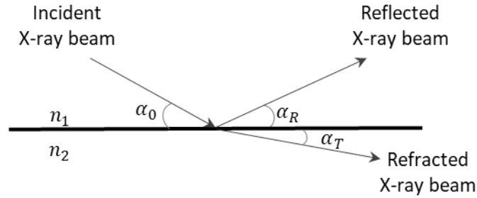
Figure 2.1. Reflection and refraction of an X-ray beam at the interface between two media.
