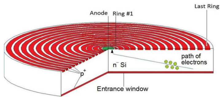
Figure 3.11. Illustration of the SDD design [14].
