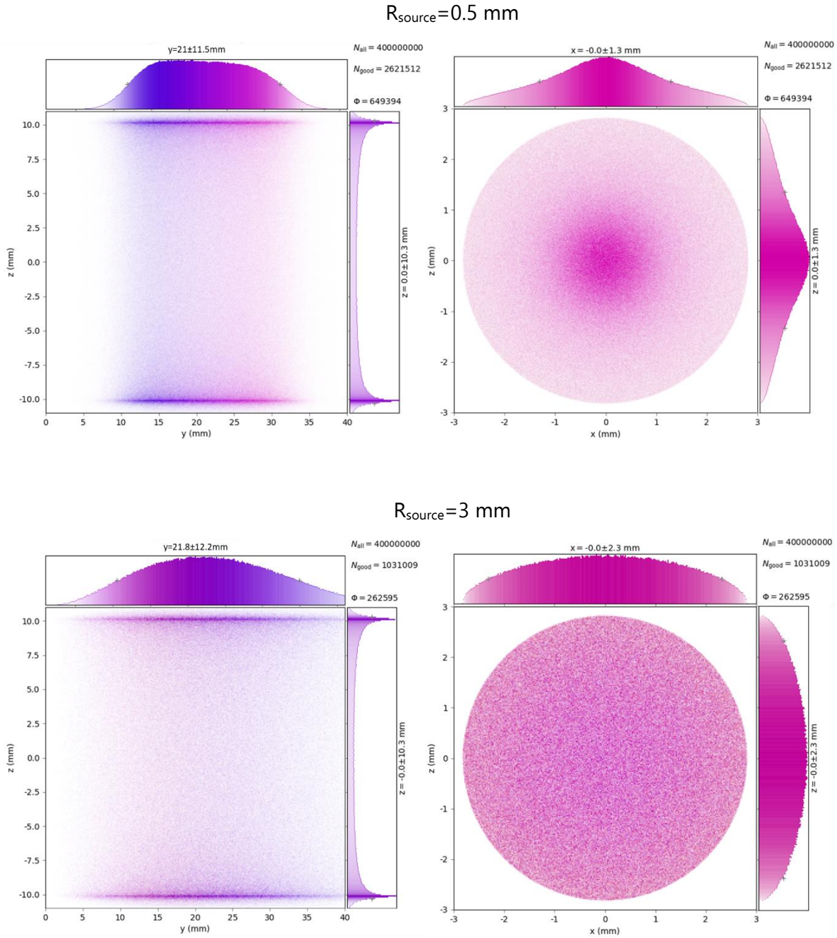
Figure 6.14. Ray footprint of a polychromatic beam on the cylindrical HOPG crystal (left panels) with collection length L=40 \text{ mm} ( Y -axis) and radius R=10.1 \text{ mm} ( Z -axis), and image of the reflected rays intercepted by the image plane (right panels). The radius of the source is 0.5 \text{ mm} (upper panels) and 3 \text{ mm} (lower panels). The distances D_1 and D_2 are equal to 50 \text{ mm} for the central energy of 13 \text{ keV} ( \theta_B = 8.17^\circ ).
