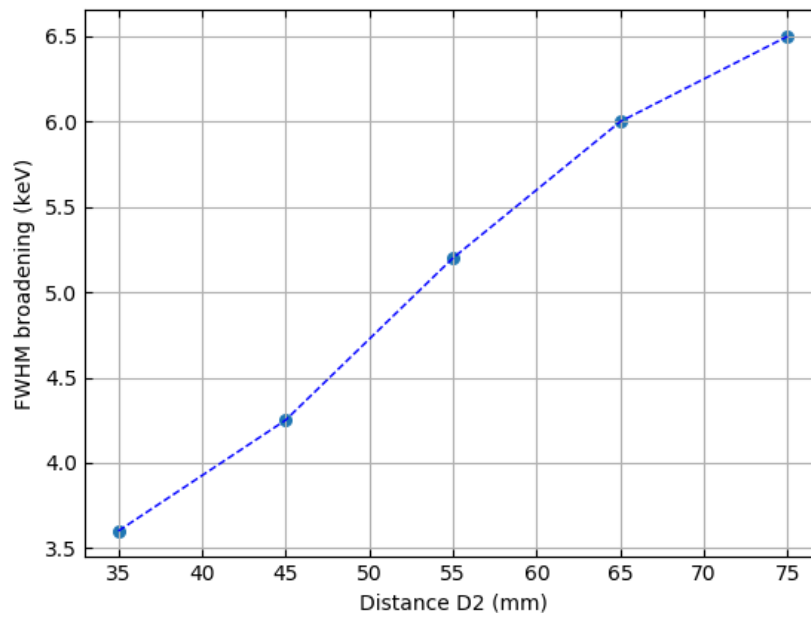
Figure 6.19. Bandwidth broadening at various distances D_2 . The distance D_1=56 mm for the central energy of 14 keV for all calculations.
