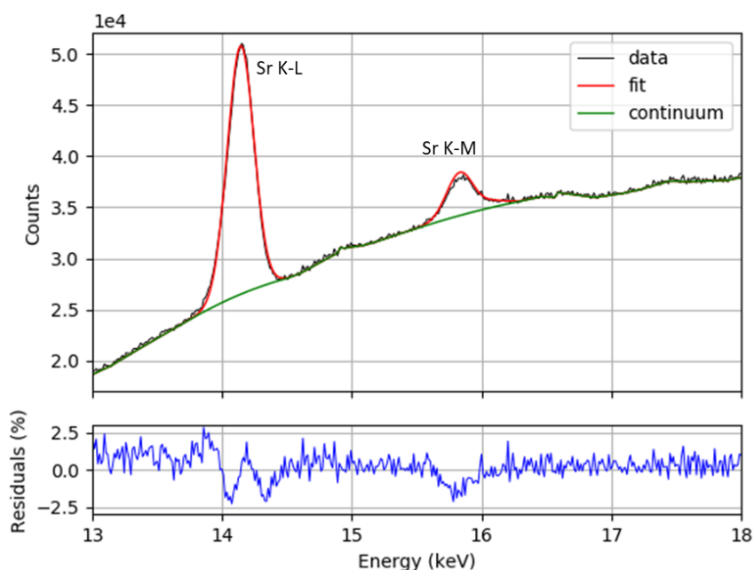
Figure 7.5. Processing of the spectrum of the sample with 100 \text{ mg L}^{-1} of Sr in \text{HNO}_3 0.5 M, collected with the first channel.
