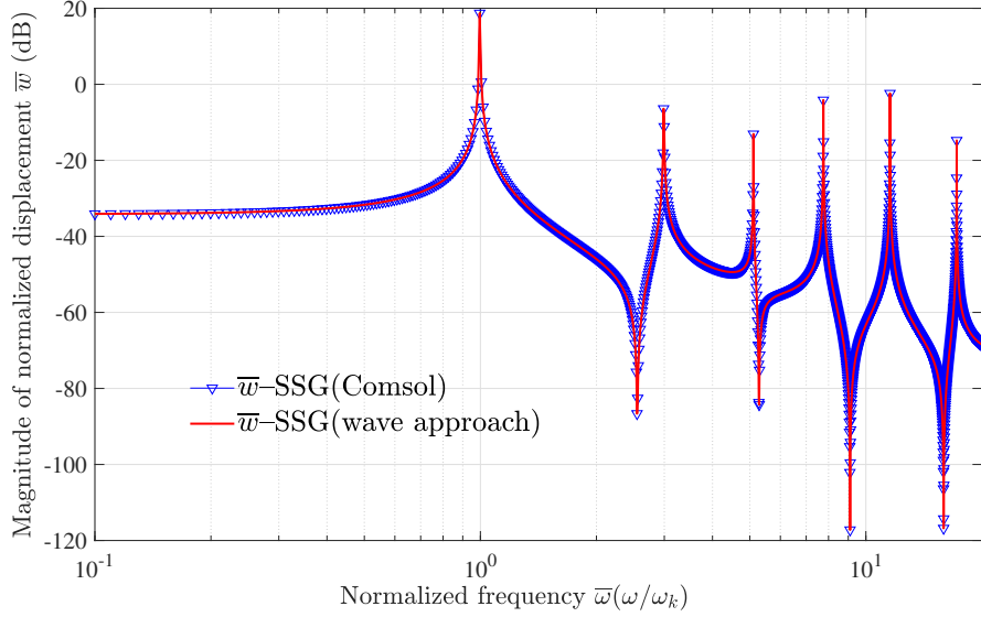
Figure 2.18: Frequency response at x = 0.78L in COMSOL
