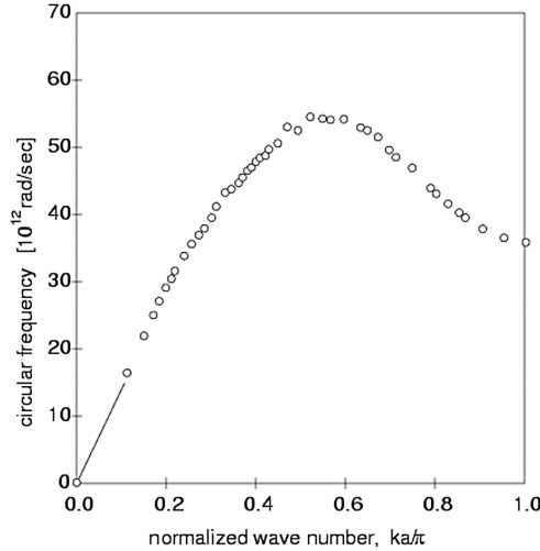
Figure 1.5: Dispersion curve for aluminum
