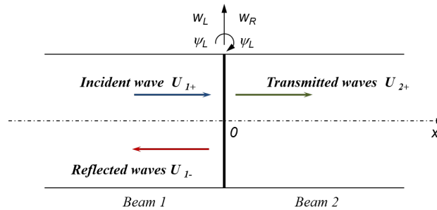
Figure 4.5: Wave reflection and transmission of bending wave
