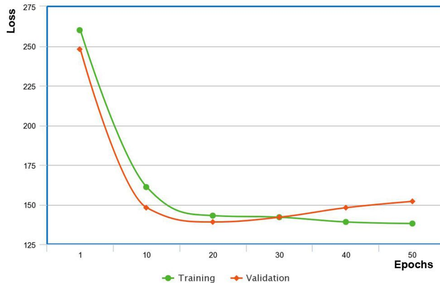
Figure 6.14 – Water Storage Tank Loss Curve 3 hidden layers
