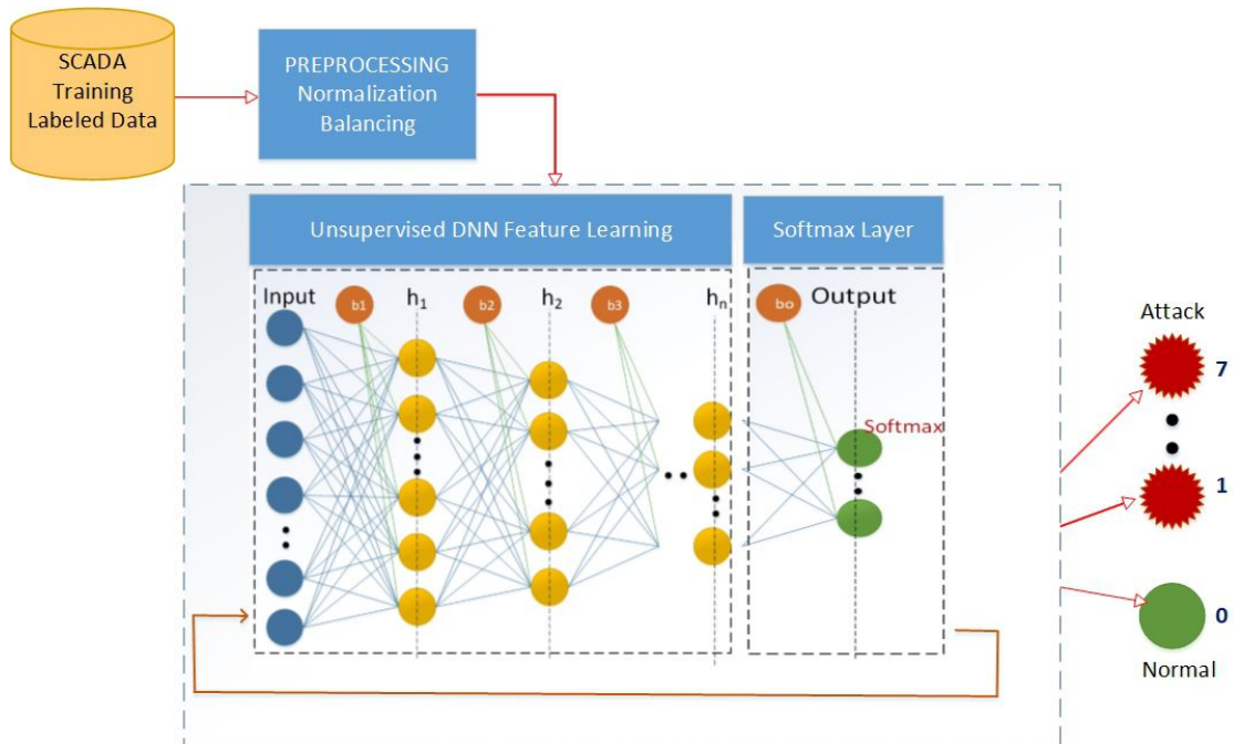
Figure 5.7 – Fine Tuning
