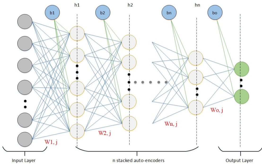
Figure 2.4 – Stacked Auto-encoder
