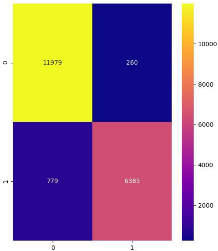
Figure 6.24 – Confusion Matrix Gas Pipeline Dataset Binary Classification
