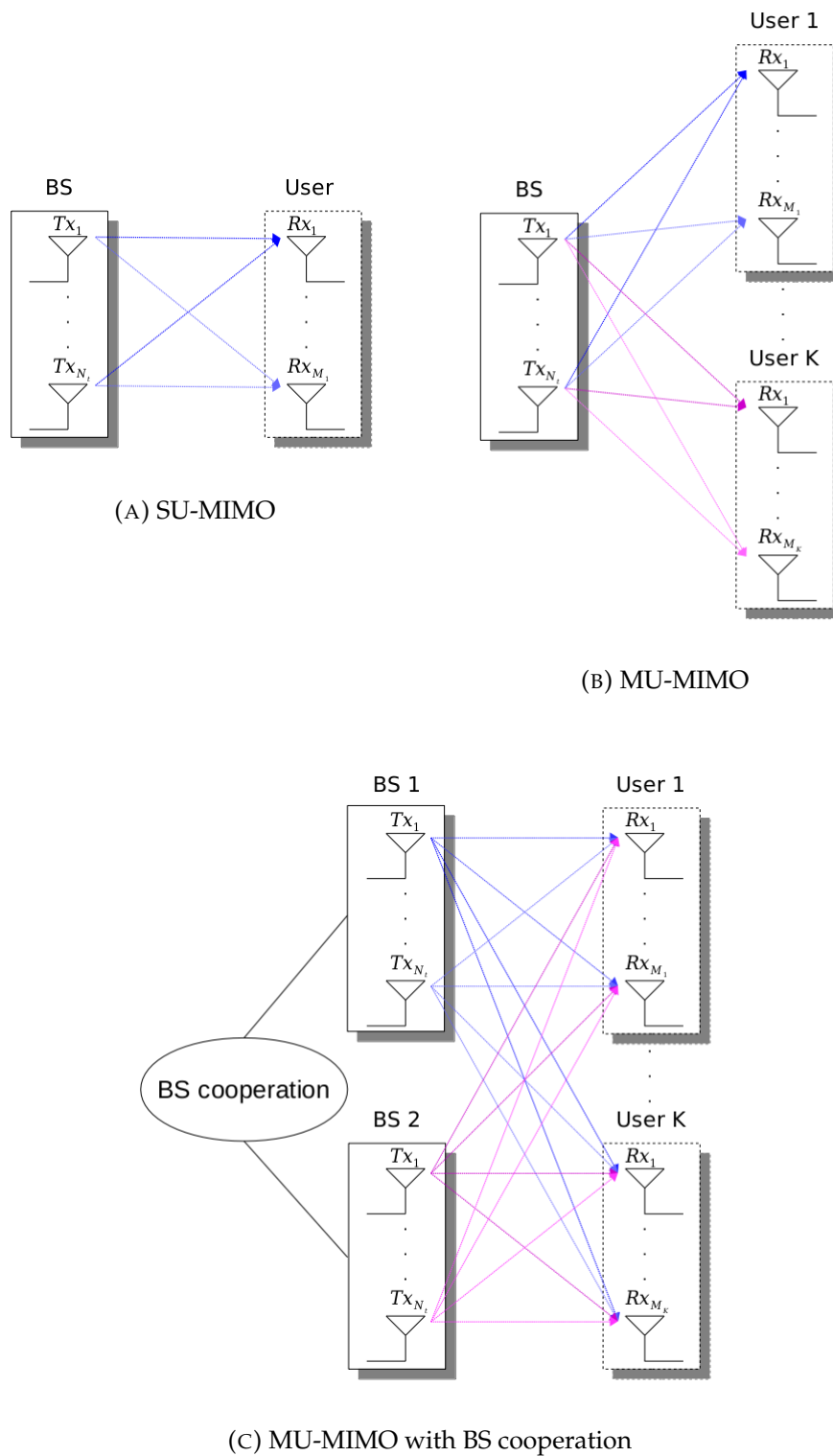
FIGURE 2.3: MU-MIMO configurations.
