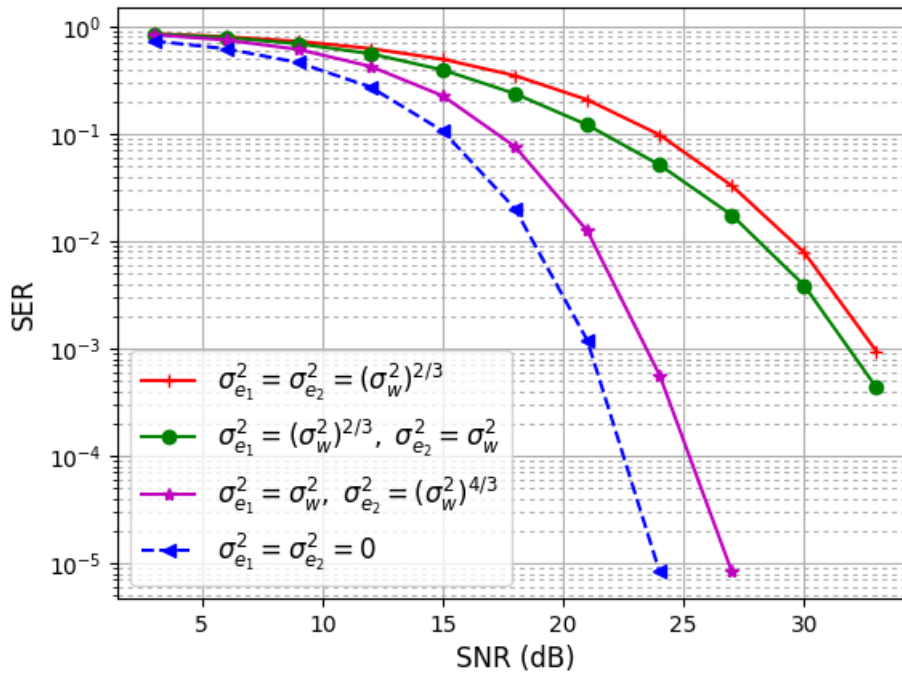
FIGURE 5.12: SER performance with varied feedback load.
