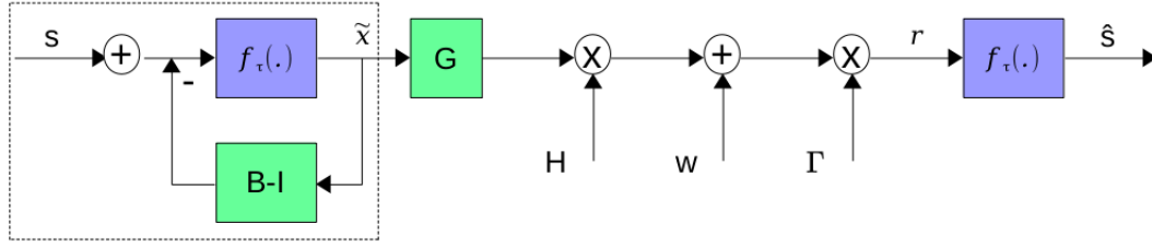
FIGURE 2.9: THP system model.
