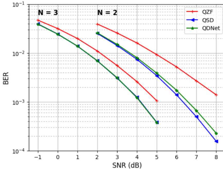
FIGURE 4.9: BER vs. SNR of different schemes for 4-QAM modulation and 5 quantization bits.
