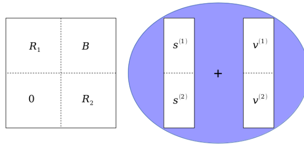
FIGURE 7.14: Block division of the precoding system.
