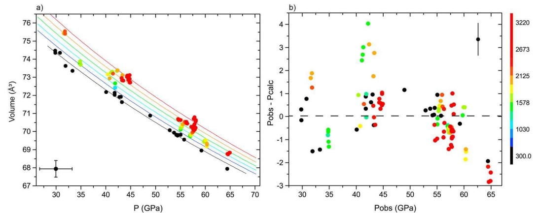
Figure 4. Results obtained fitting the zinc-blende structure with the Thermal Pressure model: (a) experimental data points and isotherms; (b) pressure residuals of the fit. On the right the temperature scale.
