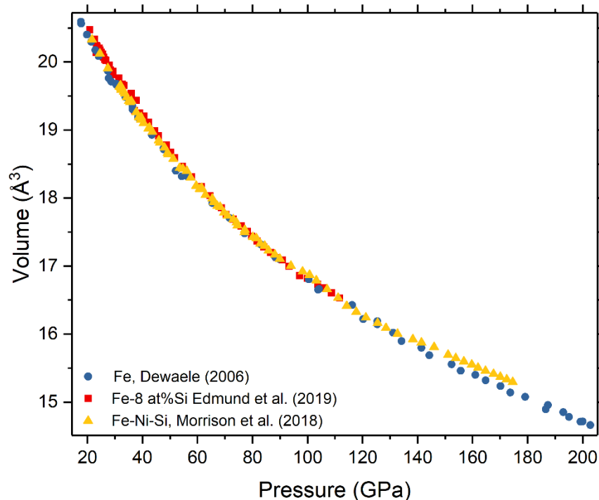
Figure 4.6: From Edmund et al. (2019). Plot of the volume over pressure data for Fe-8 at% Si, pure Fe and silicon and nickel doped iron.
