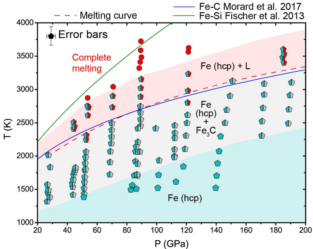
Figure 4.9: P-T diagram in the Fe-Si-C system for the composition FeSi 3 C 3 . The red dashed line represents the eutectic temperatures, above which melting occurs and (hcp) Fe is in equilibrium with a liquid. Circles represent the P-T conditions where complete melting occurred and only diffuse scattering was visible on the diffraction pattern. The melting curve is compared with those of Fe-Si (Fischer et al., 2013) and Fe-C (Morard et al., 2017).
