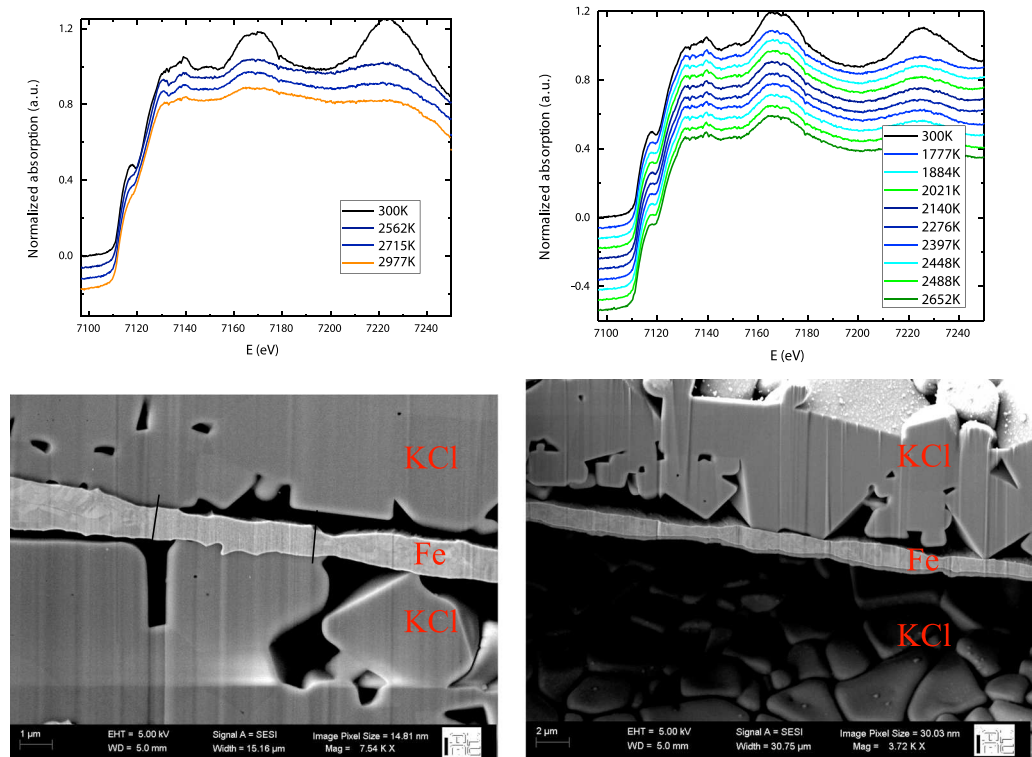
Figure 2. Validation of the melting criteria related to Fe XANES changes. Series of XANES spectra as a function of increasing temperature above (left) and below (right) the melting temperature of Fe. This melting criterion has been validated by focused ion beam cutting and SEM imaging of the hotspot cross section. Changes in the texture and irregular borders due to melting are identified on SEM figure on the left (the black lines delimitate the liquid portion of the sample). Full SEM images with a better resolution are available in the supporting information (Figures S5 and S6). XANES = X-ray Absorption Near Edge Structure; SEM = Scanning Electron Microscope.
