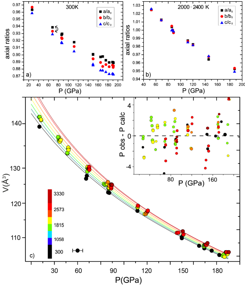
Figure 4.25: a) Fe 3 C axial ratios for a, b and c at 300K. At 60 GPa. b) Axial ratios for a, b and c at high temperature. c) Results obtained fitting the Fe 3 C data with the Mie Grüneisen Debye thermal model. In the insert the pressure residuals for the fit. Symbols represent the experimental data points collected.
