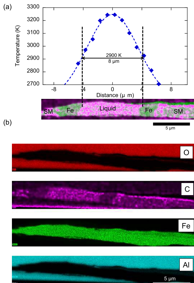
Fig. 1. (a) Temperature profile and (b) composite X-ray maps for oxygen (red), carbon (purple), iron (green), and aluminum (light blue) for run #3 performed at 138 GPa (see Fig. S1 for raw radiation spectra). Homogeneous quenched liquid is found at the center (hot part) surrounded by solid layers of iron. A measured temperature profile is combined in (a), which provides temperature at the liquid/solid boundary. (For interpretation of the colors in the figure(s), the reader is referred to the web version of this article.)
