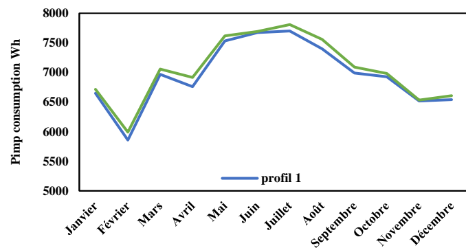
Figure 134: the variation of pump consumption using
