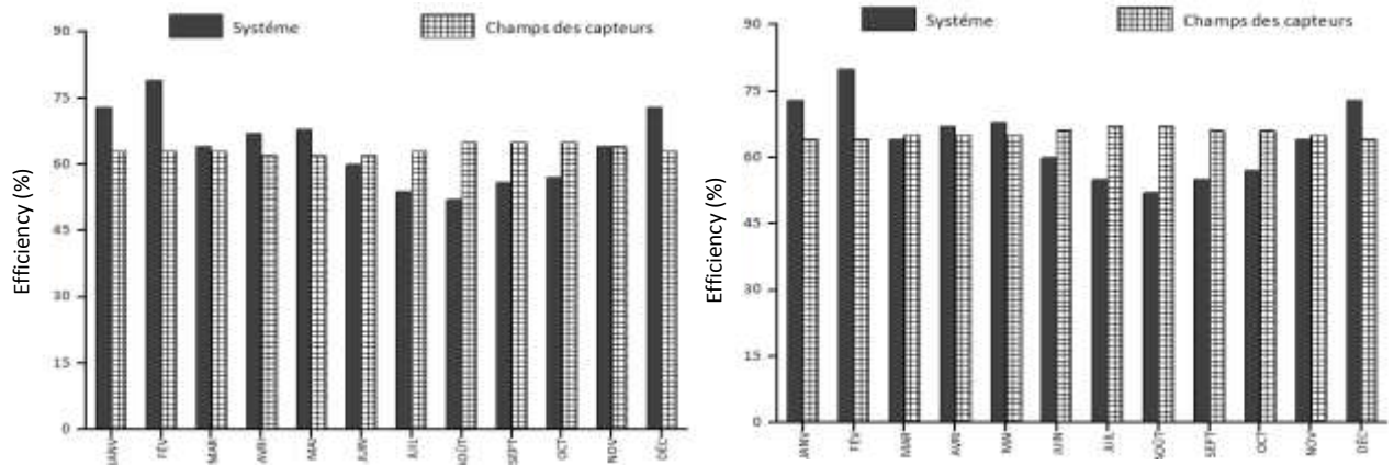
(i) (j) Figure 67: (c) flat plate collector, (d) evacuated tube collector (efficiencies).
