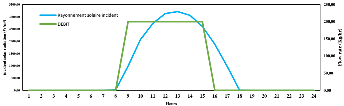
Figure 129 : Variation of incident solar radiation and water flow.
