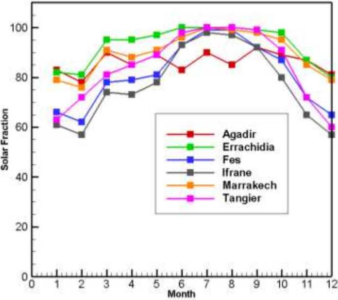
Figure 90: SHEMSY's solar fraction for the six climatic zones in Morocco.
