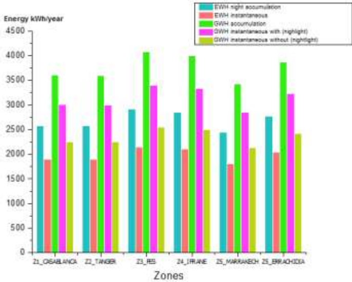
Figure 68: SWH production energy for low demand
