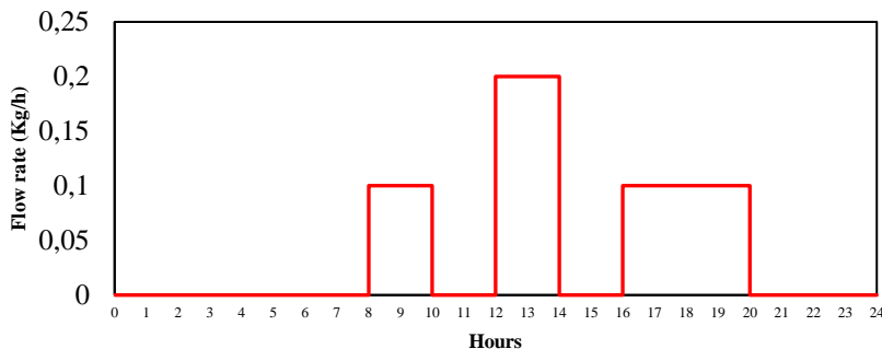
Figure 133: Load profile 3.
