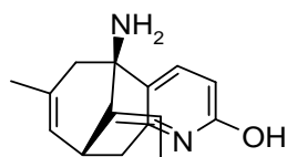
Figure 13. Huperzine A.
