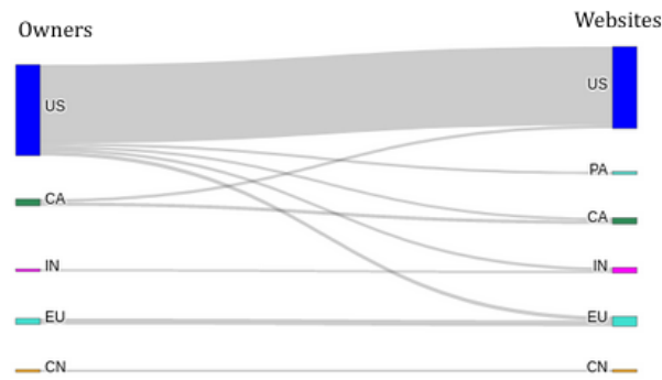
Figure 5.7: Cookie respawning with browser fingerprinting is geolocally distributed. Corresponding countries of owners (left) and websites including respawning (right) of respawned cookies. We present the top 10 (owner,website) geolocation. "EU" label represents the 27 member states of the EU.
