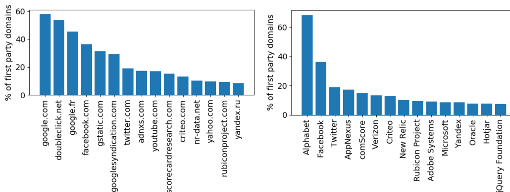
Figure 3.5: Basic tracking: Top 15 cross-site trackers and companies in charge of the trackers included in 8,744 domains.
