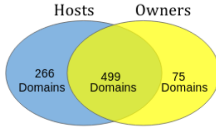
Figure 5.4: Emergence of new domains when considering cookie owners. The 1,425 respawned cookies have 765 distinct hosts and 574 distinct owners. The notion of cookie owner allows to identify 75 cookie owner domains that never appear as a cookie host. We also found 266 cookie host domains that are never used to set the cookie.
