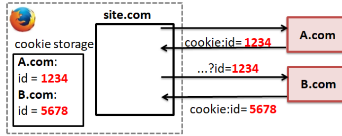
Figure 2.5: Third to third party cookie syncing behavior. First, site.com includes A.com, a request is then sent to A.com along with it's cookie. Next, A.com redirects the request to B.com and includes it's identifier 1234 in the request URL. Then, B.com receives the request along with it's cookie. This behavior allows A.com and B.com to combine the data collected about the user.
