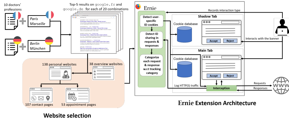
Figure 4.2: High level overview of our experimental setup. Website selection process as well as browser setup and website analysis is described in the remainder of this section. ERNIE extension architecture is presented in details in Section 2.1.
