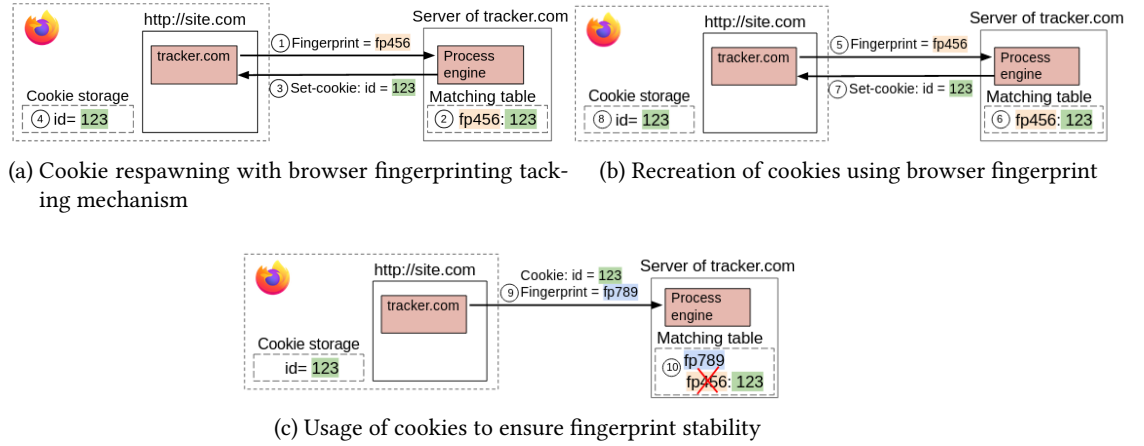
Figure 5.1: Cookie respawning with browser fingerprinting tracking technique.
