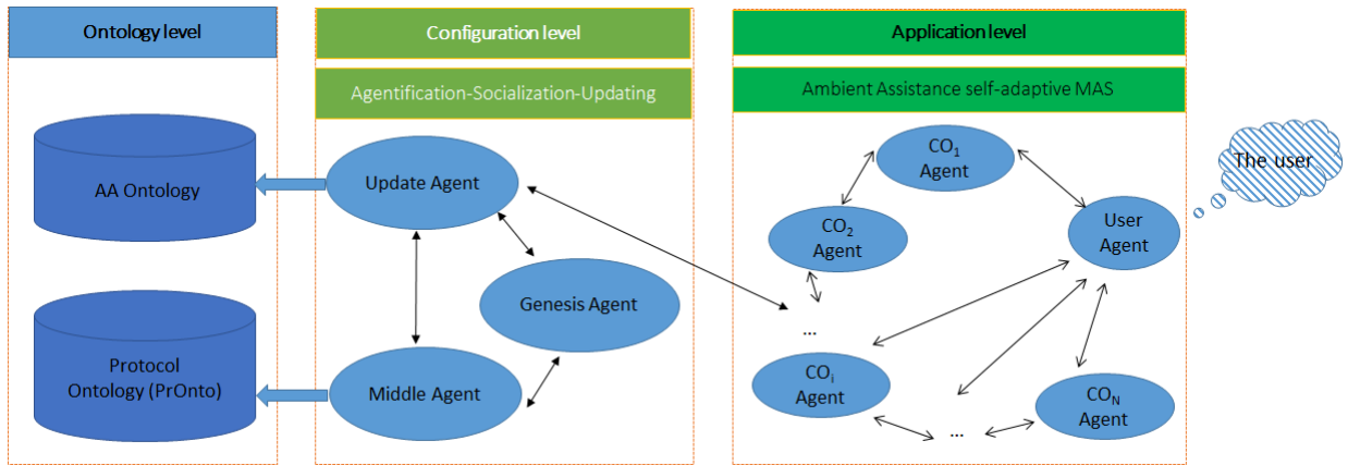
Figure 4.1 – GAAMAAA Architecture
