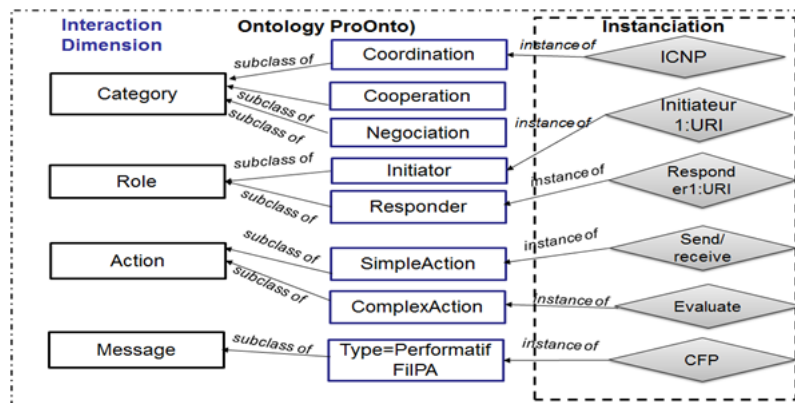
Figure 4.8 – Interaction protocol
