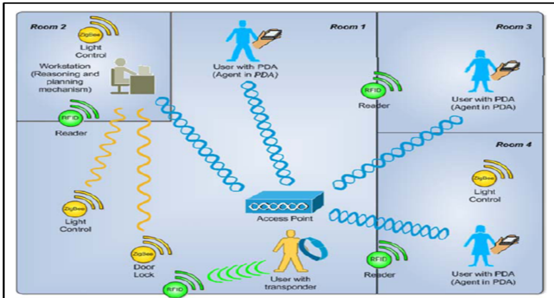
Figure 2.1 – ALZ-MAS basic schema [J.Corchado et al. 2008]
