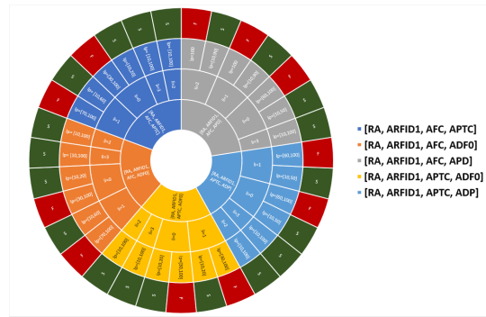
Figure 5.6 – Coalition SA Cardinality = 4
