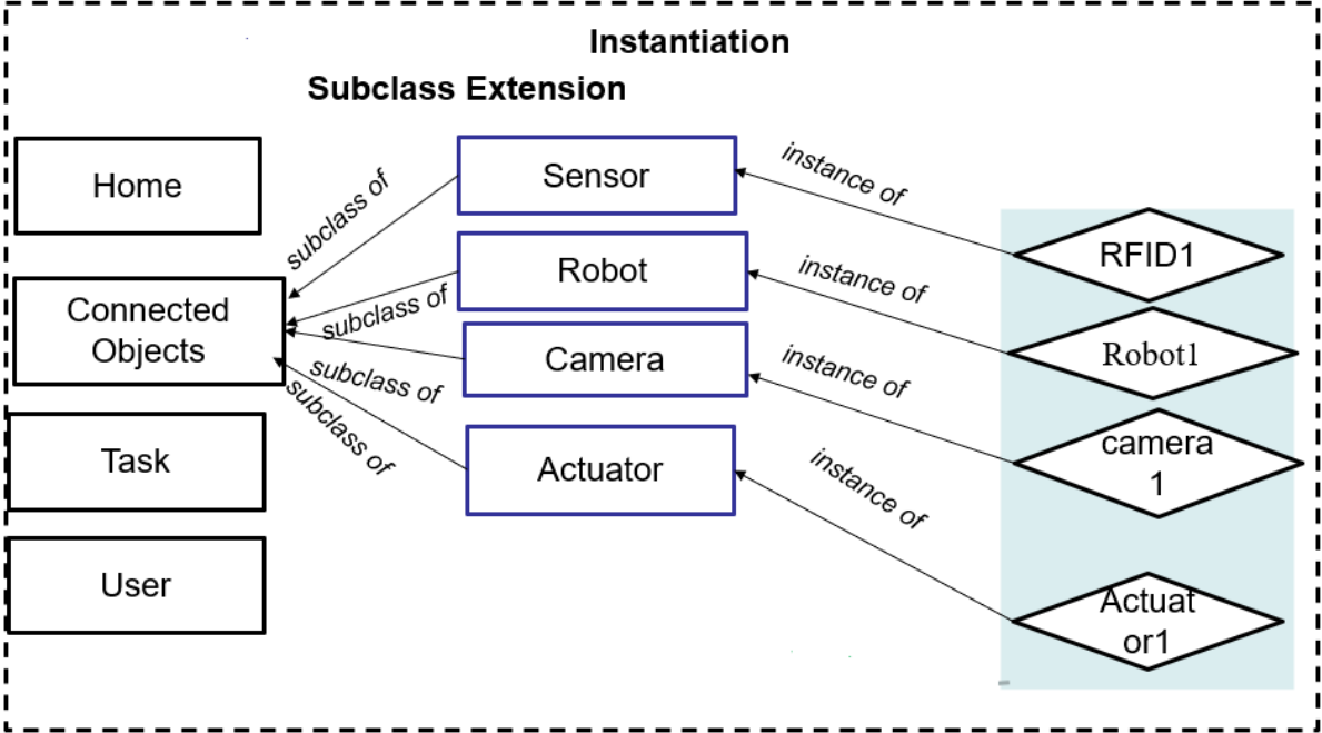
Figure 4.5 – Environmental of the ontology for MAS
