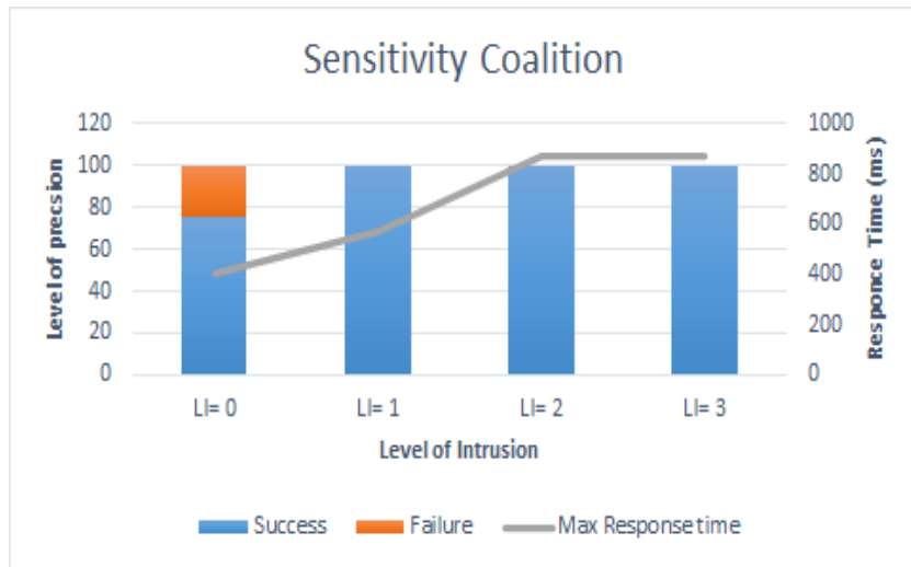
Figure 5.20 – Coalition SA results
