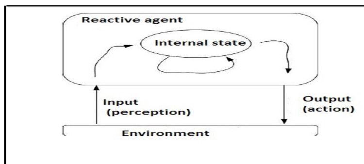
Figure 1.3 – Reactive architecture
