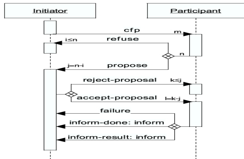
Figure 1.5 – Contract Net Interaction Protocol
