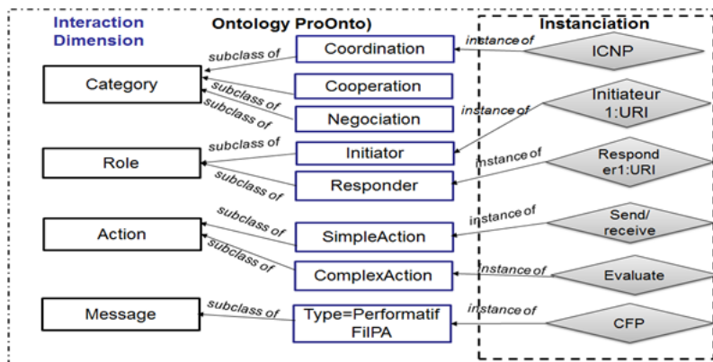
Figure 4.8 – Interaction protocol
