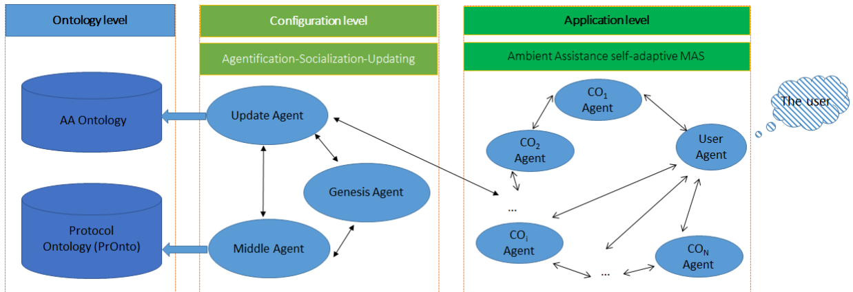
Figure 4.1 – GAAMAAA Architecture
