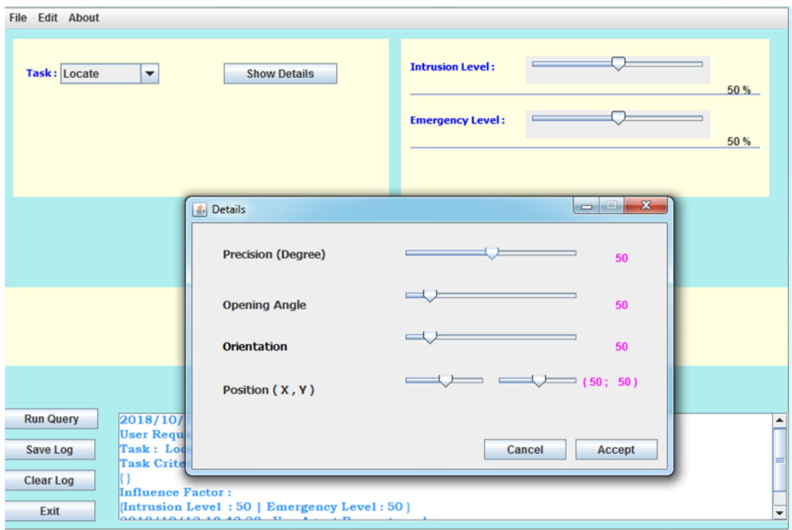
Figure 4.4 – Interface of service request
