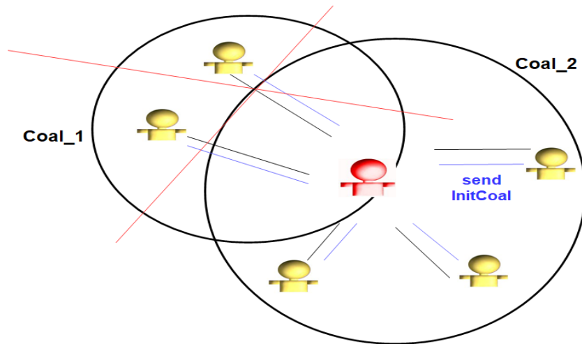
Figure 1.6 – Coalition Protocol
