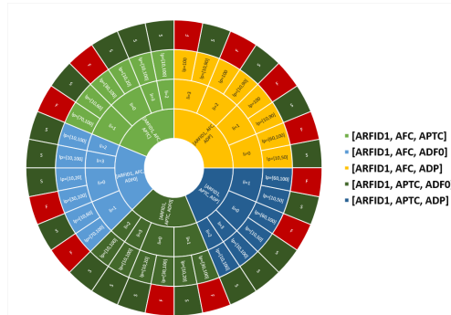
Figure 5.16 – Coalition SA Cardinality = 3
