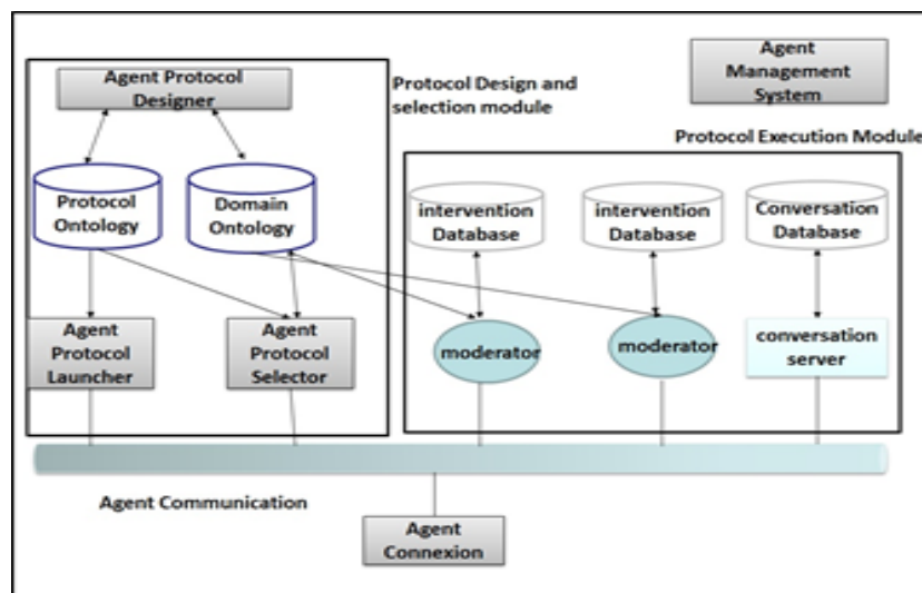
Figure 2.3 – Protocol Management System [W.Bouaziz & E.Andonoff 2015]
