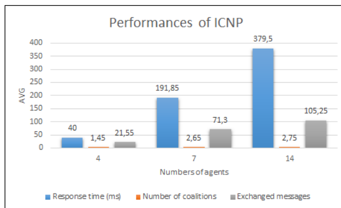
Figure 4.10 – Performances of ICNP
