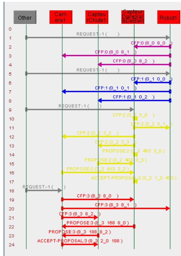
Figure 4.9 – Agent interaction diagram in Jade platform
