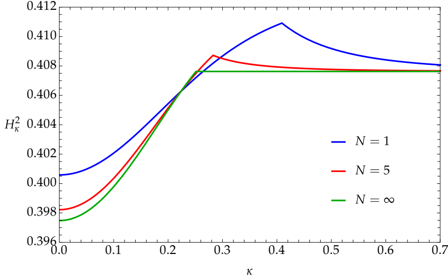
Figure 2.8: Flow of H_\kappa^2 in the broken-symmetry regime for various values of N , for m^2 = -0.05 , \zeta = 0 and \lambda = 1 . We also chose \beta = 1 and \alpha = 0.1 . The flow in the broken phase is entirely due to the longitudinal mode, and is suppressed as N is increased, up to the limit N \rightarrow \infty , where only the massless transverse modes contribute.
