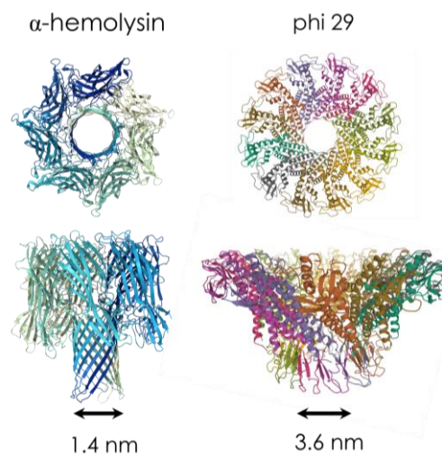
Figure 1.7: \alpha -hemolysin nanopore structure (PDB: 7AHL) and Phi29 motor nanopore structure (PDB: 1JNB).
