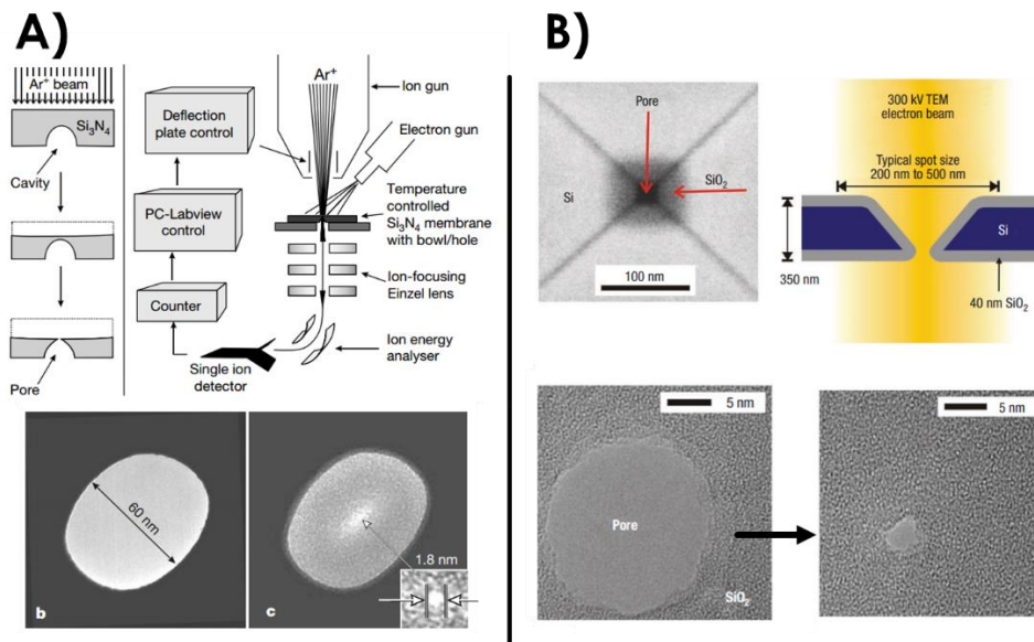
Figure 2.1: A) Nanopore fabrication technique using FIB first presented by Li et al. 26 Ion beam irradiation causes nanopore shrinking. B) Top view and cross section of the nanopore device by Storm et al. 18 , electron irradiation in TEM causes nanopore shrinking.
