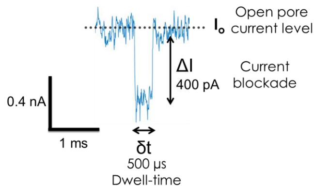
Figure 3.5: An example of current data for a translocation signal event of \lambda DNA in a 12 nm diameter \text{SiN}_x nanopore at + 200 mV (1 M KCl, 1 mM Tris/HCl, 0.1 mM EDTA buffer).
