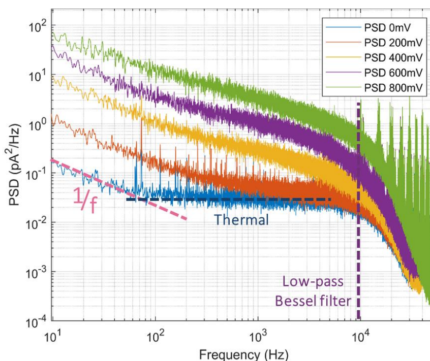
Figure 4.2: Power Spectral Density (PSD) for a 12 nm nanopore at different applied voltages in the buffer for protein and aptamer experiments (Tris-HCl 20 mM, MgCl 2 1 mM, NaCl 120 mM, KCl 10 mM, pH 7.4).
