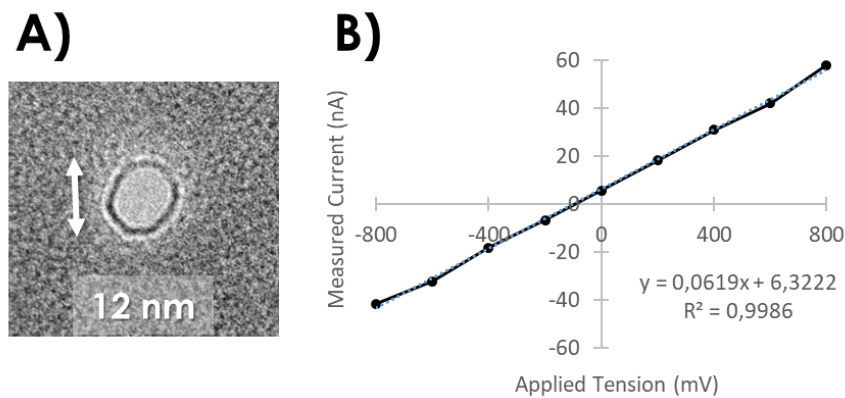
Figure 4.3: A) TEM image of the drilled \text{SiN}_x nanopore (12 nm diameter in 20 nm thick membrane). B) I-V curve characterization of the nanopore in the buffer for \lambda DNA translocations (1 M KCl, 1 mM Tris-HCl, 0.1 mM EDTA, pH 8). The experimental conductance G_{\text{exp}} is equal 61.9 nS, obtained with a linear fit (dotted line).
