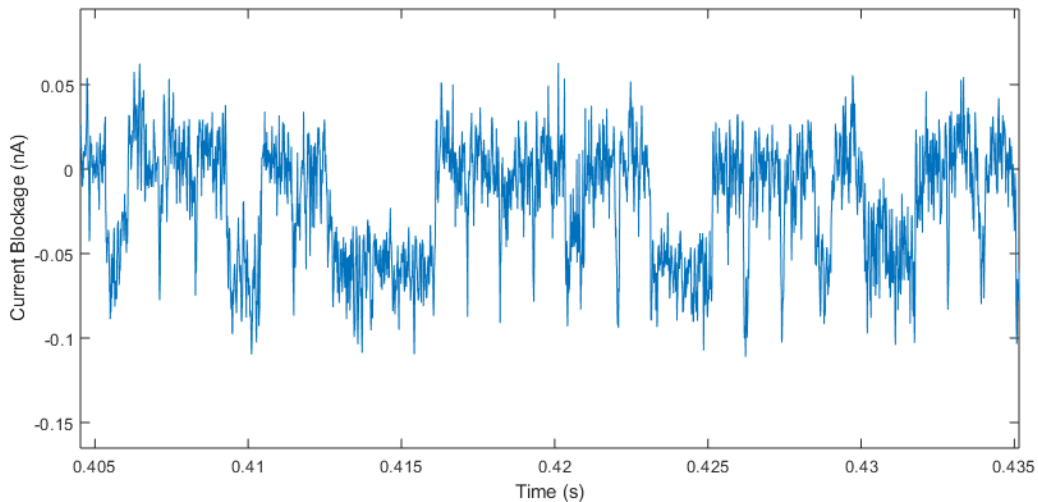
Figure 4.21: \alpha -Thrombin sensing in the aptamer-functionalized nanopore. Zoom-in of the concatenated signal with only the events detected by OpenNanopore (baseline set to 0 nA).
