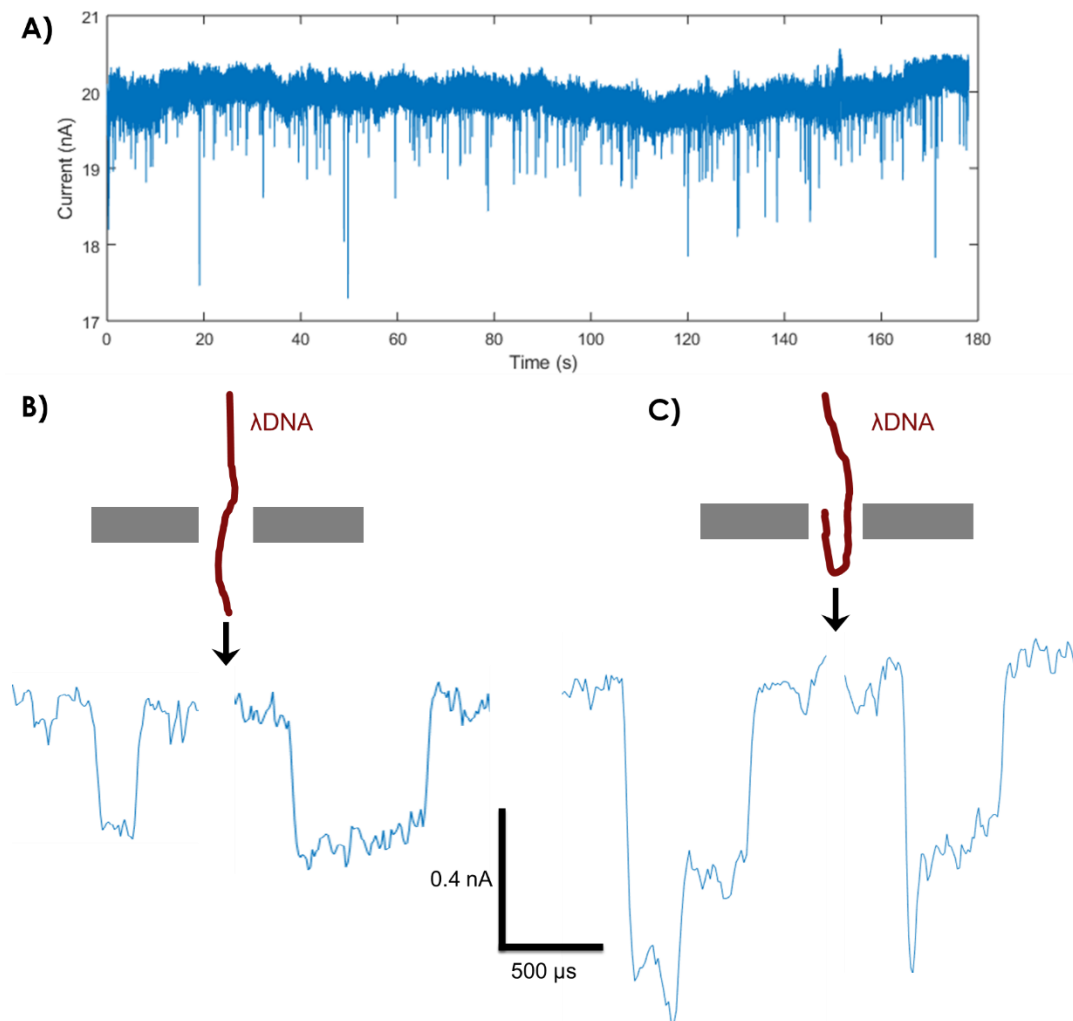
Figure 4.4: A) 3-minute recording of single-events detection of \lambda DNA in a 12 nm diameter \text{SiN}_x nanopore. \lambda DNA at 3 ng/ \mu\text{L} in the buffer for \lambda DNA translocations (1 M KCl, 1 mM Tris-HCl, 0.1 mM EDTA pH 8.0). B) Illustration and focus on two typical single-events of \lambda DNA going linearly into the pore. C) Illustration and focus on two typical single-events of \lambda DNA going partially folded into the pore.
