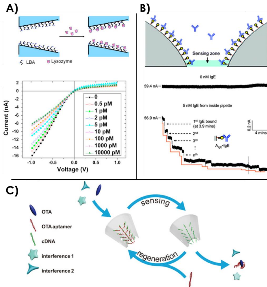
Figure 1.16: A) Illustration of lysozyme binding aptamer grafting on a 20 nm conical glass nanopores and induced ICR after addition of various concentrations of lysozyme protein 301 . B) Consecutive current decrease steps with immunoglobulin binding on the surface aptamers from reference 134 . C) Strategy for OTA toxin detection with DNA direct immobilization of aptamers from reference 305 .
