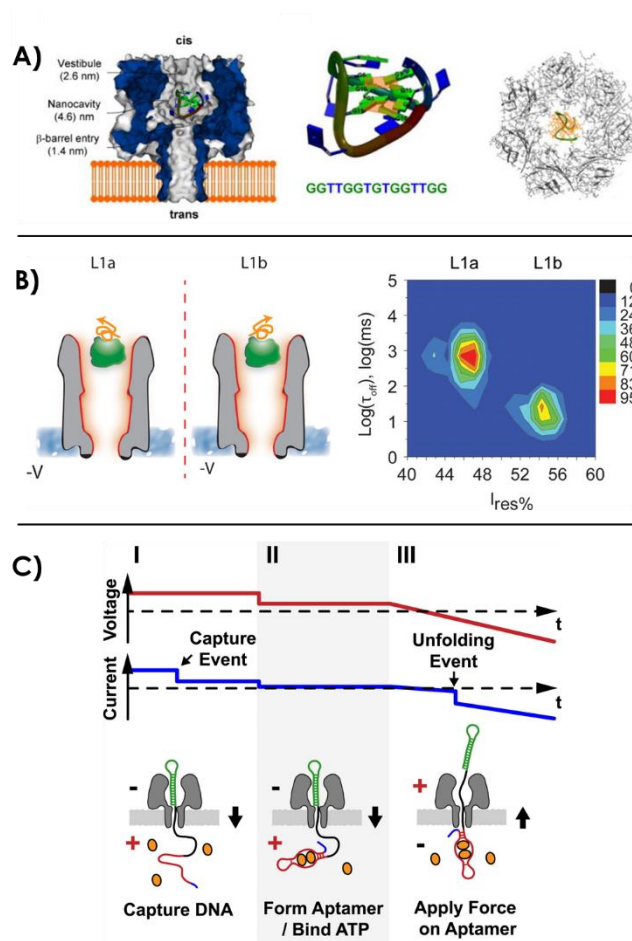
Figure 1.12: A) Capture of the folded G-quadruplex aptamer in the \alpha -hemolysin nanopore cavity. When linearized, the aptamer is able to go through the narrowest region of the pore and translocates 245 . B) Aptamer-ligand conformation study of thrombin-binding aptamer and two possible isomeric configurations demonstrated with a ClyA nanopore 252 . C) Nanopore force spectroscopy of an ATP-aptamer complex 254 .
