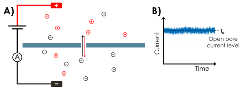
Figure 1.5: Illustration of solid-state nanopore principle. A) A dielectric membrane separates two electrolyte reservoirs that are connected solely through the nanopore. Electrodes are placed at each side of the membrane and a voltage is applied. B) Measured ionic current results from the electrolyte charges moving through the nanopore. I_0 is the open-pore current level.
