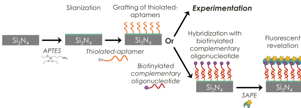
Figure 3.15 : Different steps of the surface functionalization of \text{SiN}_x with aptamers. First, the surface is silanized in order to graft aptamers. Then, the chip can either be used for protein sensing experimentations or be hybridized with the biotinylated complementary oligonucleotide for a further fluorescent revelation using SAPE.
