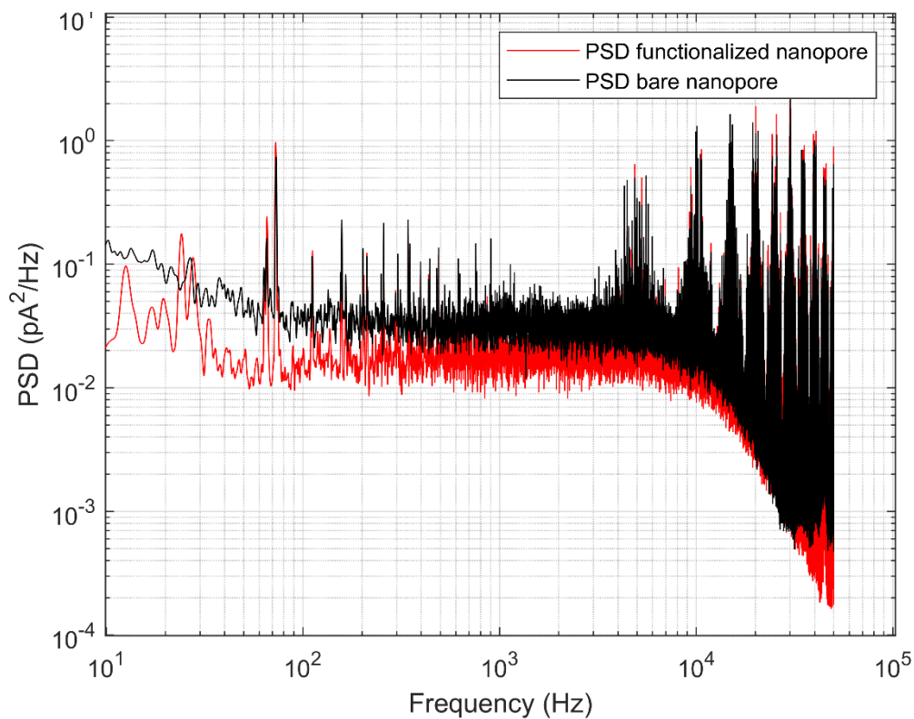
Figure 4.10: Power Spectral Density (PSD) of a 12 nm diameter nanopore measurement at 0 mV in the buffer for protein and aptamer experiments (Tris-HCl 20 mM, MgCl 2 1 mM, NaCl 120 mM, KCl 10 mM, pH7.4) before (black) and after its surface functionalization with aptamers (red).
