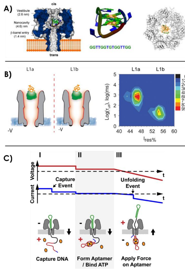
Figure 1.12: A) Capture of the folded G-quadruplex aptamer in the \alpha -hemolysin nanopore cavity. When linearized, the aptamer is able to go through the narrowest region of the pore and translocates 245 . B) Aptamer-ligand conformation study of thrombin-binding aptamer and two possible isomeric configurations demonstrated with a ClyA nanopore 252 . C) Nanopore force spectroscopy of an ATP-aptamer complex 254 .
