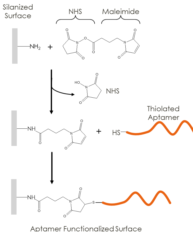
Figure 3.18: Aptamer grafting on the SiN x aminated silanized surface via a maleimide-NHS linker.
