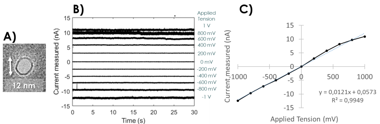
Figure 4.1: Experimental determination of the conductance of a 12 nm diameter nanopore in the buffer for protein and aptamer experiments (Tris-HCl 20 mM, MgCl 2 1 mM, NaCl 120 mM, KCl 10 mM, pH7.4). A) TEM image of the pore. B) Measured current as a function of time for an applied voltage range of [-1 V; +1 V] with a 200 mV voltage step. C) I-V curve of the same nanopore, with current values extracted from B), the slope of this curve fitted by the dotted line gives the nanopore experimental conductance G_{\text{exp}} = 12.1 \text{ nS} .
