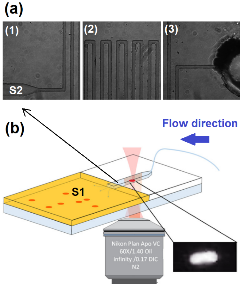
FIGURE 3.1: (a) Microfluidic chip used for investigating the adsorption of macromolecules onto RBCs. (1): Area of observation situated at about 500 \mu\text{m} from the "pool" (S1), (2) resistance-channel to decrease the flow velocity and (3) inlet where the buffer solution is injected. (b) Sketch representing a single RBC dragged from a macromolecule solution (in the "pool" S1) to a buffer solution "S2"
