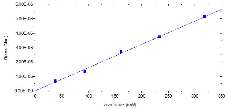
FIGURE 2.9: Stiffness calibration using the thermal noise method for a generated trap as a function of the laser power
