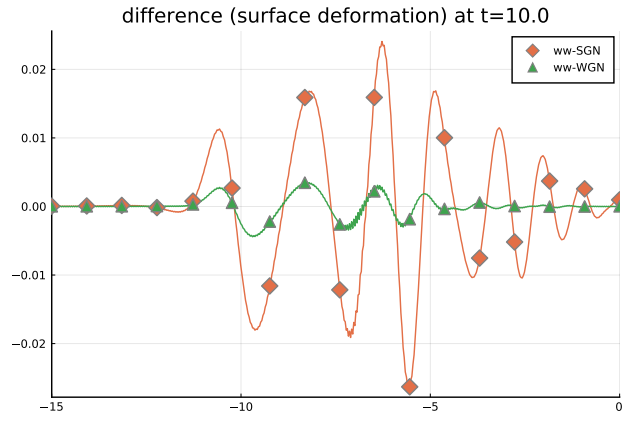
(d) Difference at time t = 10 . \mu = 0.1 , \varepsilon = 0.25
