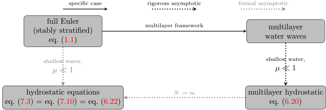
Figure 7.2 – Hydrostatic limits.
