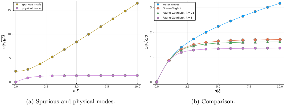
Figure 9.1 – Wave frequencies, |\omega_{\pm}|(|\xi|) , corresponding to the Favrie–Gavrilyuk system, and comparison with the water waves and the Green–Naghdi systems.
