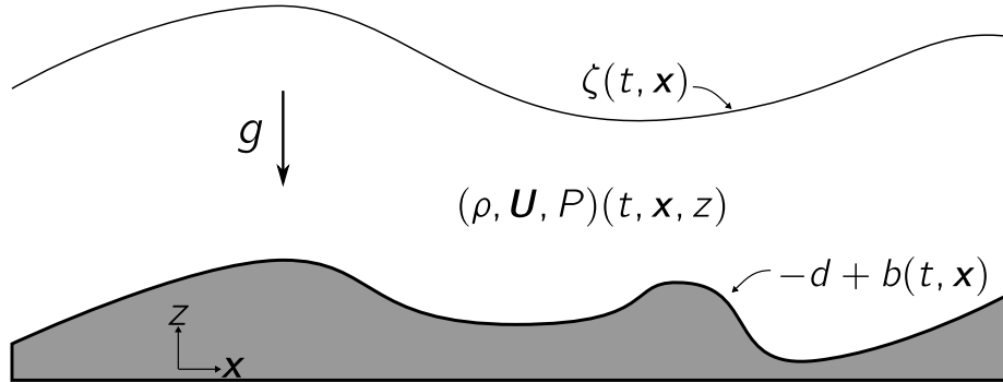
Figure 1.1 – Sketch of the domain and notations
