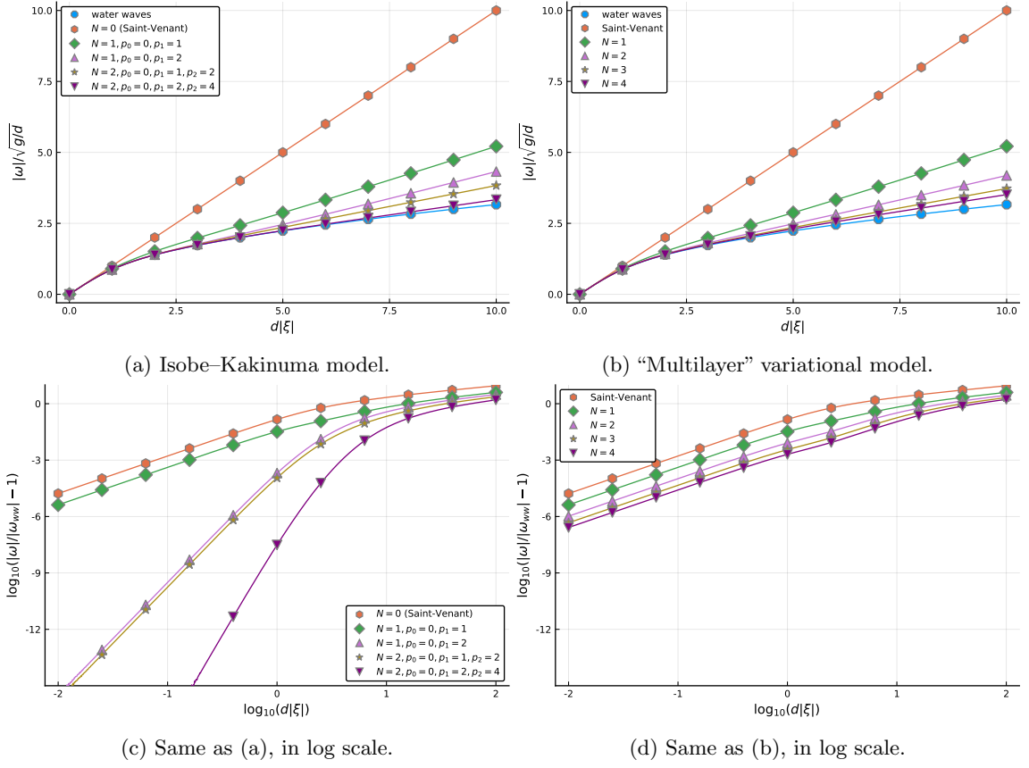
Figure 13.1 – In (a) and (b), wave frequencies, |\omega|(|\xi|) , given by the dispersion relations corresponding to the (linearized about rest) Isobe-Kakinuma and “multilayer” variational models, respectively. In (c) and (d), the “error” is represented in log scale.
