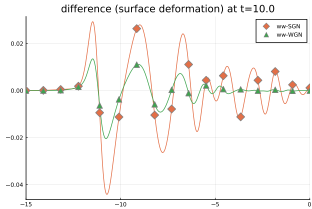
(f) Difference at time t = 10 . \mu = 0.1 , \varepsilon = 0.5
