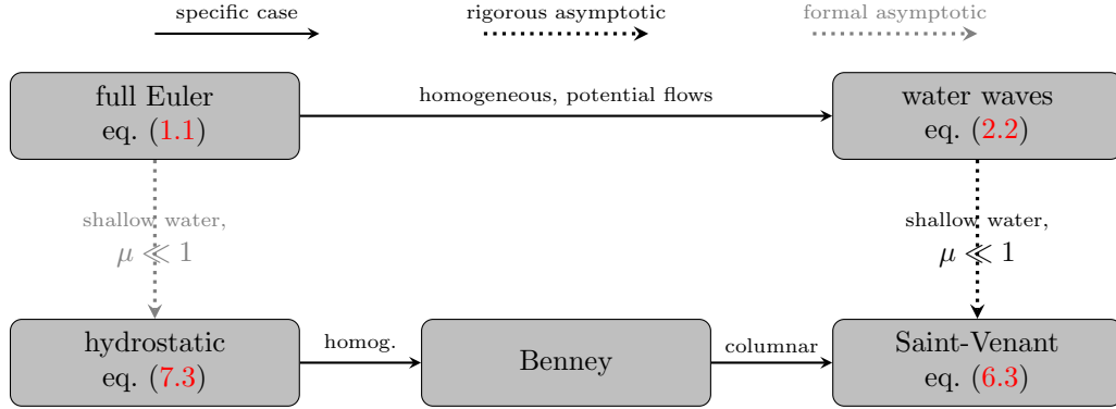
Figure 7.1 – Some hydrostatic models.
