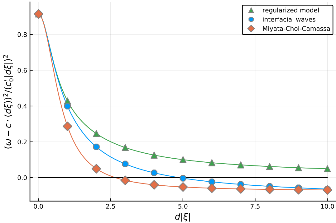
Figure 14.3 – Dispersion relation. We plot (\omega(\xi) - c(\xi) \cdot \xi)^2 / |\xi|^2 = a(\xi)b(\xi) / |\xi|^2 (with \mu = 1 ) for the full bilayer interfacial waves system (and hence the fully dispersive model), the original Miyata–Choi–Camassa model and a regularized model; negative values indicate unstable modes.
