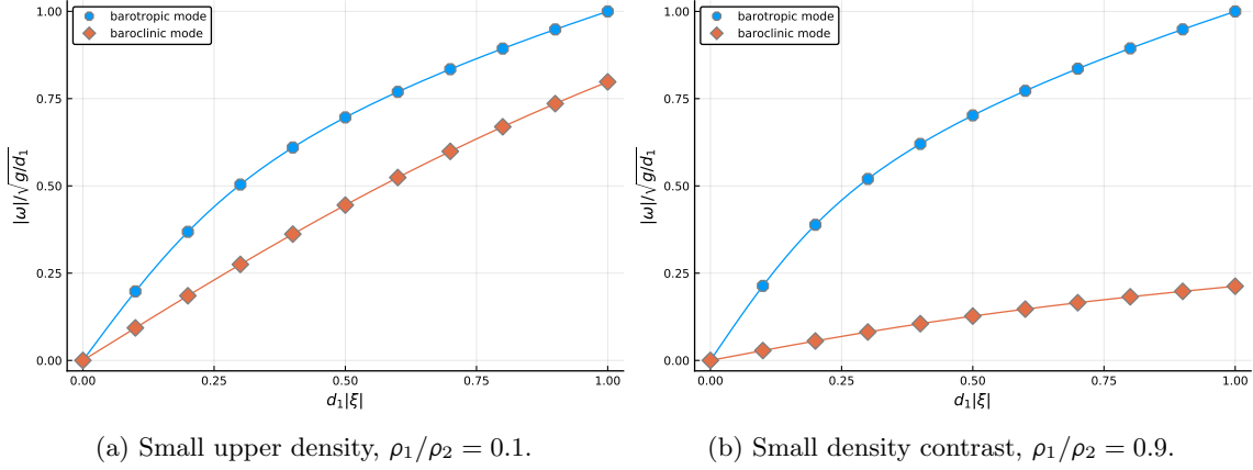
Figure 3.2 – Wave frequencies, |\omega|(d_1|\xi|) , according to eq. (3.11). d_2 = 4d_1 .
