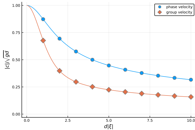
Figure iii – Phase and group velocities of the linearized water waves equations.
