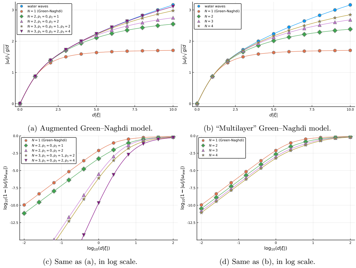
Figure 12.1 – In (a) and (b), wave frequencies, |\omega|(|\xi|) , given by the dispersion relations corresponding to the (linearized about rest) augmented and “multilayer” Green–Naghdi models, respectively. In (c) and (d), the “error” is represented in log scale.
