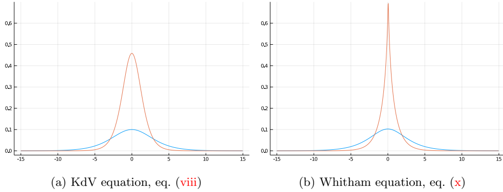
Figure vi – Solitary waves of unidirectional models with velocity c = 1.05c_0 (blue, smaller) and c = 1.2290408c_0 (red, larger). g = 9.81 \text{ m.s}^{-2} , d = 1 \text{ m} , c_0 = \sqrt{gd} .
