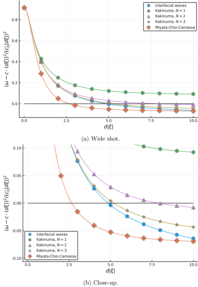
Figure 15.1 – Dispersion relation. We plot (\omega(\xi) - \mathbf{c}(\xi) \cdot \xi)^2 / |\xi|^2 = a(\xi)b(\xi) / |\xi|^2 (with \mu = 1 ) for the full bilayer interfacial waves system, Kakinuma systems and Miyata–Choi–Camassa model, as predicted by eq. (3.12), eq. (15.25) and eq. (14.7); negative values indicate unstable modes.
