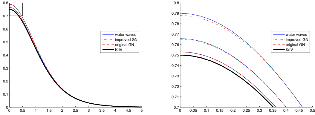
(a) Rescaled solitary waves for c = 1.025, 1.01, 1.002 .
