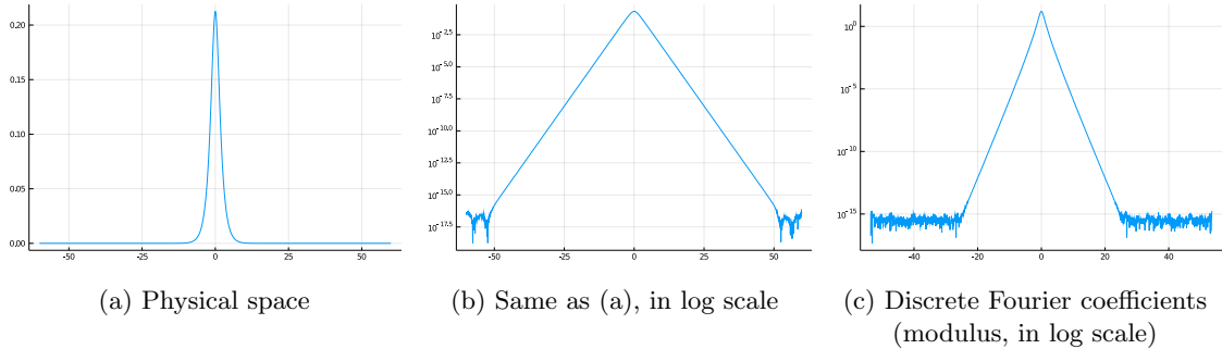
Figure I.1 – Computed solitary wave of eq. (I.1) with velocity c = 1.1 .
