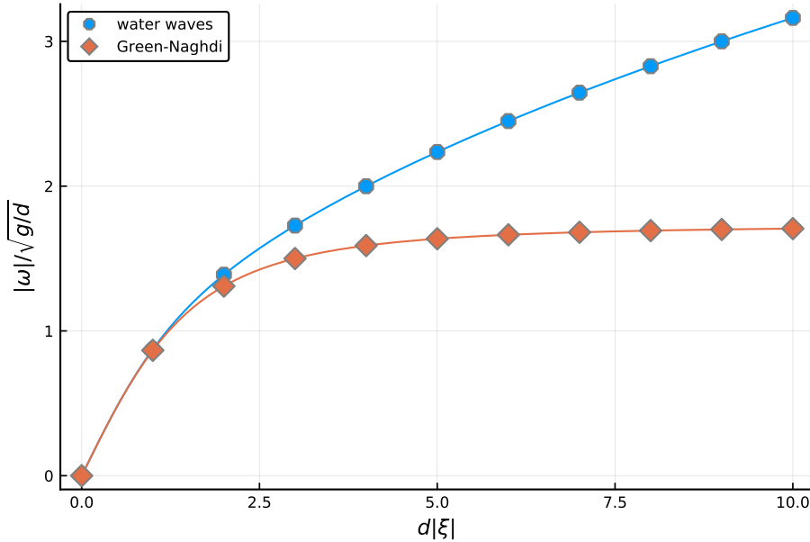
Figure 8.1 – Non-trivial wave frequencies, |\omega|(|\boldsymbol{\xi}|) , solutions to the dispersion relation corresponding to the (linearized about rest) water waves and Green–Naghdi systems.
