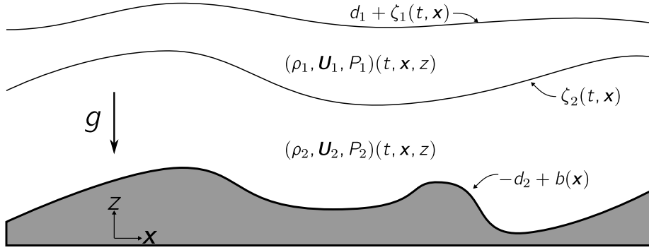
Figure 3.1 – Sketch of the domain and notations
