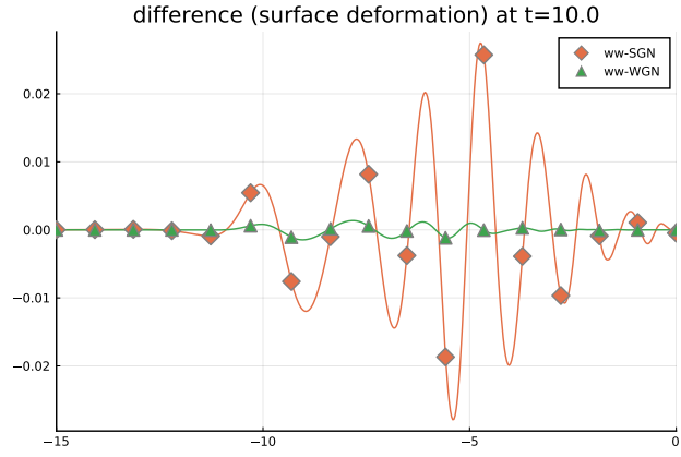
(b) Difference at time t = 10 . \mu = 0.1 , \varepsilon = 0.125
