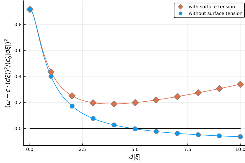
Figure 3.3 – Dispersion relation. We plot (\omega(d\xi) - c(d\xi) \cdot d\xi)^2 / |c_0' d\xi|^2 = a_\sigma(d\xi)b(d\xi) / |c_0' d\xi|^2 ; negative values indicate unstable modes.
