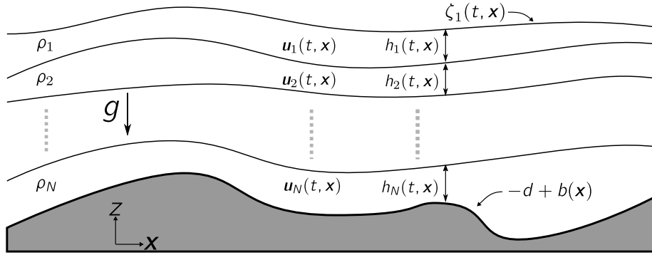
Figure 6.3 – Sketch of the domain and notations in the multilayer framework.
