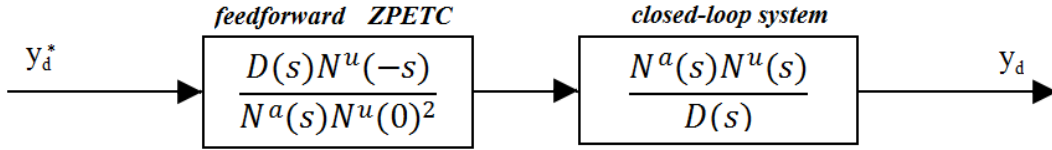
Figure 3.4 – Block diagram of the original ZPETC.
