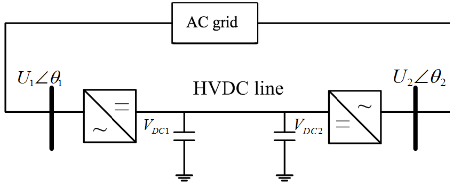
Figure 2.2 – HVDC inserted in an AC grid.
