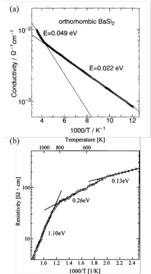
Fig. 2.5-1 Electrical conductivity of BaSi 2 as a function of reciprocal temperature, 1/T in the temperature region (a) 80-290 K, 88 and (b) RT-1200 K. 89
