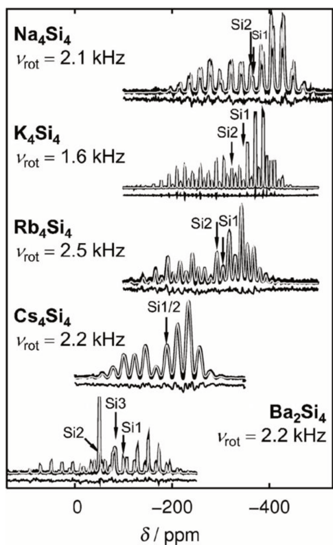
Fig. 2.5-10 29 Si MAS NMR signal. The positions of the isotropic shifts are marked by arrows. 110
