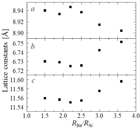
Fig. 4.1-3. The lattice constants ( a , b , and c ) of the films. Each constant was determined by the Nelson-Riley relationship. 122
