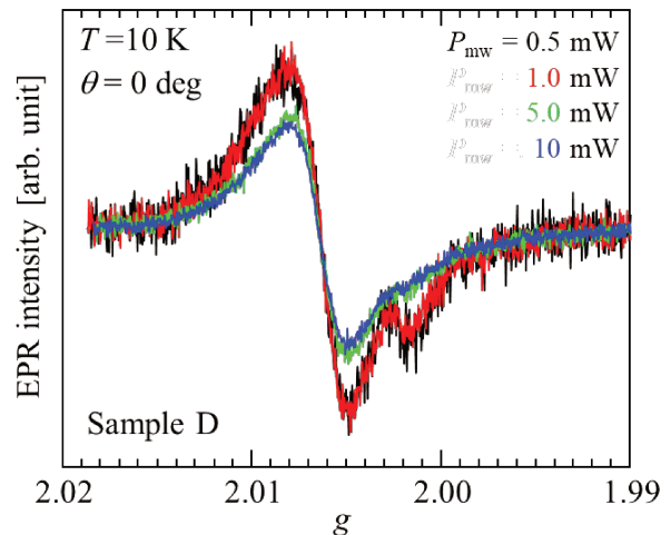
Fig. 4.3-2. Microwave power ( P_{MW} ) dependence of the EPR spectra recorded at 10 K with \theta = 0 deg.
