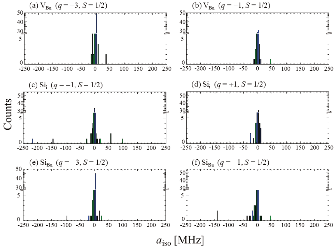
Fig. 5.5-3 Isotropic part of hyperfine tensor for the defects under Si-rich condition. Blue and green bars correspond to 29 Si and 135 Ba ( 137 Ba) atoms, respectively.
