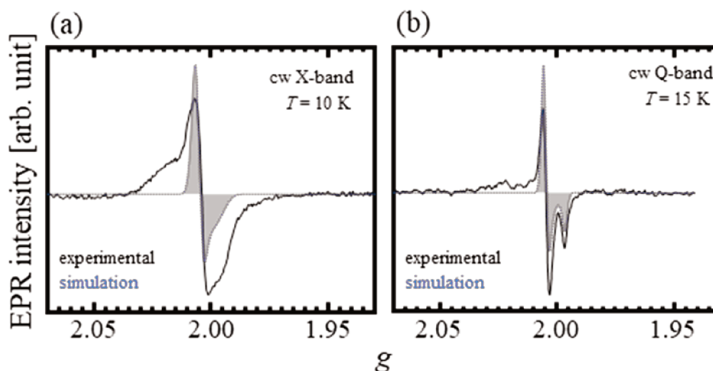
Fig. 5.4-1 Experimental and simulated spectra of Sample I.
