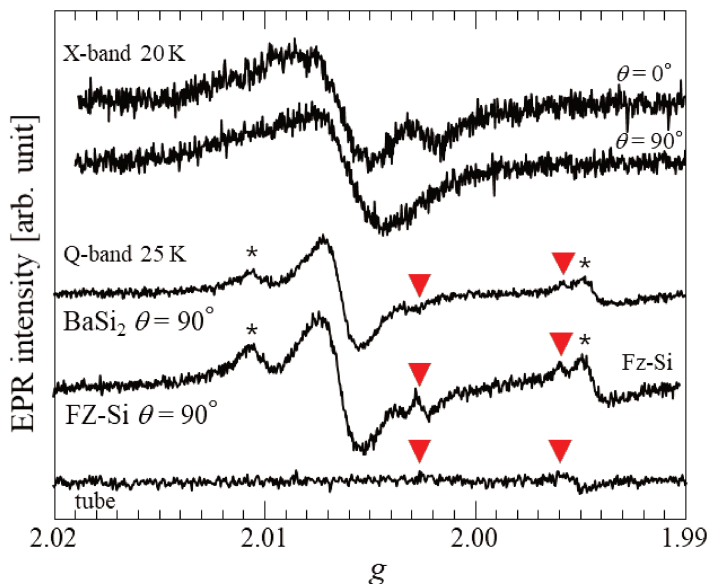
Fig. 4.4-2 The EPR spectra of BaSi 2 film, FZ-Si substrate, and the annealed EPR tube. Even after annealing the tube, a few paramagnetic centers ( \blacktriangledown ) remained.
