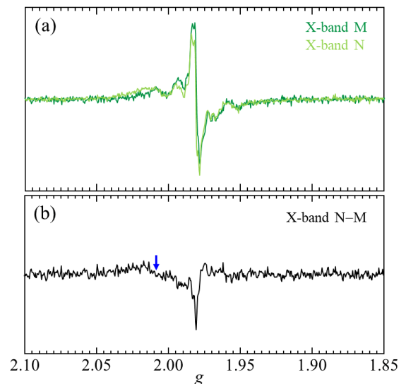
Fig. 5.1-4 (a) EPR spectra of Sample M and N recorded with X-band frequency at 50 K. (b) A Subtracted spectrum (Sample N – Sample M). I speculated that a line placed at blue arrow corresponded to that observed in Si-rich samples.
