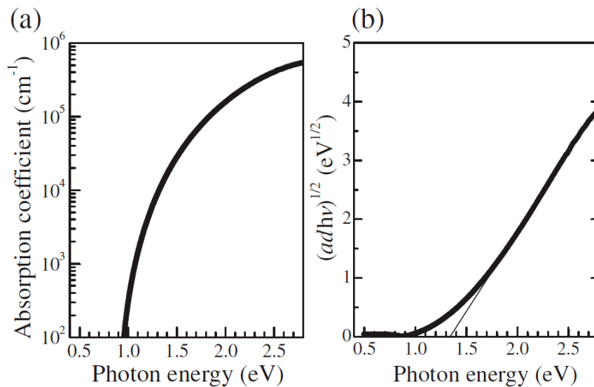
Fig. 2.2-2 (a) Absorption spectrum and (b) (\alpha h\nu)^{1/2} versus photon energy plotted for BaSi 2 . 41
