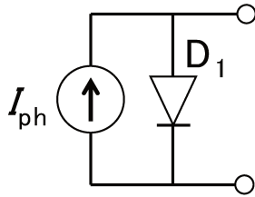
Fig. 1.2-5 Ideal solar cell equivalent circuit.
