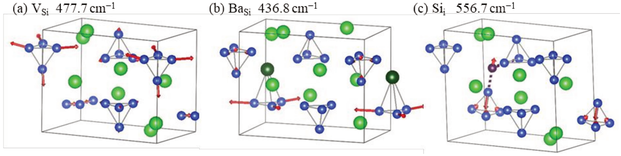
Fig. A.3-2 Local vibrational modes of (a) V_{Si} , (b) Ba_{Si} , and (c) Si_i .
