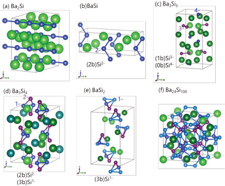
Fig. 2.1-3 Crystal Structure of Ba-Si binary compounds. (a) Ba 2 Si, 28 (b) BaSi, 29 (c) Ba 3 Si 5 , 30 (d) Ba 3 Si 4 , 31 (e) BaSi 2 , 22 and (f) Ba 24 Si 100 . 32 Big and small circle correspond Ba and Si atoms, respectively. (#b) indicate the number of Si bonds with its charge.
