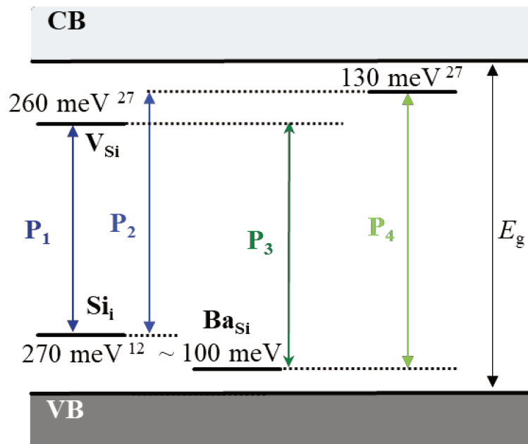
Fig. 6.4-3 A model of radiative defects in BaSi_2 . Each assignment is discussed in the text.
