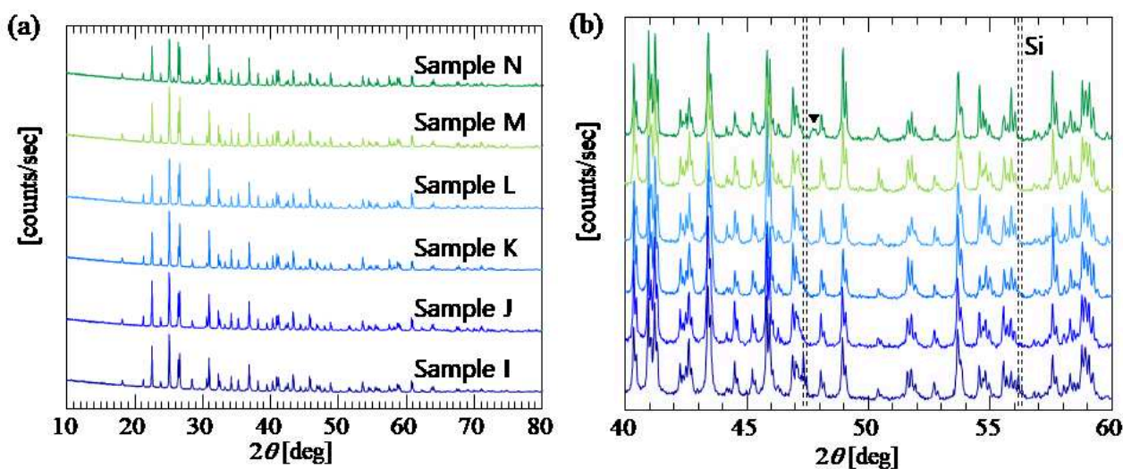
Fig. 5.1-1 (a) Powder XRD pattern of sample I–N. (b) Enlarged the results of (a) between 2\theta = 40 – 60 deg. In sample I, at 2\theta = 47.5 and 56 deg, the peaks of crystallized Si were observed. In sample N, the peak of precipitation (probably Ba 3 Si 4 31 ) was confirmed at 2\theta = 48 deg (as shown as a triangle, ▼).
