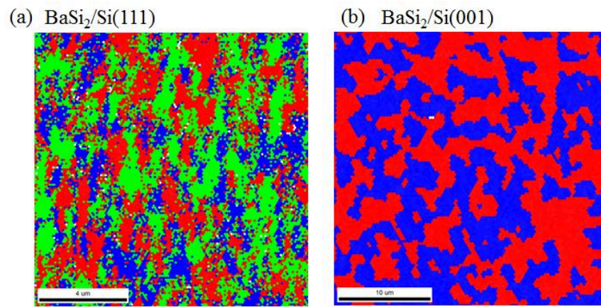
Fig. 2.3-2 EBSD maps of BaSi 2 films on (a) Si(111) and (b) Si(001). 61,63
