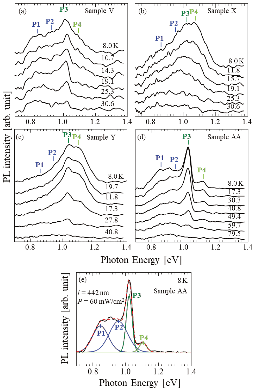
Fig. 6.3-3 Temperature dependence of PL spectra of (a) sample V, (b) sample X, (c) sample Y, and (d) sample AA. (e) A typical fitting result for sample AA assuming four Gaussian curves were shown as a red broken line. Each sample contains four different transition as denoted by P 1 (dark blue), P 2 (blue), P 3 (green), and P 4 (light green) in the figures.
