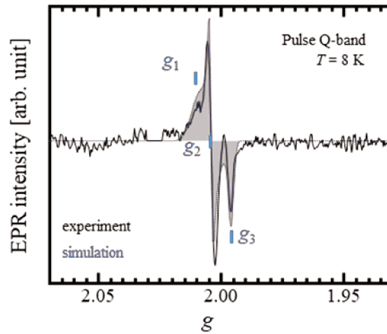
Fig. 5.4-2 Filed sweep spectrum of Sample I. A light blue dot line indicates a fitting spectra of the Defect 2, assuming the principle values of g -tensor were set g_1 = 2.009 , g_2 = 2.005 , g_3 = 1.998 as initial values.
