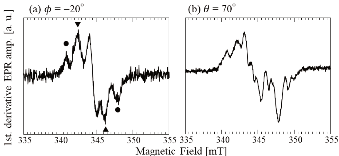
Fig. 5.3-5. EPR spectra of Si-rich single crystal at (a) \phi = -20 deg and (b) \theta = 70 deg. The substructures marked circles and triangles in (a) are separated by 3.49 (●) and 1.89 (▲) mT, respectively. Much more complicated spectrum was observed in (b).
