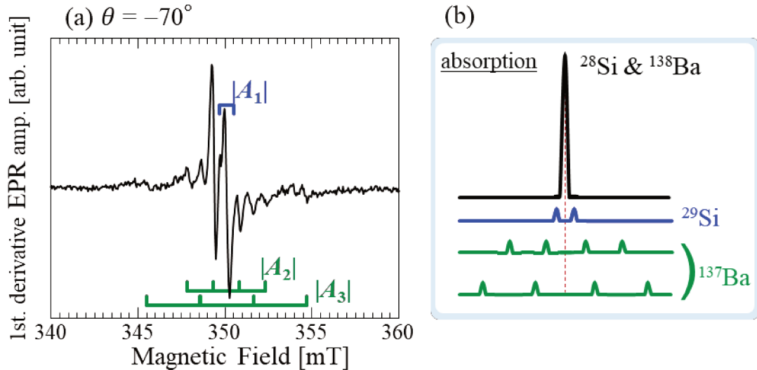
Fig. 5.3-8. (a) EPR spectra of Ba-rich single crystal at \theta = -70^\circ . Each line is explained by three different hyperfine couplings as depicted in (b) schematically. The central line contains no hyperfine coupling following natural abundance of Si and Ba isotopes.
