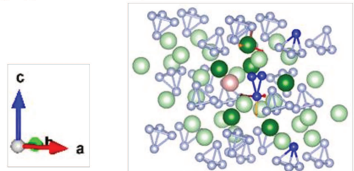
(f) Ba Si ( q = +3, S = 1/2 )
