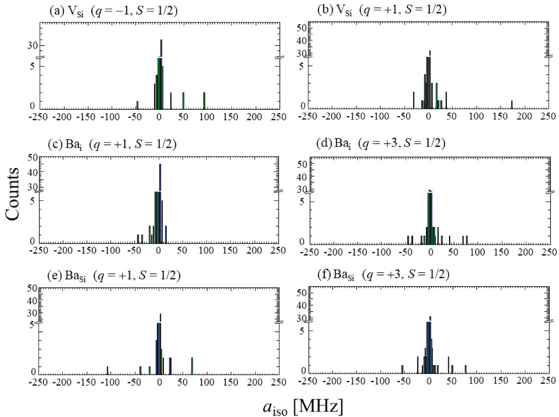
Fig. 5.5-4 Isotropic part of hyperfine tensor for the defects under Ba-rich condition. Blue and green bars correspond to 29 Si and 135 Ba ( 137 Ba) atoms, respectively.
