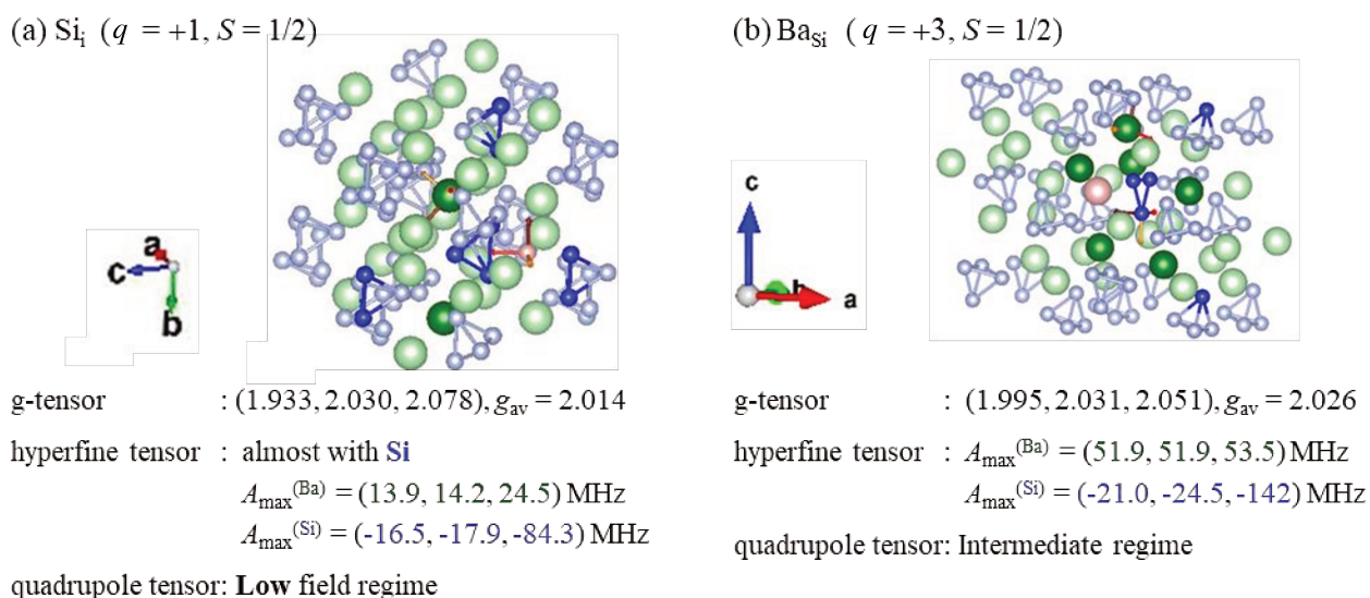
Fig. 5.6-1 Defect models of (a) interstitial Si ( q = +1 ) and (b) Ba antisite substituted for Si ( q = +3 )
