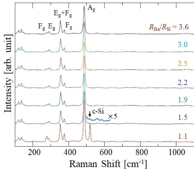
Fig. 4.1-4. Raman spectra of BaSi 2 epitaxial films. The peaks originated from Si 4 cluster were observed in the range of 250-500 cm -1 . The samples with R_{Ba}/R_{Si} = 1.5 and 1.1 are containing c-Si precipitation (Si TO phonon appears at 520.2 cm -1 ).
