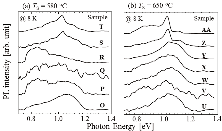
Fig. 6.3-2 PL spectra of BaSi 2 films grown at (a) T_S = 580^\circ\text{C} and (b) T_S = 650^\circ\text{C}
