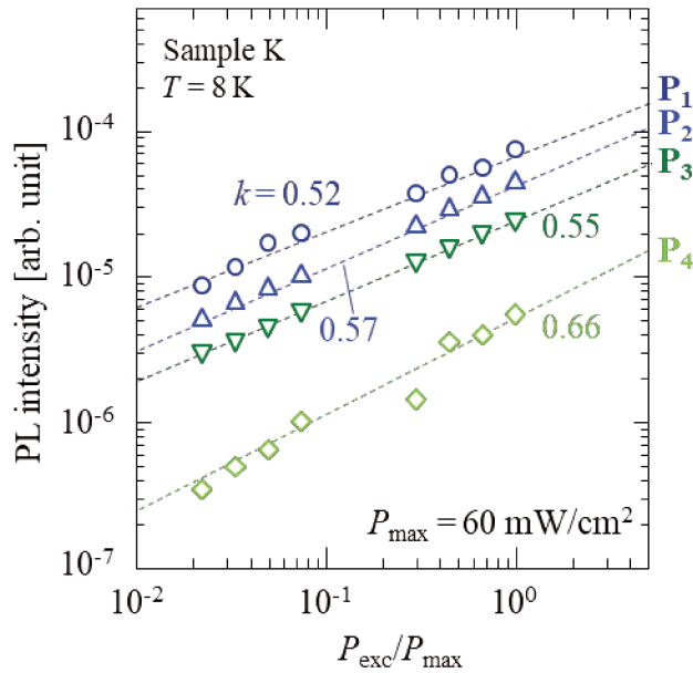
Fig. 6.2-4 Excitation intensity dependence of PL intensity at 8 K for sample K. All transitions follows I_{\text{PL}} \propto P_{\text{exc}}^k ( k < 1 ) as drawn by broken lines.
