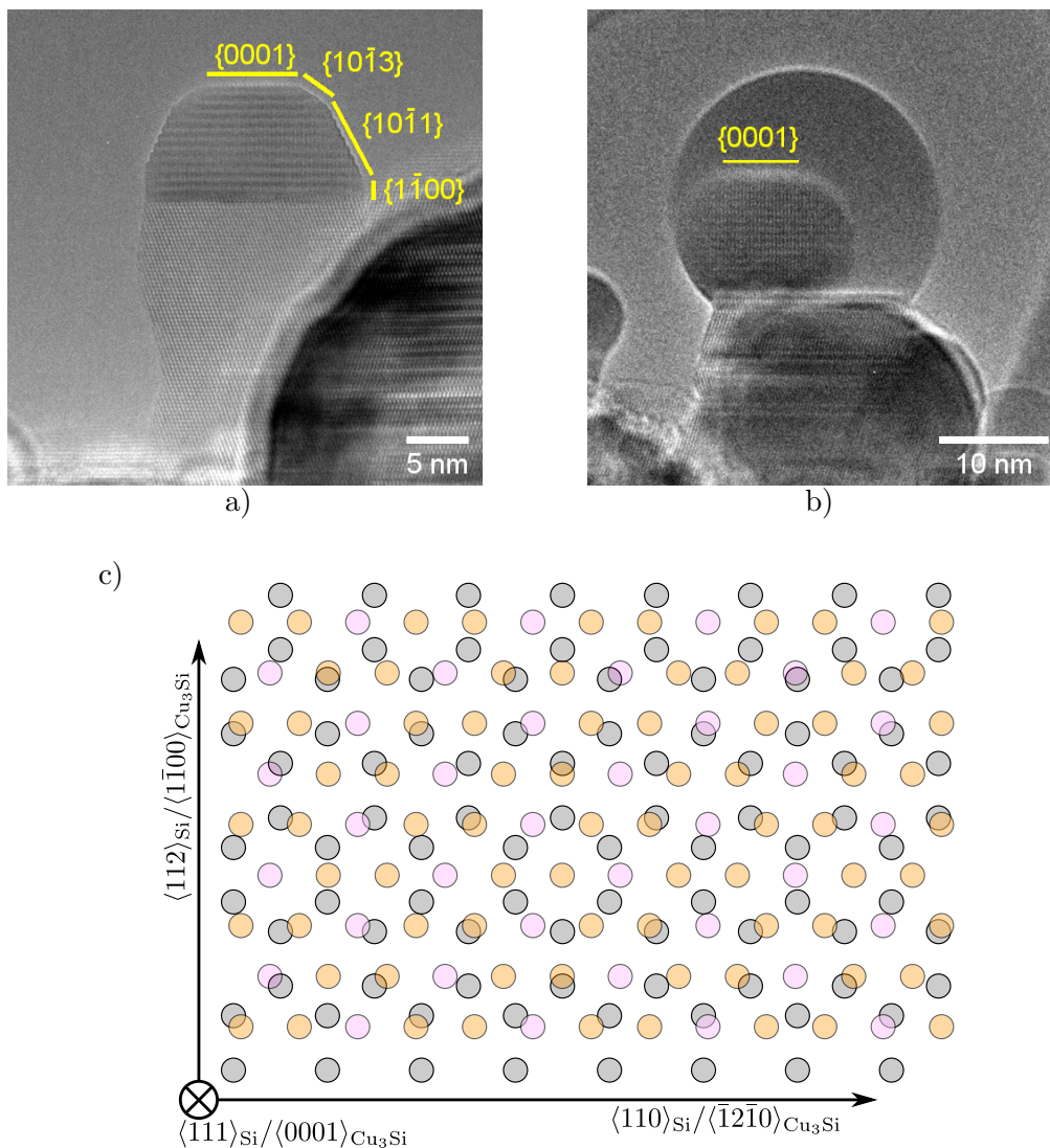
FIGURE 5.18: Orientation of the \text{Cu}_3\text{Si} catalyst in the \langle 111 \rangle_{\text{Si}} || \langle 0001 \rangle_{\text{Cu}_3\text{Si}} epitaxial relationship. a) Side-view TEM image of the catalyst-nanowire interface in a majority-Cu catalyst in this orientation. b) Side-view TEM image of a majority-Sn SiNW where the \text{Cu}_3\text{Si} core is in this orientation. c) Top-view schematic of the interface depicting how the first two layers in a Si and \text{Cu}_3\text{Si} crystal interface stack together with the \langle 111 \rangle_{\text{Si}} || \langle 0001 \rangle_{\text{Cu}_3\text{Si}} epitaxial relationship. Colors are described in Figure 5.17b.
