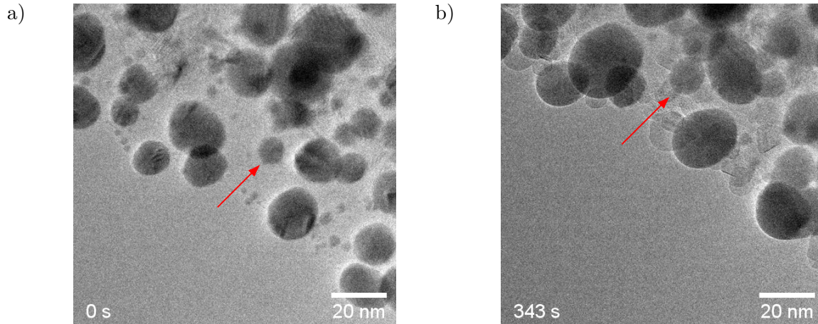
FIGURE 3.2: TEM micrograph of a random assembly of AuGe particles taken at a) the initial stage when the Ge beam is switched on and b) 343 s later at a temperature of 400 °C with the Ge MBE source heated at 1200 °C. The red arrow on both images shows the same particle at different times. Its position is different across both pictures because of image drift.
