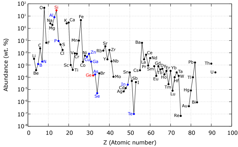
FIGURE 1.1: Abundance of various elements of the periodic table in Earth's crust in weight percentage. Si and Ge are indicated in red. Other elements that are relevant for the semiconductors industry are marked in blue. Data from [12].
