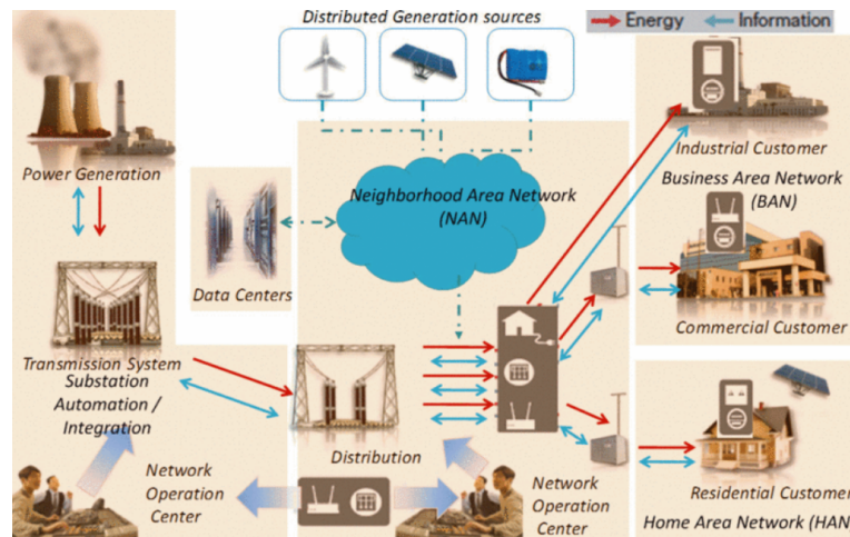
Figure 1.3 – The communication infrastructure for smart grid application [160].
