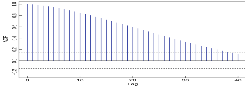
(b) ACF diagram of the time series with an upward trend
