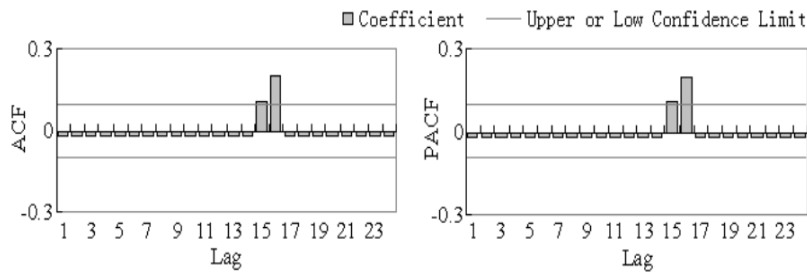
(b) ACF and PACF diagram of the improper sampling period selection
