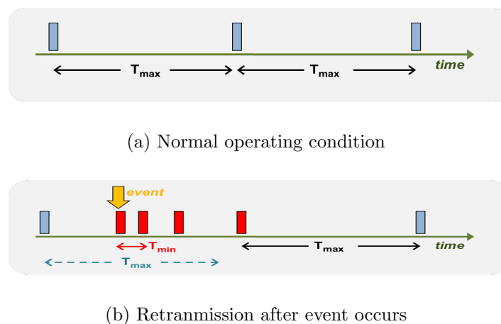
Figure 3.5 – Retransmission mechanism in GOOSE [128].
