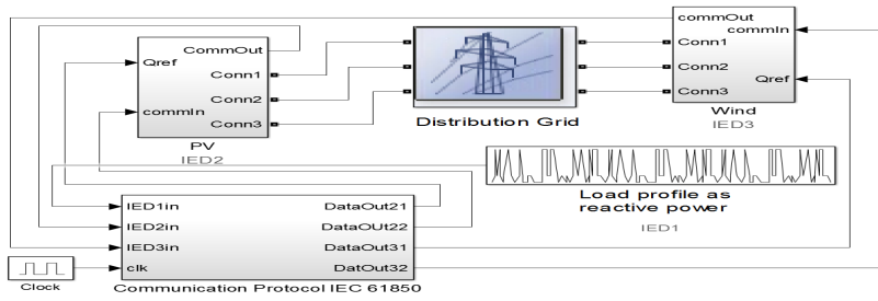
(a) Simulation block diagram of the communication architecture [137]
