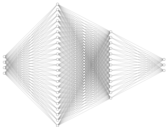
Figure 5.1: A_{NN} architecture with d = 3 assets
