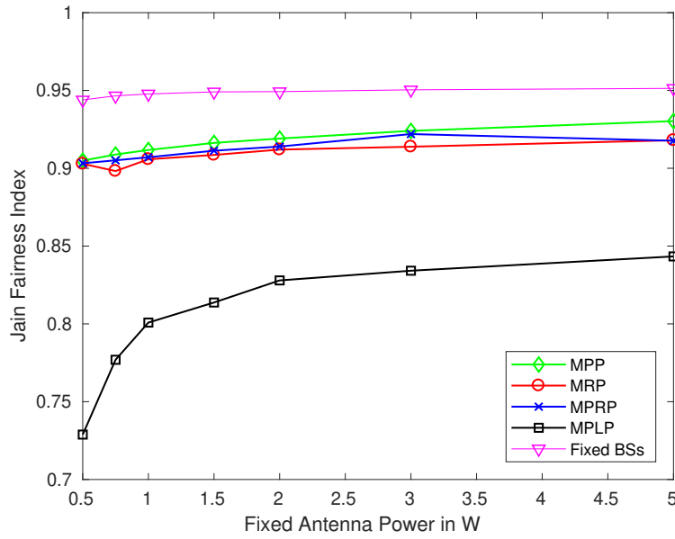
Figure 5.6 – Fairness comparison of the positioning techniques as a function of the fixed antenna power.
