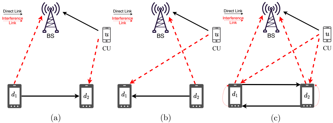
Figure 1.11 – D2D transmission underlaying a cellular system (a) HD transmission, first half time slot, d_1 transmits to d_2 . (b) HD transmission, second half time slot, d_2 transmits to d_1 . (c) FD transmission, d_1 and d_2 transmit to each other in the same time slot.
