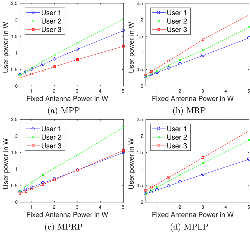
Figure 5.8 – User power allocation according to the selected UPT.
