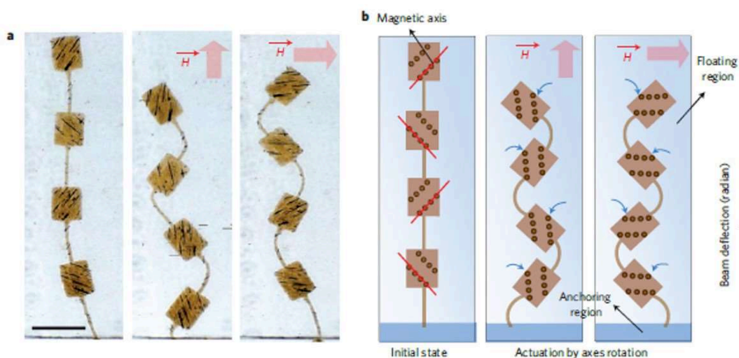
Figure 2.15: a) A microactuator undergoing several bending motions by changing the direction of the magnetic field (scale bar is 100 \mu\text{m} ). B) Scheme of the actuator describing the easy magnetic axis of each part and the possible actuation mechanisms. [175]
