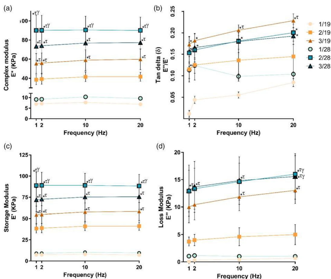
FIGURE 3 Mechanical properties of dense hydrogel discs (2 × 9.1 mm) of different compositions (hydrogel concentration is expressed as de ratio DGL/PEG in mM) measured at room temperature under PBS immersion by dynamical mechanical analysis in compression at a 10% strain and 60 μm of amplitude. A, complex modulus, B, tan delta, C, storage modulus, and D, loss modulus. ( n = 7 , Two-way ANOVA, p < 0.05 , *compared with 1/19, τ compared with 1/28, and γ compared with 2/19)
