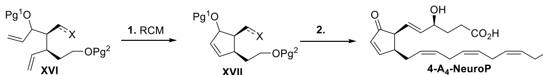
Scheme 23. Envisaged approach to A- and J-NeuroPs.
