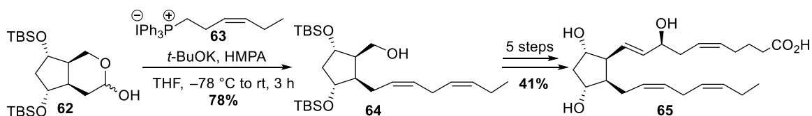
Scheme 14. Total synthesis of 7- F_{4r} -NeuroP 65 by Kim et al.
