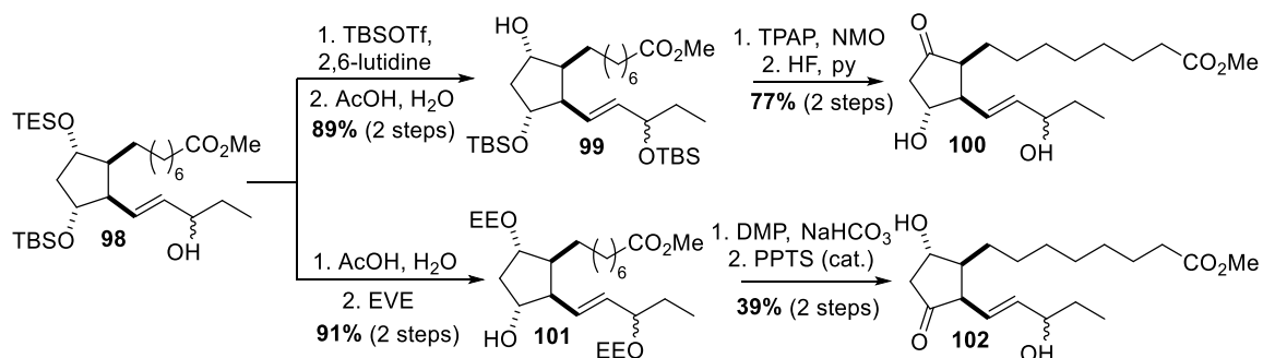
Scheme 22. Completion of synthesis of 16-E 11 -PhytoP and 16-D 11 -PhytoP methyl esters 100 and 102 by Smrček et al.
