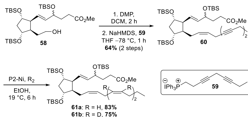
Scheme 13. Approach to 4( RS )-4-F 4t -NeuroP and its deuterated analogue by Oger et al.
