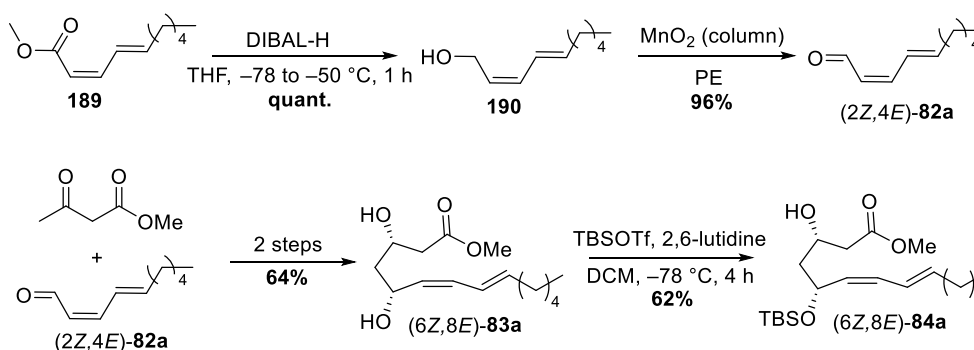
Scheme 81. Synthesis of cyclization precursor (6 Z ,8 E )- 84a .
