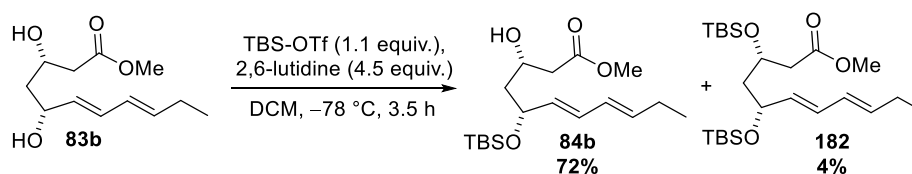
Scheme 75. Synthesis of silyl ether 84b .
