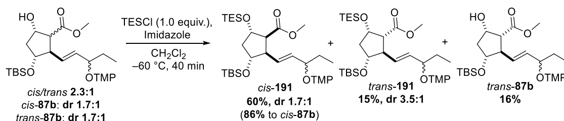
Scheme 82. Diastereoselective silylation of 87b .
