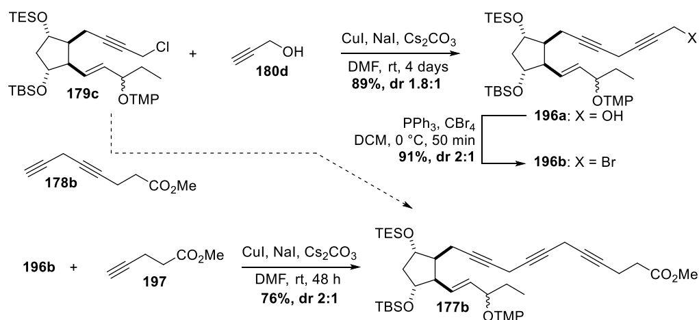
Scheme 88. Synthesis of triyne 177b .
