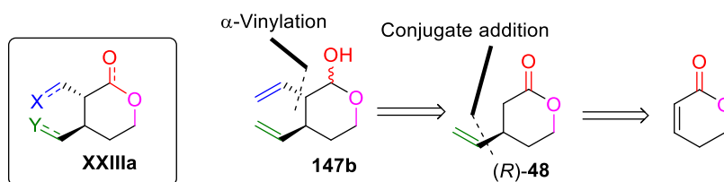
Scheme 53. Retrosynthetic analysis of 147b .
