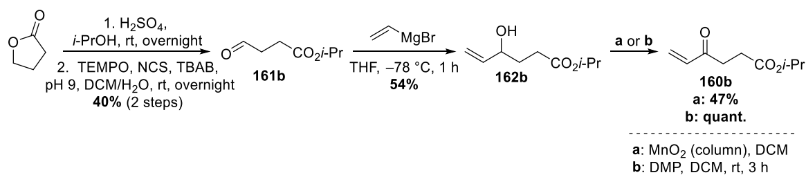
Scheme 65. Synthesis of enone 160b .
