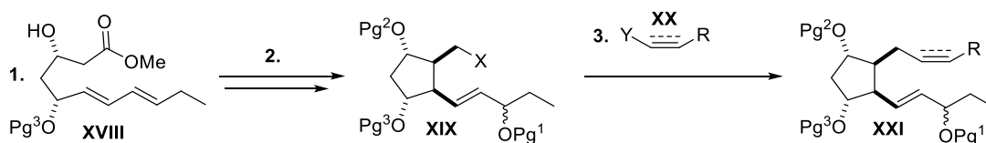
Scheme 24. Envisaged approach to isoprostanoids with 3-hydroxypentenyl ω-chain and a skipped polyene α-chain.
