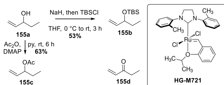
Scheme 59. Structures and preparation of model reactants 155 and structure of catalyst HG-M721 .
