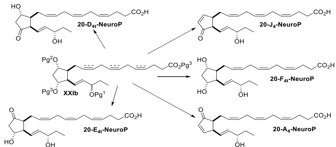
Scheme 26. Envisaged syntheses of 20-NeuroPs.
