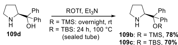
Scheme 31. Synthesis of Hayashi pyrrolidine catalysts 109b and 109c .
