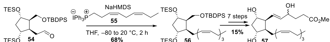
Scheme 12. Synthesis of 4( RS )-4-F 4t -NeuroP-OMe 57 by Durand et al.
