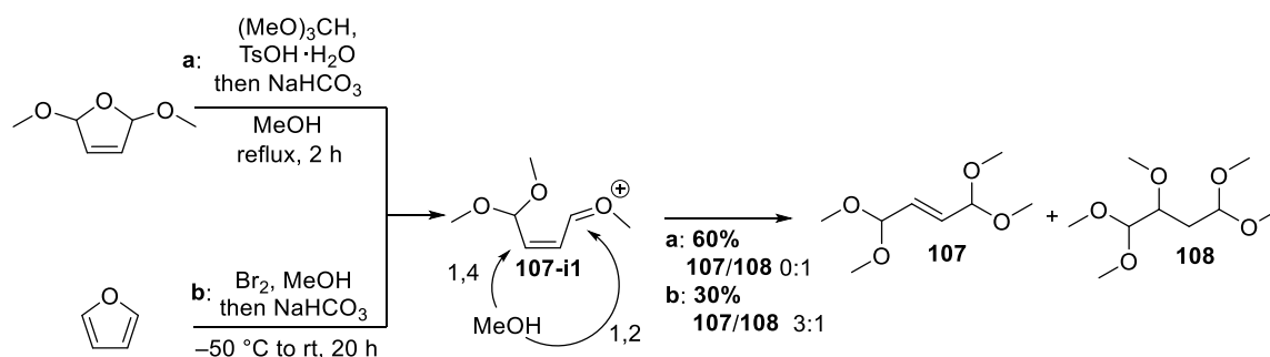
Scheme 29. Synthesis of diprotected enal 107 .
