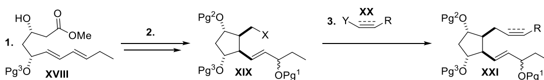
Scheme 24. Envisaged approach to isoprostanoids with 3-hydroxypentenyl \omega -chain and a skipped polyene \alpha -chain.
