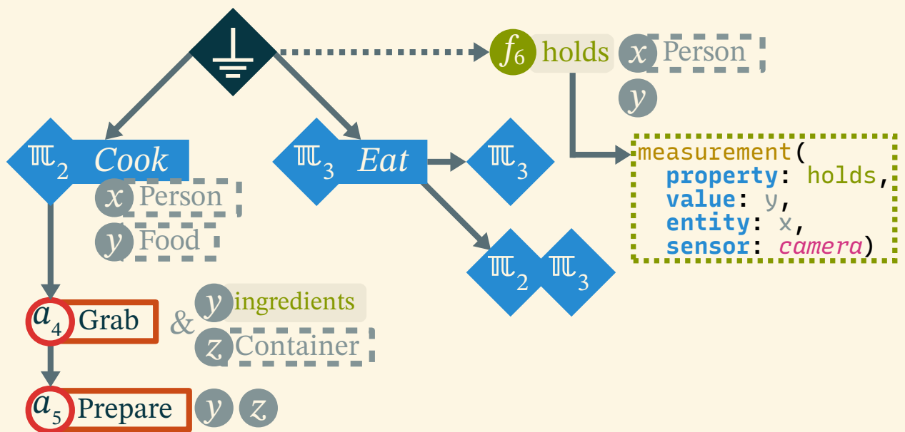
Figure 7.2: The valued grammar used for intent recognition
