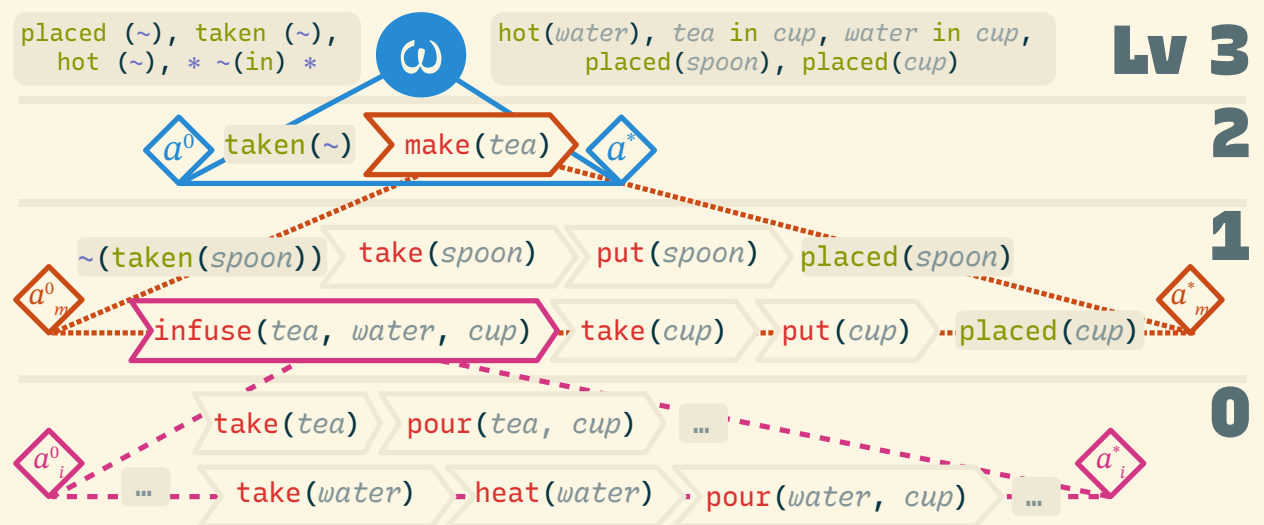
Figure 6.12: Illustration of how the cyclical approach is applied on the example domain. Atomic actions that are copied from a cycle to the next are omitted.
