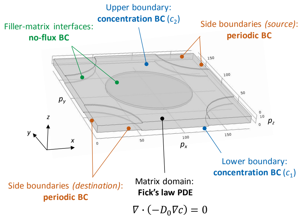
Figure A.2.2 - Tridimensional representation of the unit cell showing the boundary conditions
