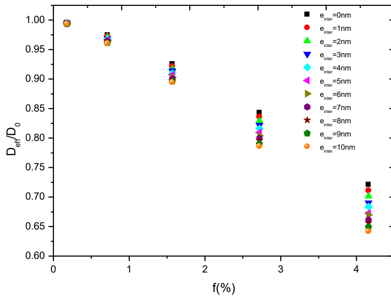
Figure A.3.15 Relative effective diffusivity variation versus filler volume fraction for several values of interplatelet spacing
