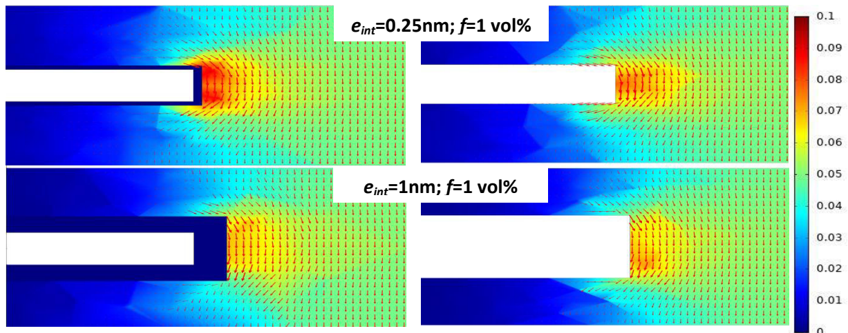
Figure A.4.8 Diffusive flux magnitude field ( \text{mol}\cdot\text{m}^{-2}\cdot\text{s}^{-1} ) and diffusive flux vector field in the vicinity of an impermeable filler surrounded by a low diffusivity interphase ( D_{int}/D_0=10^{-4} ) (left) and in the vicinity of the equivalent fully impermeable filler (right). Arrow length is proportional to the flux magnitude.
