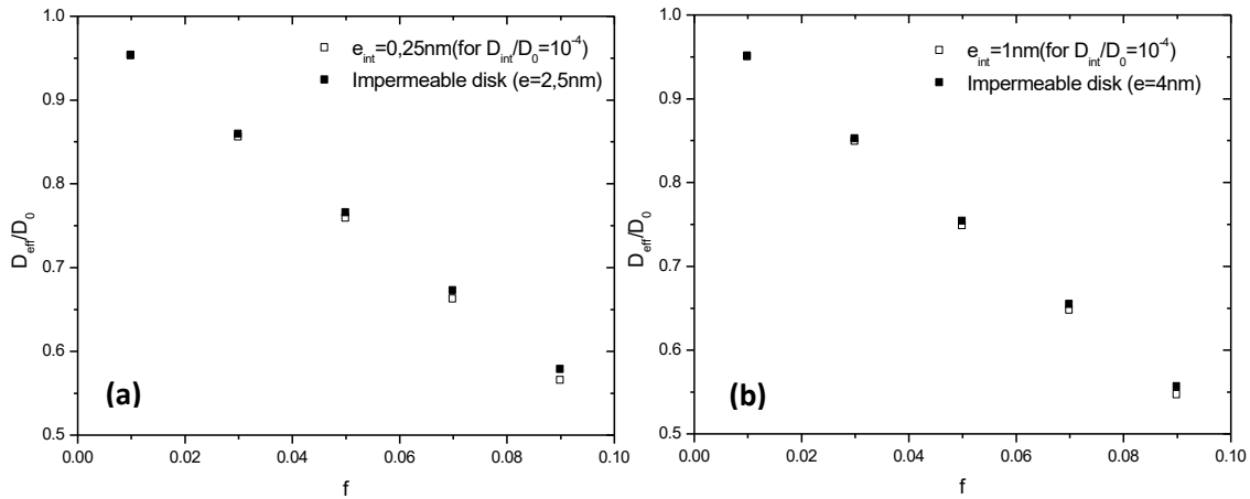
Figure A.4.7 Comparison between the overall diffusivity for systems presenting low diffusivity interphase and fully impermeable interphase (a) e_{int} = 0.25 nm; (b) e_{int} = 1 nm
