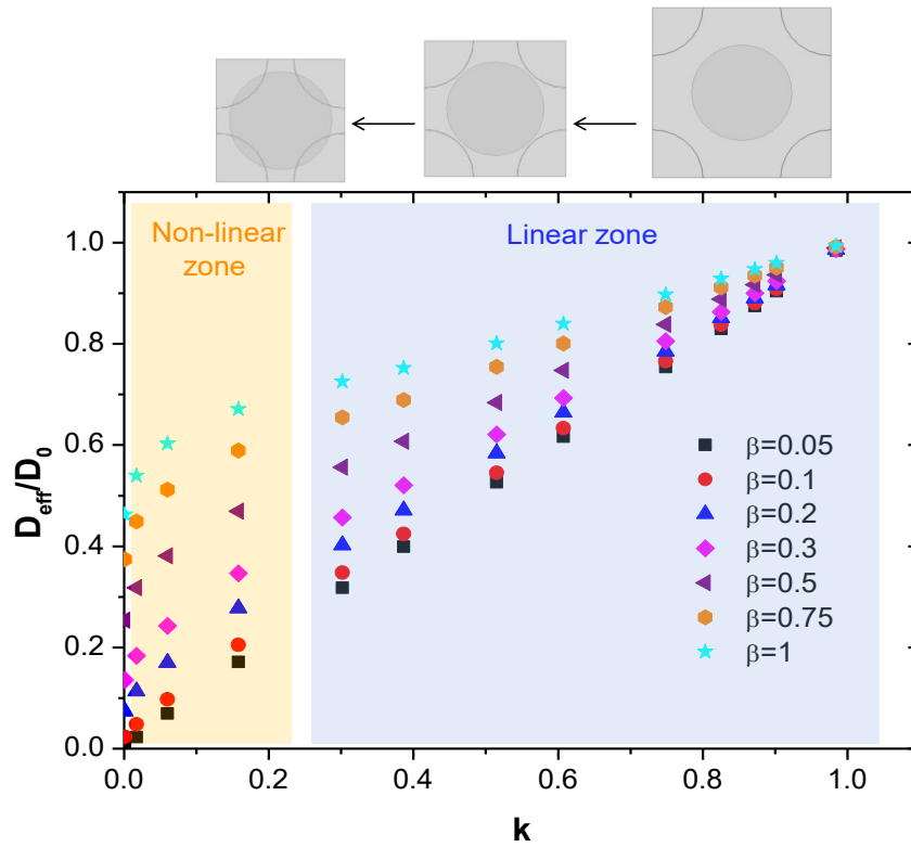
Figure A.2.8 - Relative effective diffusivity versus the projected area ratio k for several values of parameter \beta (centered position of the middle-layer disk)
